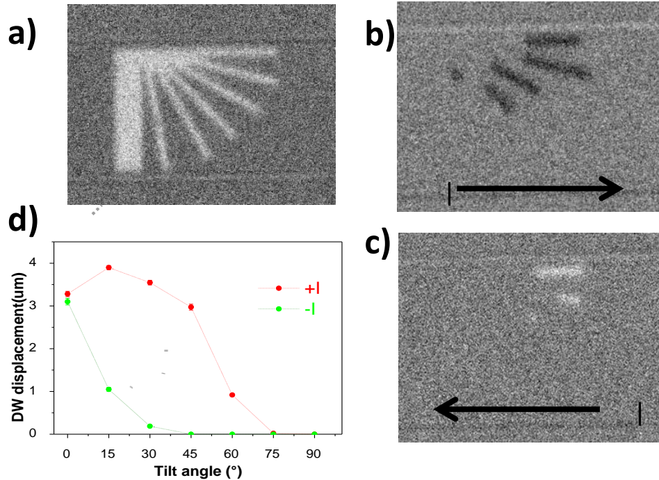
Figure IV.3. MOKE microscopy images of the Pt/Co/ \text{AlO}_x wires in the non-collinear geometry. a) The down magnetic saturated state. b) The differential images of the up/down DW displacement under positive current injection. c) The down/ up DW motion under negative current injection. d) DW displacement with respect to the tilt angle of the wires. The displacements under the a positive (resp. negative) current are shown in red (resp. green). The current density is 1.75 \times 10^{12} \text{ Am}^{-2} and a series of 10 pulses of 2.62ns were applied.
