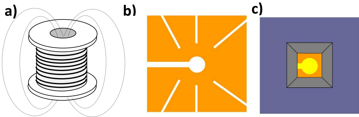
Figure II.6. Schematics of the out-of-plane magnetic coil used for the experiments. a) The normal macroscopic solenoid coil with copper windings. b) The front side of the micro-coil fabricated from copper. The white part shows the insulating part. During the imaging, the face of the sample is glued to this surface. c) The back side of the micro-coil. This side generally faces the objective of the microscope and the imaging is done through the hole at the center [Bonfim 2001]
