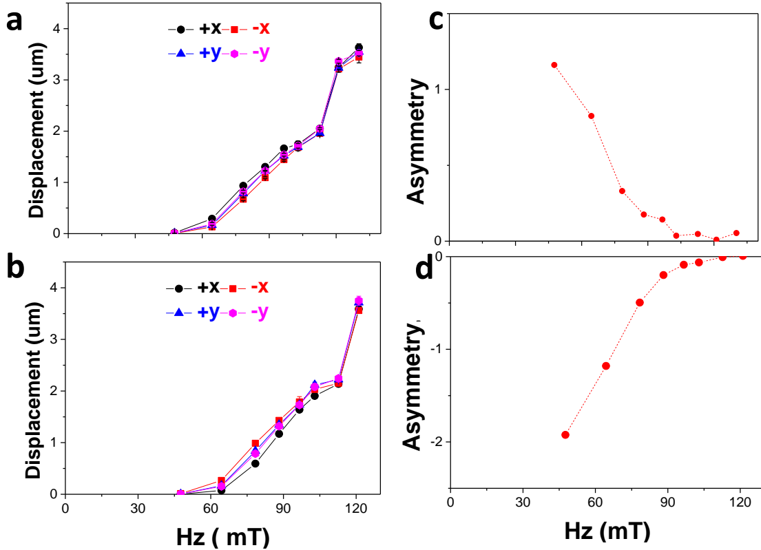
Figure III.21. The DW displacement vs. H_z for Pt/Co/Pt measured from the differential images in figure III.20. a) for H_x = -80\text{mT} b) for H_x = +80\text{mT} . Here the DW displacements along the axis of H_{ip} ( \pm X axis) are different for low H_z values. They became equal at around H_z = 110\text{mT} where the asymmetry disappears. c, d) The asymmetry vs. H_z plots for H_x = -80\text{mT} and for H_x = +80\text{mT} respectively.
