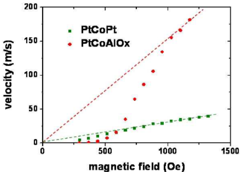
Figure III.22. The DW velocity vs. magnetic field graph measured by I.M. Miron [Miron 2009]. For the same field values, the velocity of the Pt/Co/AlO x (shown in red) is much larger than that of Pt/Co/Pt (shown in green)
