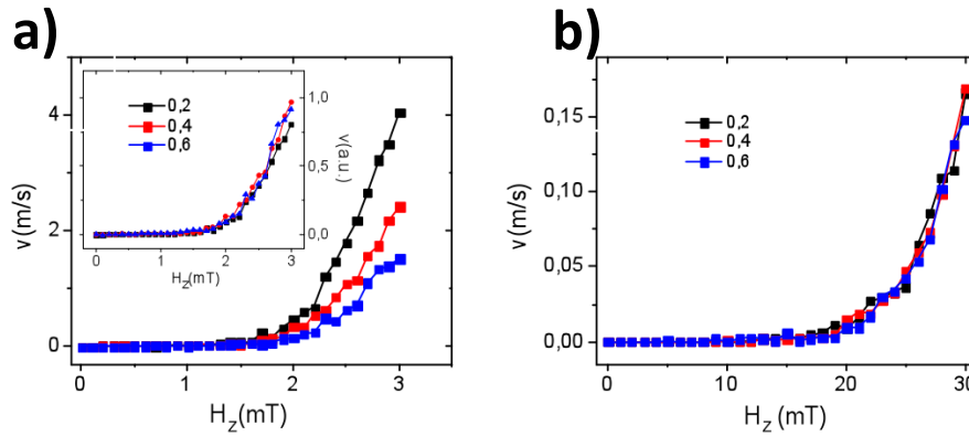
Figure III.14. DW velocity in the 1D model for 3 different damping values. Each velocity point is obtained after averaging 30 displacements produced by 500ns long pulses a ). DW velocity when the width of the pinning potential is 10 times larger than the size of the DW (5nm). The inset shows the velocity curves normalized by the inverse of the damping value. b ). The velocity calculated for a potential half the width of the DW (5nm). In this case, the DW velocity is independent of the damping value.
