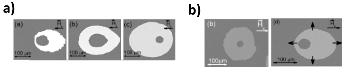
Fig III.5. a) The MOKE images of asymmetric bubble expansion studied by A. Hrabec et al [Hrabec 2014] measured for three different Pt/Co/Ir( t )/Pt samples ( t = 0, 2.3 Å and 4.6 Å from left to right). The asymmetry of the bubble expansion reverses its direction as the t is increased. This is due to the reversal of the sign of the DMI. b) The comparison of the bubble expansion for the epitaxial and sputtered samples. For the epitaxial samples, no asymmetry in the DW motion was observed. This indicates that there is no SIA exist in the epitaxial sample.
