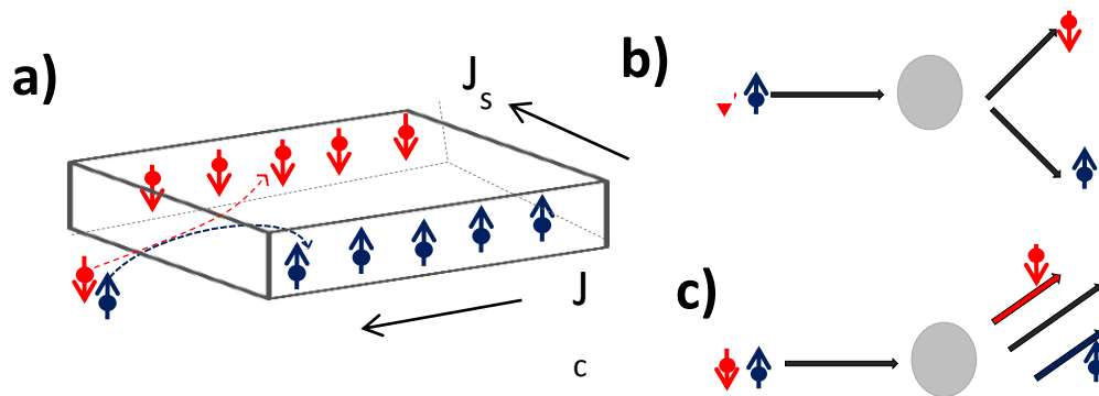
Figure I.18. The schematic diagram of a) the formation of transverse spin accumulation in heavy metal b,c) The two mechanism that causes the spin hall effect: b, the skew scattering where the two spins are scattered due to the spin orbit interaction with an impurity. c, the side jump mechanism due to the spin dependent wave function modification.
