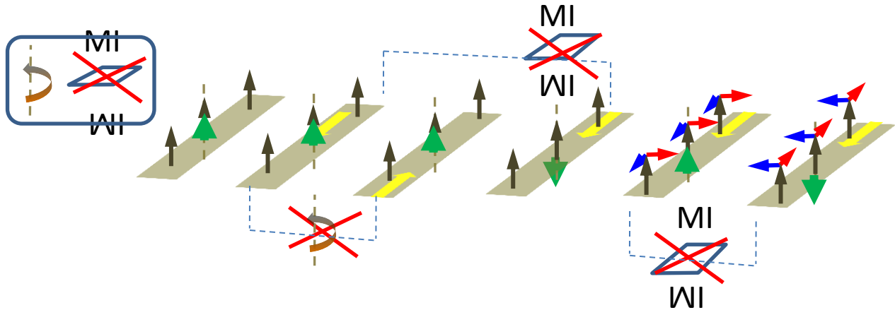
Figure 1.12: In the presence of an additional vertical electric field represented by the green arrow, the mirror symmetry is broken. Then, the existence of an effective field acting on the magnetization does not imply the existence of its opposite. There is no more cancellation and the SOT are allowed.
