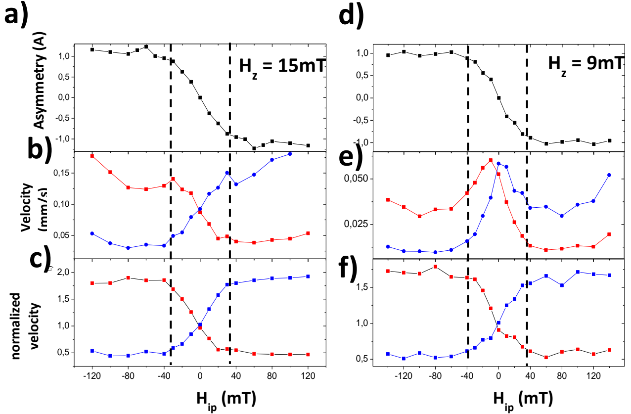
Fig III.8. The experimental graph for a,d) the asymmetry v/s H_{ip} b,e) the velocity v/s H_{ip} c,f) the normalized velocity v/s H_{ip} for the two samples \text{Pt}_{(30\text{\AA})}/\text{Co}_{(6\text{\AA})}/\text{Pt}_{(15.6\text{\AA})} and \text{Pt}_{(30\text{\AA})}/\text{Co}_{(6\text{\AA})}/\text{Pt}_{(18.6\text{\AA})} respectively. The asymmetry and the normalized velocities for both DWs saturate at H_{ip} = \pm 40\text{mT} associated with a slope change of the velocity graphs at the same field.
