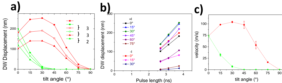
Figure IV.4. a) DW displacement with respect to the tilt angle for three different pulse lengths 3.75ns, 3.14ns and 2.76ns. The DW displacements corresponding to a single pulse are plotted. They are calculated by dividing the total displacement in each wire by the number of pulses injected for each case. b) DW displacement versus the pulse length for each wire. Note that for a negative current, there is no plot for wires with angles > 30^\circ because the displacements were zero. c) DW velocity versus the tilt angle. The DW velocity value in this graph is obtained from the slope of the corresponding linear plot in figure b.
