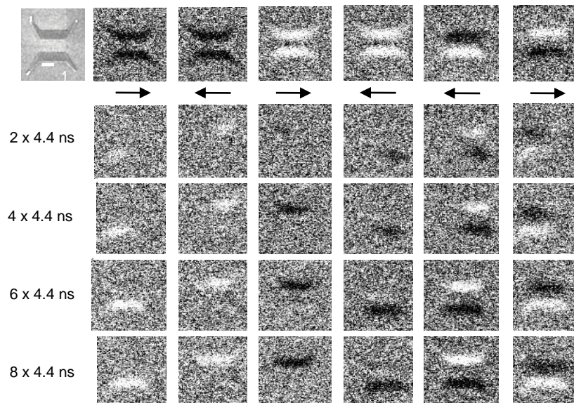
Figure IV.16: Step by step imaging of the DW motion during the switching for a u-shape device and an inverted u-shape device. The pulses used were 4.4ns long. The first row contains the images of the initial magnetic states of the switches. The black arrows show the direction of the current. The further consecutive images in each column correspond to the step-by-step DW motion after applying a series of 2 current pulses at each step. These images confirm that the switching occurs according to the nucleation and DW propagation mechanism explained in the text
