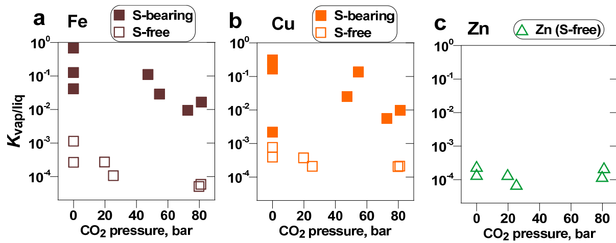
Fig. 6. Bulk vapor-liquid partition coefficients for Fe, Cu and Zn as a function of CO 2 pressure in the S-free (#m31) and S-bearing (#m28) systems.
