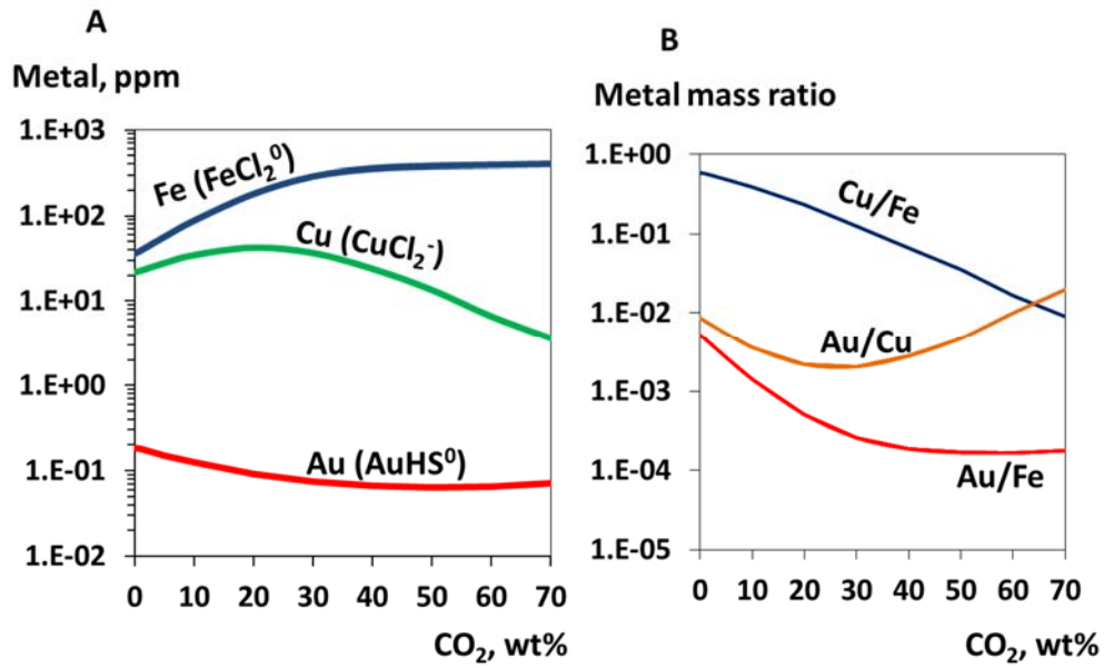
Fig. 15. Solubility of pyrite, chalcopyrite and native gold in supercritical fluids at 450°C and 2 kbar with 7 wt% (NaCl + KCl), as a function of \text{CO}_2 content (A), and the corresponding metal ratios in the fluid (B), predicted using the model parameterized in this study. The dominant metal species are indicated in (A). Redox and acidity conditions are buffered by the QMK and PPM assemblages ( \text{H}_2\text{S} \sim 0.1 wt%). These conditions simulate relatively oxidizing and S-poor (<0.1 wt% S) fluids, typical of orogenic Au deposits, and, possibly, some deep porphyry and volcanic massive sulfide Cu-Fe-Au deposits.
