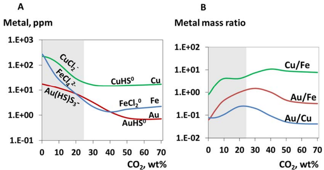
Fig. 17. Solubility of pyrite, chalcopyrite and native gold in supercritical fluids at 500°C and 1 kbar with 10 wt% NaCl and 1 wt% S ( H_2S:SO_2 = 1 ) as a function of CO_2 content (A), and the corresponding metal ratios in the fluid (B), predicted using the model of this study. The dominant metal species are indicated in (A). Redox and acidity conditions are controlled by the QMK or QAK buffers (muscovite transforms into andalusite at 40 wt% CO_2 ). These conditions simulate the oxidizing S-rich fluids of magmatic origin from typical porphyry Cu-Au deposits. The gray region denotes the maximal range of CO_2 contents reported in such deposits.
