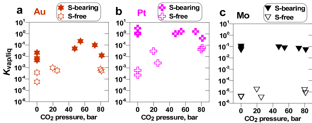
Fig. 7. Bulk vapor-liquid partition coefficients for Au, Pt and Mo as a function of CO 2 pressure in the S-free (#m31) and S-bearing (#m28) systems.
