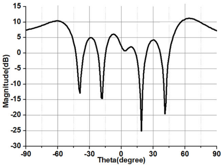
Fig.4.17 Directivity pattern in E-plane ( E_\theta ) for 6-groove array with w=15\text{mm}
