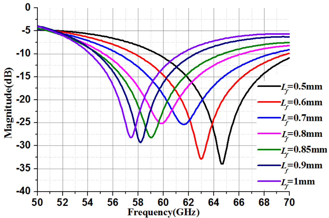
Fig.2.39 S11 when l_s=1\text{mm} , w_s=0.1\text{mm} and L_f varies in [0.6, 1] mm
