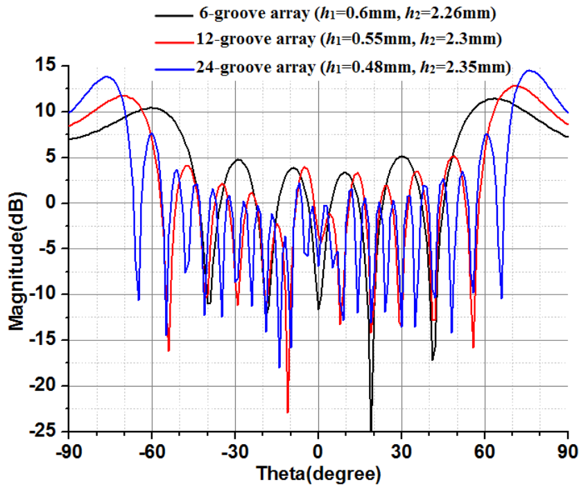
Fig.4.36 Comparison of main beam pointing for array in different sizes
