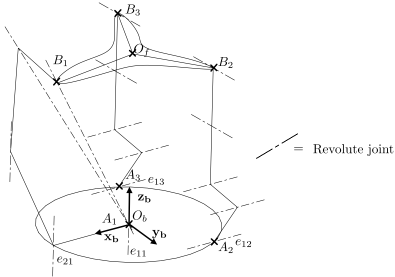
Figure 2.13 – 2T2R–Candidate II.
