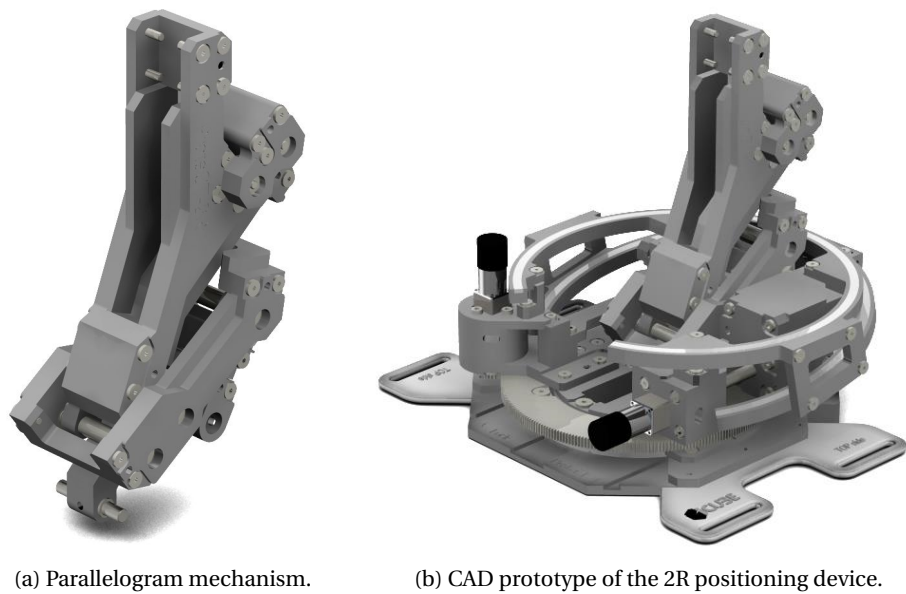
Figure 3.18 – CAD design of the positioning device [Wach, 2014].
