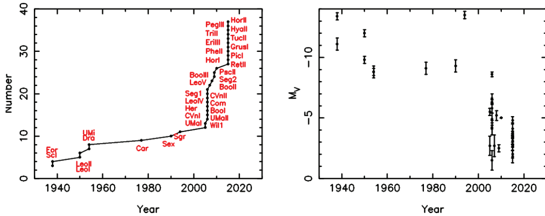
Figure 1.2 - Left: The number of satellites as a function of discovery data. The number of galaxies, shoots up with the age of large CCD surveys, going from 11, pre-2005 to \sim 37 as of this year. Right: M_V of satellites as a function of the year they were found. The explosion of satellites in the SDSS and DES, coincides with many new fainter satellites.
