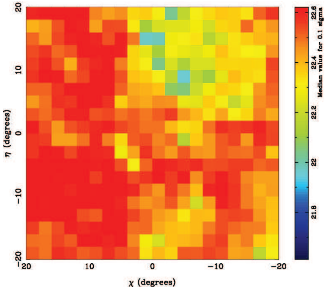
Figure 7.5 - The usual 1600 \text{ degree}^2 patch, centred on (l, b) = (30^\circ, 70^\circ) , colour-coded by the median i-band magnitude at which the photometric uncertainty is \sigma_i = 0.1 . This value is inserted into equation 7.2, which is in turn inserted into equation 7.1, giving the completeness function, used to accept and reject “observed” stars.
