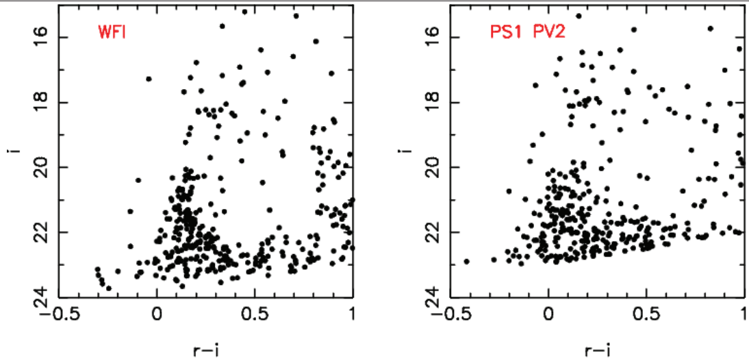
Figure 3.1 - Left : WFI data of Segue 1, with a very clear Main-Sequence, a turn off and a sparsely populated red giant brach. The photometric improvement is quite considerable, showing extra depth as well as a tighter Main Sequence Right : PV2 photometry from PS1 for Segue 1. Though it is clear that there is something here with a whole bunch of blue stars, the scatter in photometry does not allow for a clear Main Sequence to be determined.
