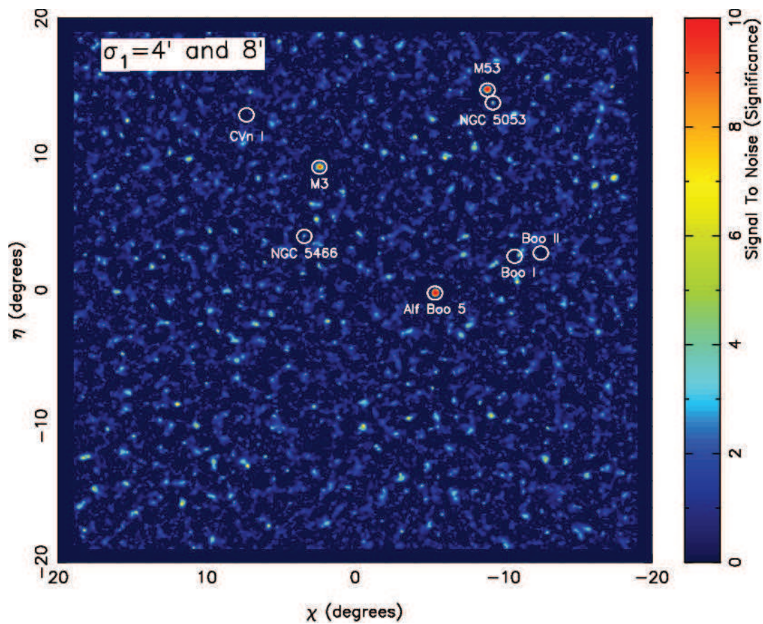
Figure 2.19 - Stacked (4' and 8') S/N map for galaxies' sample. Many of the MW satellites show up as insignificant detections in the galaxies' map confirming them to be real stellar systems. Some of the MW GCs also show up as significant detections in the galaxies' map. This because they are so bright that the star-galaxy separation breaks down and also starts classifying some of the sources here as galaxies. 'Alf Boo 5' shows up significantly in the galaxies' map and the stellar map in Figure 2.18, confirming that it is a contaminant in the stellar map and should be excluded.
