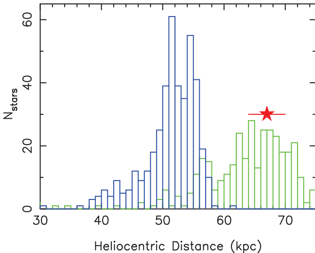
Figure 6. Heliocentric distance histogram of all particles in the Law & Majewski (2010b) model within 1 degree of Sgr II's longitudinal position (no constraint was applied on the latitude). As in Figure 5, blue and green dots represent particles from the leading and trailing arm, respectively. The distance to Sgr II and its uncertainty are represented by the red star and the error bar and show that Sgr II is perfectly compatible with belonging to the trailing arm of the Sgr stream.
