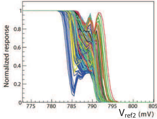
Figure 4.22: The measured “S” curves for the in-pixel discriminator V2 at nominal speed. Due to the coupling between column data line and V_{ref1} , the “S” curves are strongly disturbed.
