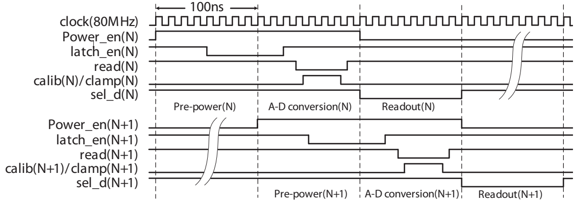
Figure 4.13: Timing diagram.
