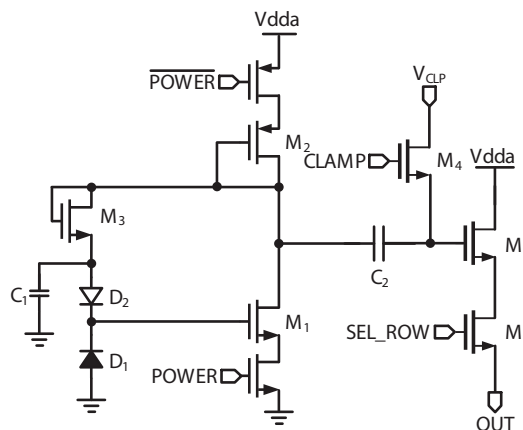
Figure 3.8: The schematic of the pixel P25 in MIMOSA-32Ter.
