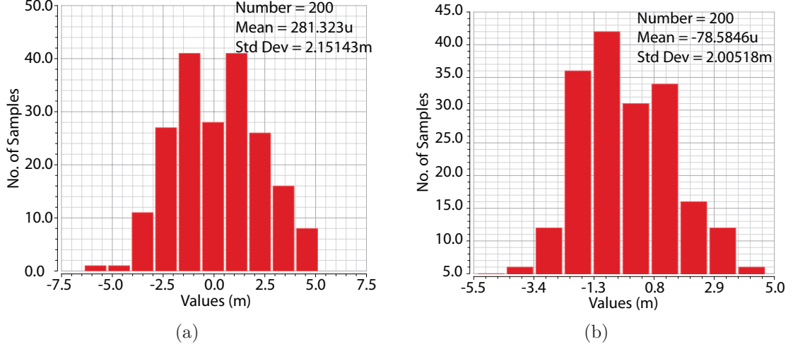
Figure 4.17: Simulated offset distribution of the dynamic latch. (a) the mismatches of all the transistors are considered and (b) only the mismatch from the input pair is considered.
