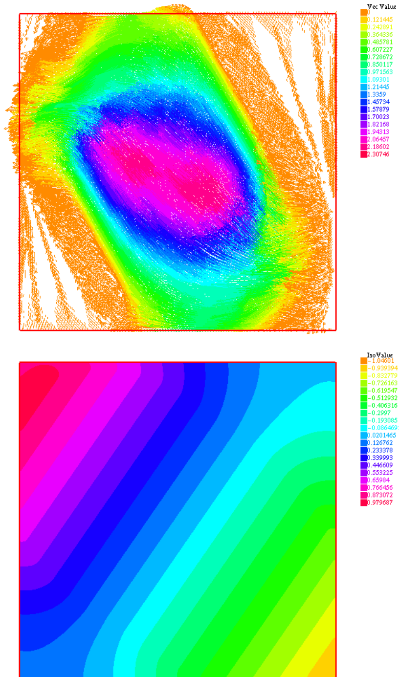
Figure 5.4 – Test case 3 : k = 15 , v_j = \left(\cos\left(\frac{(j-1)\pi}{k}\right), \sin\left(\frac{(j-1)\pi}{k}\right)\right) and \xi_j = \cos\left(\frac{2(j-1)\pi}{k}\right) for j = 1, \dots, k with f = f_1 .
