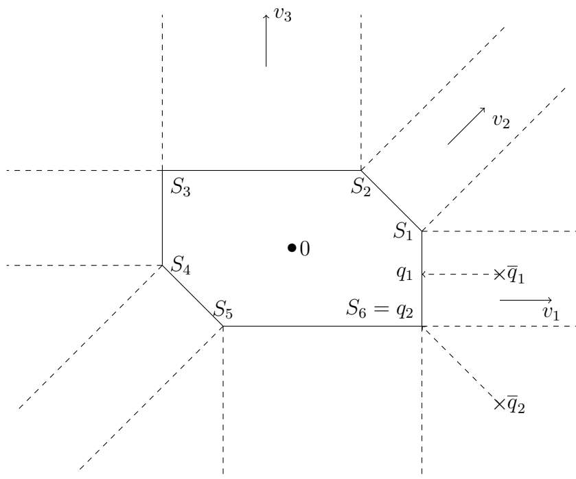
Figure 5.1 – An illustration of projection on a polyhedron.
