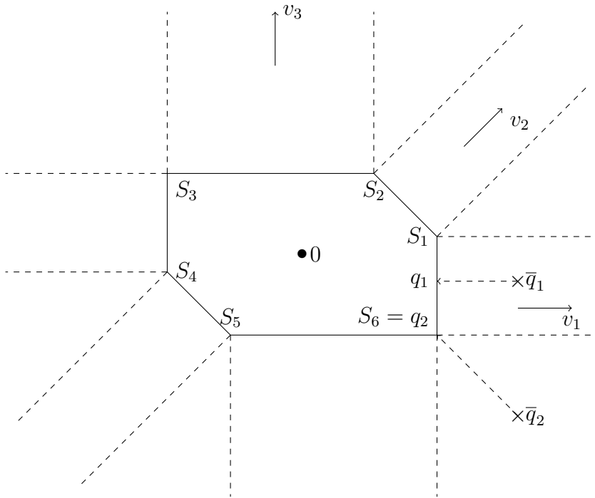
Figure 5.1 – An illustration of projection on a polyhedron.
