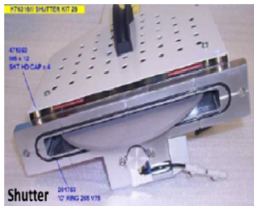
Figure III-5: Image du Shutter
