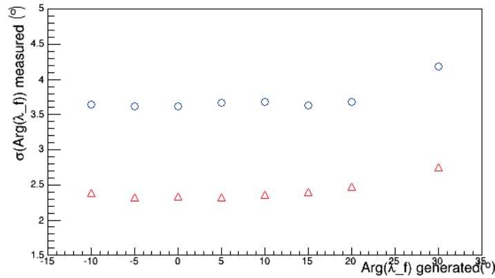
Figure 3.16: Estimated statistical uncertainty on the measured value of \arg(\lambda_f) as a function of the generated value of \arg(\lambda_f) , observed for the expected D^0 \rightarrow K^+K^- decay statistics (red triangles) and for the expected D^0 \rightarrow \pi^+\pi^- decay statistics (blue circles) in Belle II.
