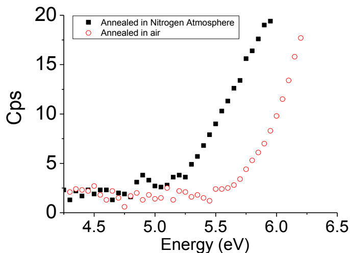
Figure 7.7: Square roots of photoelectron yield vs energy for annealed LPE-G in nitrogen (black dots) and for comparison the spectra reported in Figure S13 for LPE-G annealed in air (void red dots)
