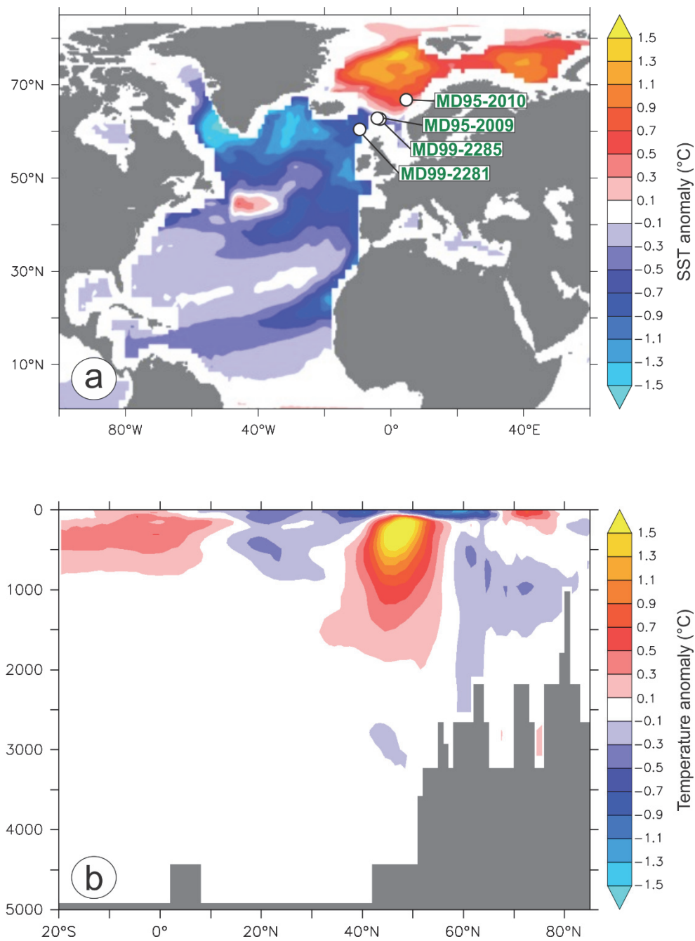
Figure 1: Five-member ensemble mean of temperature differences. a , Map showing the cores location (from north to south: MD95-2010, 66.68°N, 4.57°E, 1,226 m depth; MD95-2009, 62.74°N, -4.00°E, 1,027 m depth; MD99-2285, 62.69°N, -3.57°E, 885 m depth; MD99-2281, 60.34°N, -9.46°E, 1,197m depth) as well as SST differences (°C) between hosing and control experiments averaged over the 4th decade. The study area constitutes a nodal point regarding the modern surface oceanic circulation. It is indeed located at the convergence of (i) the northward warm North Atlantic water inflow and (ii) the southward polar water outflow through the East Greenland current terminal limb, i.e. the East Icelandic Current. Previous paleoclimatic studies 34,35 evidenced that this area was also a key sector during the Last Glacial Maximum when, similarly to the SST pattern shown on the present map, warmer SST were recorded within the Nordic Seas and colder ones within the North Atlantic. This suggests that such a situation might represent a regular feature, at least for glacial periods. b , Latitude-depth section of the temperature differences (in °C, averaged over the whole Atlantic basin) between hosing and control experiments averaged over the 4th decade.
