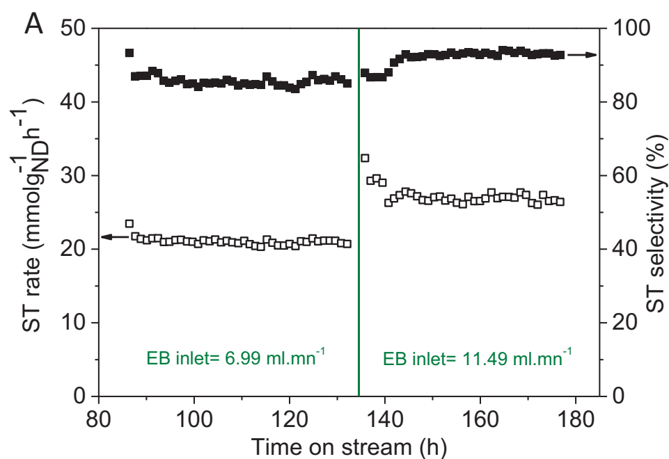
Figure 65. Influence of the ethylbenzene concentration on the DH performance of the ND/CNF-FLG catalyst. Reaction conditions: catalyst weight = 300 mg, 600 °C, EB concentration = 6.99 and 11.49 \text{ml.min}^{-1} EB in helium, total flow rate = 30 \text{mL}\cdot\text{min}^{-1} .
