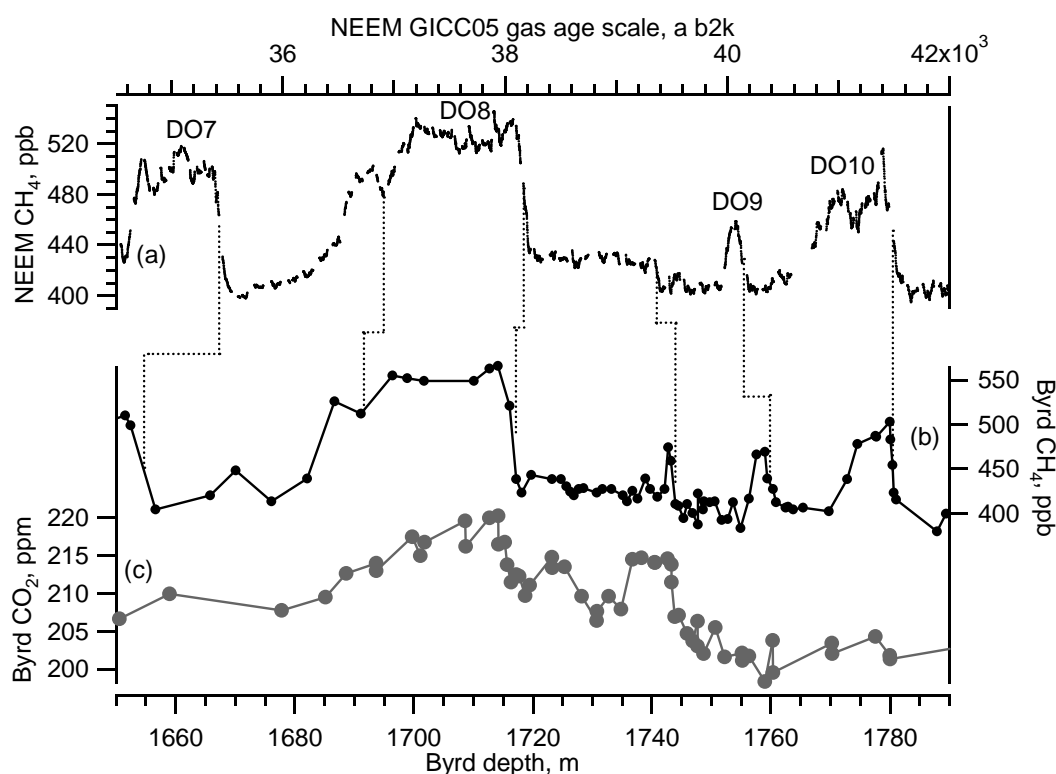
Figure 5.11: Construction of a gas age scale for the Byrd ice core. (a) NEEM methane data (Chappellaz et al., 2013) on the NEEM GICC05 gas age scale (Rasmussen et al., 2013). (b) CH 4 and (c) CO 2 data from the Byrd ice core on a depth scale (Ahn et al., 2012). The dotted black lines indicate the match points used to tie the Byrd record to the NEEM GICC05 gas age scale.
