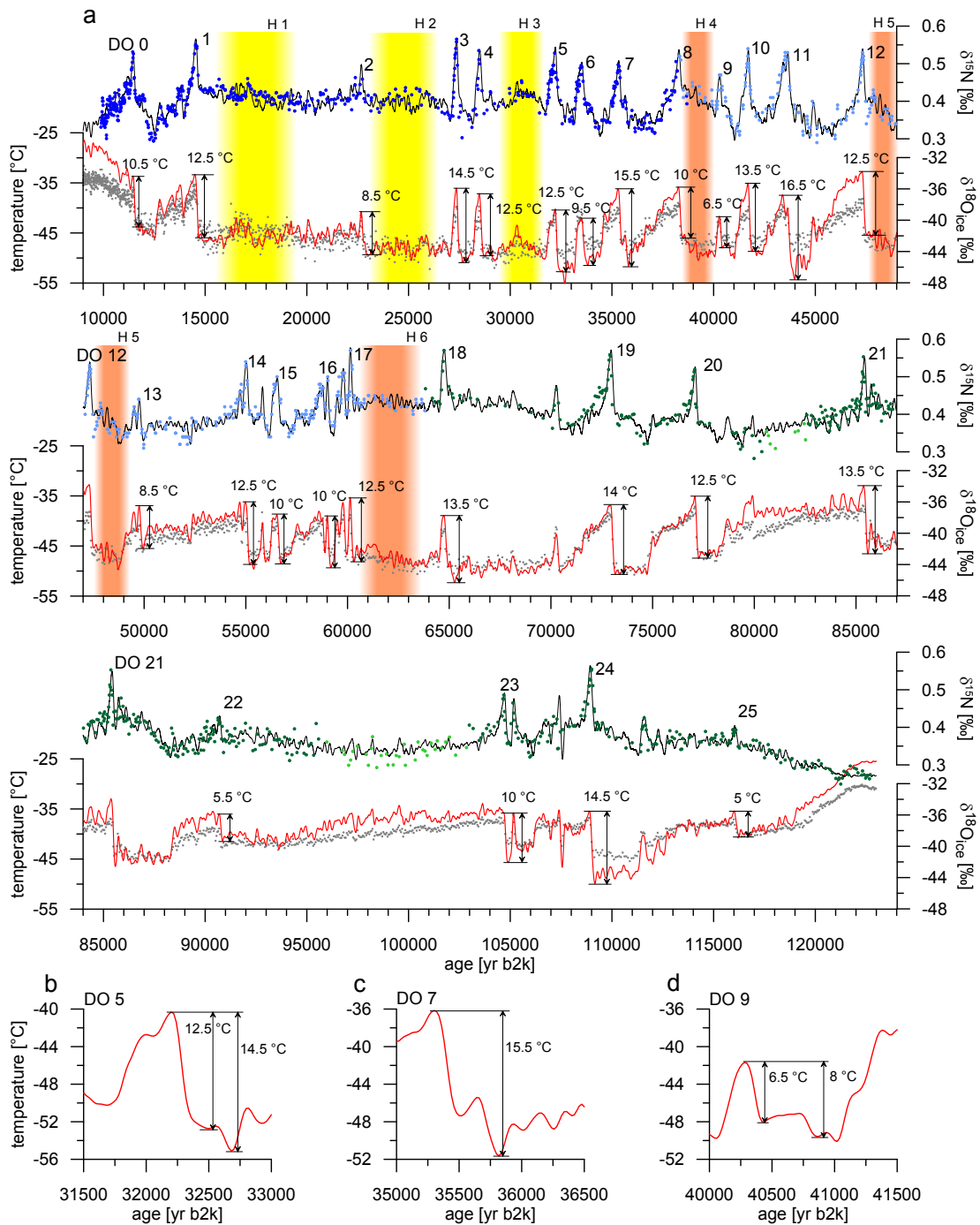
Fig. 3. (a) NGRIP temperature reconstruction from 10 to 120 kyr b2k on the ss09sea06bm time scale. Red line: temperature reconstruction, grey points: \delta^{18}O_{ice} (0.55m mean data, (NGRIP members, 2004)) on ice age scale, dark blue points: new \delta^{15}N measurements, this study, light blue points: measurements from Huber et al. (2006b), dark green points: published \delta^{15}N measurements from LSCE (Landais et al., 2004a, 2005; Capron et al., 2010a,b, 2012), light green points: unpublished \delta^{15}N measurements from LSCE, black line: modelled \delta^{15}N , all \delta^{15}N data is plotted on the gas age scale. Because there is no exact agreement in the literature about the timing and the duration of H events (Hemming, 2004; Sánchez Goñi and Harrison, 2010; Jonkers et al., 2010; Roche et al., 2004), we do not explicitly indicate the H events themselves but the stadials in which they took place by colouring the corresponding time period in yellow (no long term warming observed in the stadial with a H event) and orange (a long term warming is observed). (b) to (d): Focus on the temperature evolution of DO 5, 7 and 9.
