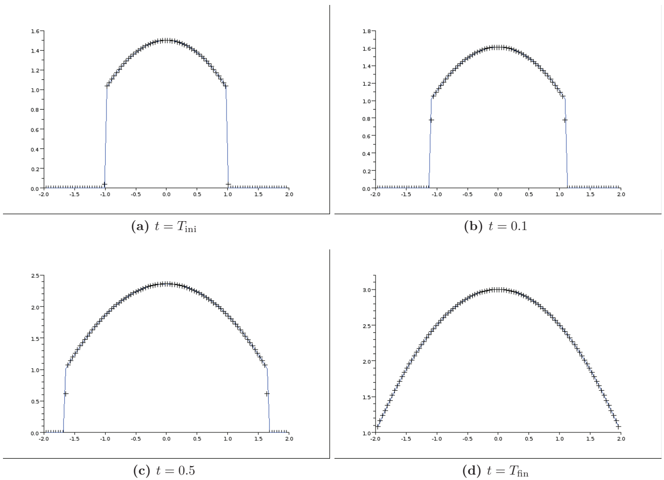
Figure 1.7 – Evolution of the solution \bar{u} in blue and of the discrete solution u in black crux.
