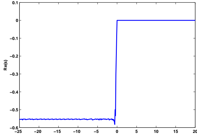
Figure 3.11: The distribution for the real parts of the roots of Eq. (3.21).
