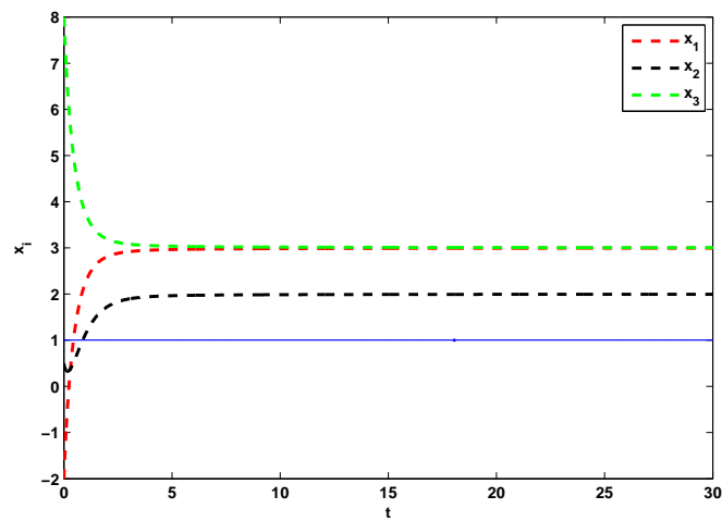
Figure 5.4: The states of agent i with a constant reference state using control law (5.2) in Fig. 5.3.
