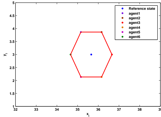
Figure 5.18: The desired formation geometric form for six agents using control law (5.22).
