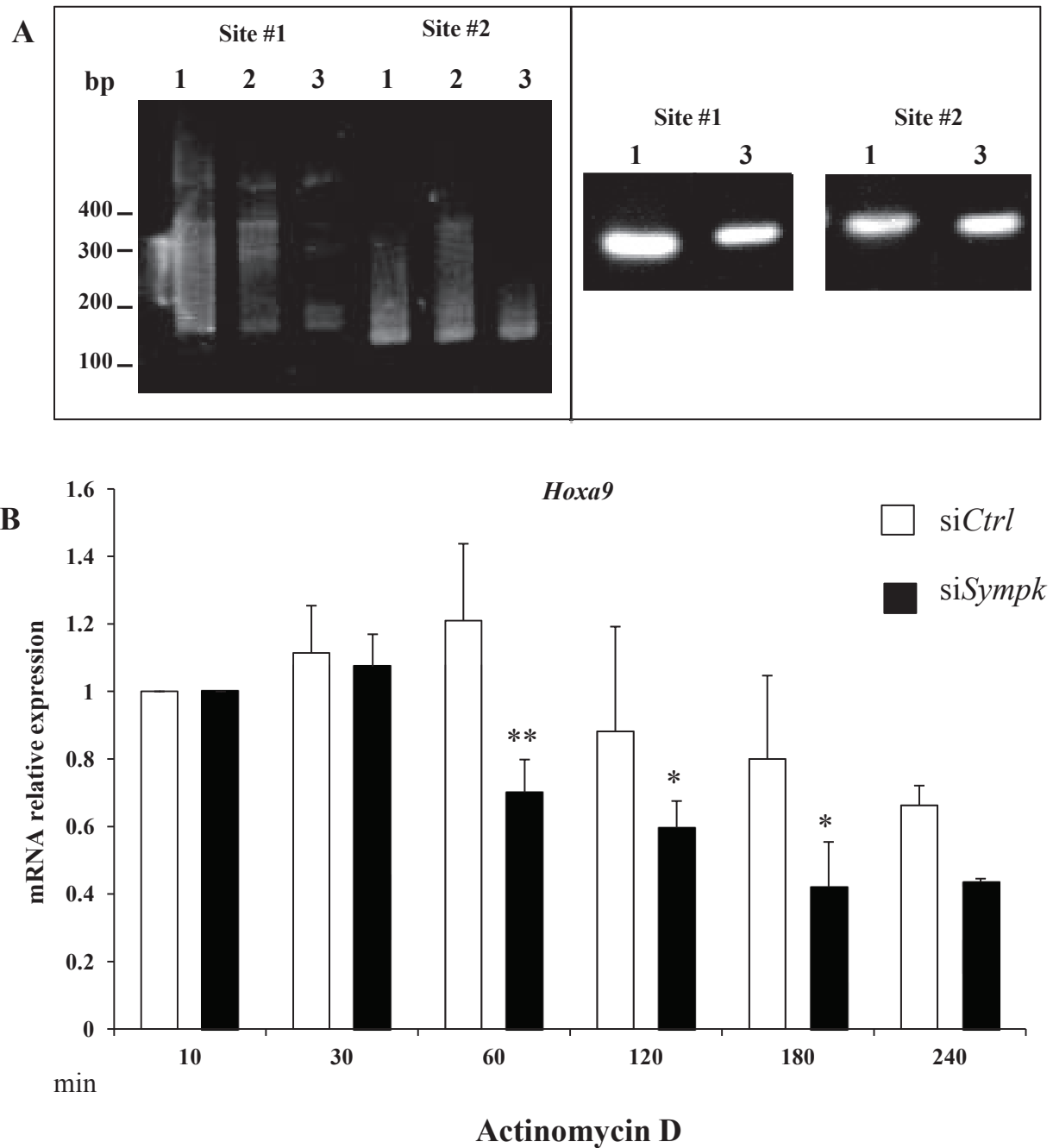
Fig. 5. Symplekin acts on polyadenylation of Hoxa9 mRNA. (A) Impairment in Hoxa9 polyadenylation after Symplekin knockdown. Cells were transfected with siCtrl (1), siMOZ (2) or siSympk (3). The amplified products corresponding to polyadenylated Hoxa9 (left panel) or controls (right panels) were analyzed by PAGE. (B) Cells were transfected with siCtrl or siSympk and treated with actinomycin D, 24 hrs after transfection. Hoxa9 mRNA level was measured by RQ-PCR. Error bars represent standard deviation (n=3).
