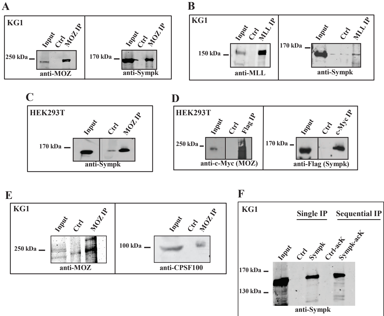
Fig. 1. Sympk is associated with MOZ and MLL. (A) Sympk interacts with MOZ in KG1 cells. IP were performed with anti-MOZ, then immunoprobed with anti-MOZ or anti-Sympk. (B) Sympk interacts with MLL. IP were performed with anti-MLL, then immunoprobed with anti-MLL or anti-Sympk. (C) Sympk interacts with MOZ in HEK293T cells. IP were performed with anti-MOZ, then immunoprobed with anti-Sympk. (D) Flag-Sympk interacts with c-Myc-MOZ. Flag-Sympk or c-Myc-MOZ vectors were transfected into HEK293T cells. IP were performed with anti-Flag or anti-c-Myc, then immunoprobed as indicated. (E) MOZ interacts with CPSF100 in KG1 cells. IP were performed with anti-MOZ, then immunoprobed with anti-MOZ or anti-CPSF100. (F) Sympk is acetylated. A first IP was performed with anti-Sympk, eluted, then a second IP was performed with anti-acetylated lysine (anti-acK) and immunoprobed with anti-Sympk.
