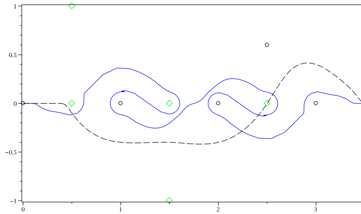
FIGURE 13. The final path \tilde{\Gamma}_1 associated with \tilde{\lambda}_0 , the fixed singular points A and the movable singular ones \tilde{\lambda}_0(1) - B
