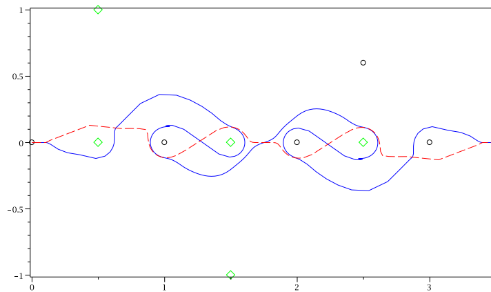
FIGURE 14. On the same picture, the path \Gamma_1 with dashed lines and the path \tilde{\Gamma}_1 . We have also indicated the fixed (circles) singular points A and the movable (diamonds) singular points \lambda_0(1) - B = \tilde{\lambda}_0(1) - B .
