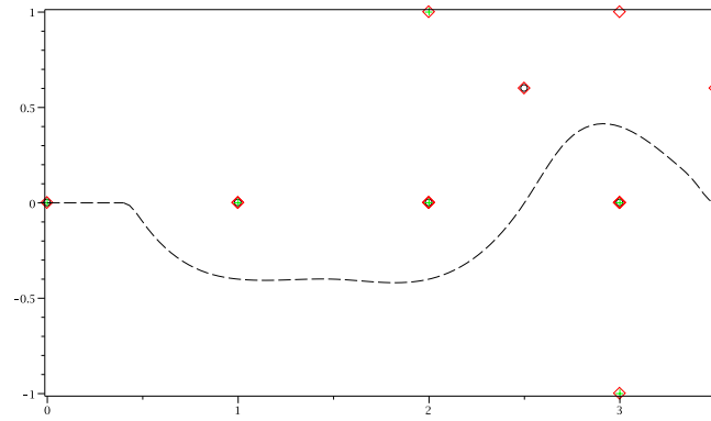
FIGURE 9. The path \tilde{\lambda}_0 drawn with dashed lines and the singular locus A + B
