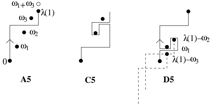
FIGURE 27. An example of a “double” pinching.
