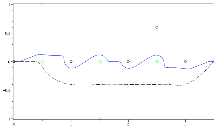
FIGURE 8. The final path \Gamma_1 associated with \lambda_0 and the fixed (circles) and movable (diamonds) singular points.
