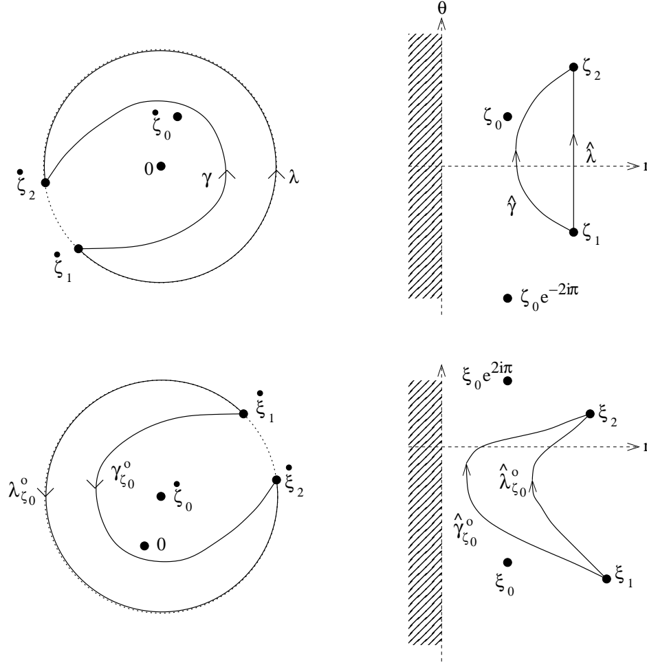
FIGURE 21. On the upper-left picture, the path \gamma is homotopic to the path \lambda in D(0, R)^* \setminus \{\zeta_0\} . On the upper-right picture, their liftings on \mathbb{H} . On the lower-left picture, the path \gamma_{\zeta_0}^\circ = \zeta_0 - \gamma is homotopic to the path \lambda_{\zeta_0}^\circ = \zeta_0 - \lambda in D(0, r + R)^* . On lower-right picture, their liftings on \mathbb{H} where \xi_0 and \xi_0 e^{2i\pi} are above \zeta_0 . No pinching occurs when \zeta_0 \rightarrow 0
