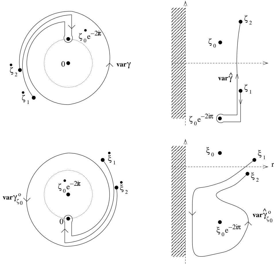
FIGURE 23. Effect of the monodromy on the paths drawn on Fig. 22, up to homotopy : the paths \text{var } \gamma , \text{var } \hat{\gamma} , \text{var } \gamma_{\zeta_0}^o and \text{var } \hat{\gamma}_{\zeta_0}^o .
