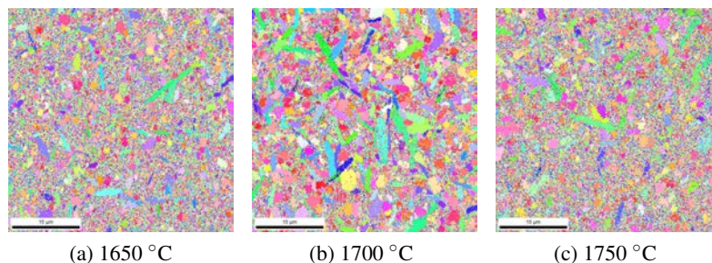
FIGURE 3.5: EBSD micrographs of the materials sintered with addition of 5% of \text{Y}_2\text{O}_3 at 1650 (a), 1700 (b) and (c) 1750 °C
