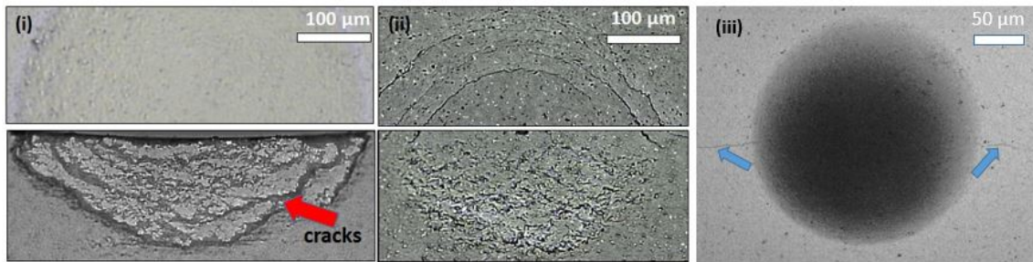
FIGURE 4.6: Optical micrographs of surface and subsurface contact damage in silicon nitride materials with porosity (i) 18% and (ii) 3% under maximum load of 500 N, (iii) specimen with 18% of porosity under 750 N. Indentation tests were made by diamond sphere of radius R_2 = 1 mm
