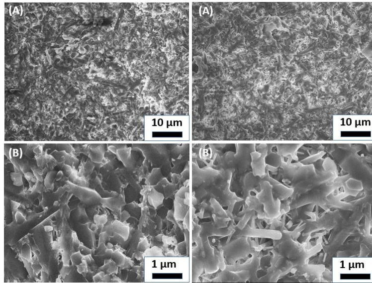
FIGURE 4.3: Fracture surface in materials with 3% (left) and 18% (right) porosity volume content at different magnifications : (A) \times 1000 and (B) \times 5000
