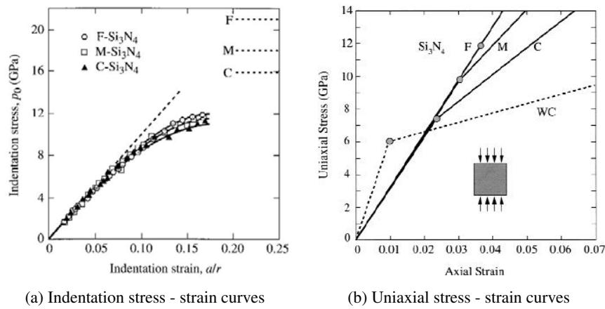
FIGURE 1.22: Indentation and true stress-strain curves for fine (F), medium (M) and coarse (C) silicon nitride [Lee et al., 1997]
