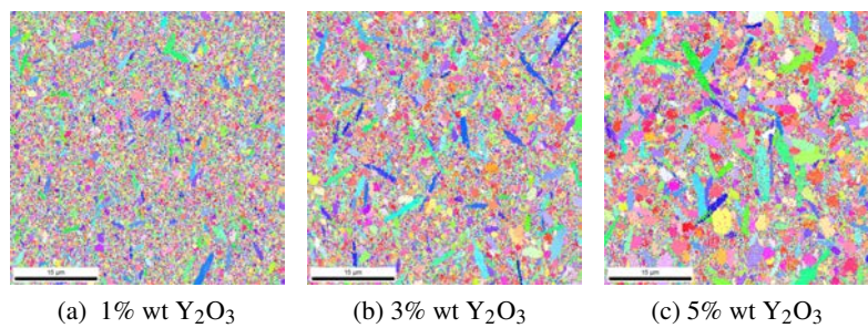
FIGURE 3.4: EBSD micrographs of the materials sintered with addition of (a) 1% wt, (b) 3% wt and (c) 5% wt of \text{Y}_2\text{O}_3 at 1700 °C
