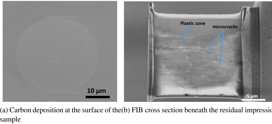
FIGURE 3.15: Subsurface damage in coarse silicon nitride after indentation with a sphere of radius 0.2 mm at peak load P = 45 N
