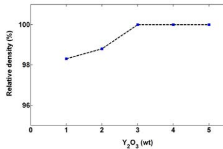
FIGURE 3.3: Evolution of the relative density of \text{Si}_3\text{N}_4 samples sintered at 1700 °C depending on the \text{Y}_2\text{O}_3 content
