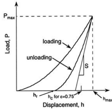
FIGURE 2.8: Indentation technique
