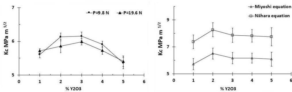
(a) Effect of maximum load for Palmqvist crack system (b) Niihara versus Miyoshi for median crack system
