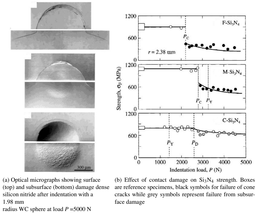
FIGURE 1.13: Contact damage (a) and strength degradation in silicon nitride with different grain sizes (b) [Lawn, 1998]
