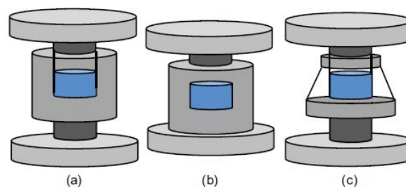
FIGURE 1.8: Different configuration of the SPS system
