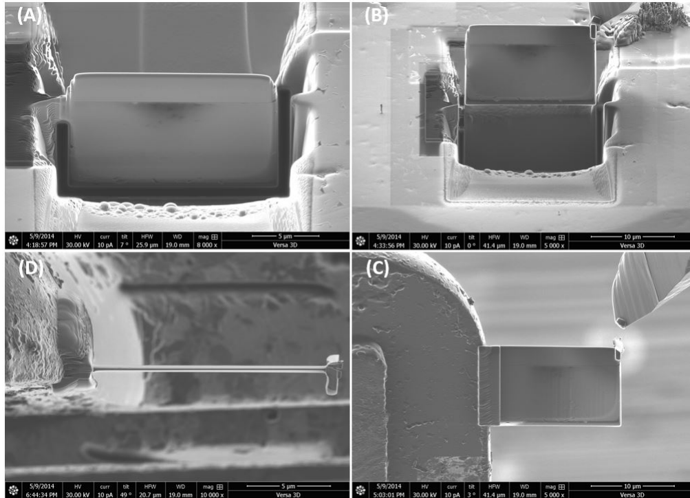
FIGURE 2.6: Transmission Electron Microscopy thin foils preparation from the damaged area (a) edges and bottom cutting (b) lift-out (c) TEM grid (d) rotation and final thinning
