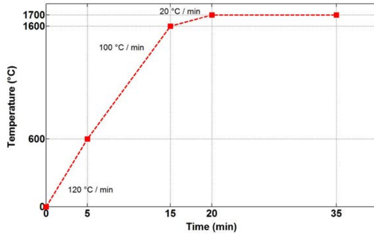
FIGURE 2.1: Sintering temperature cycle
