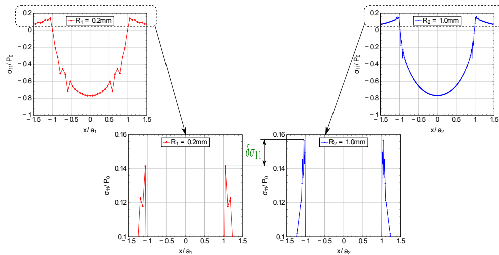
FIGURE 4.16: The obtained profile of the radial stress in the porous material for the two indenter radii
