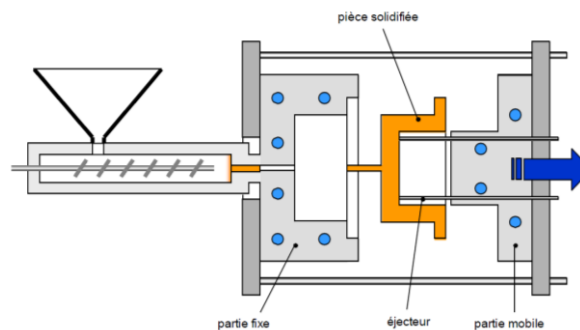
Figure 1.7 : Phase d'éjection [31]
