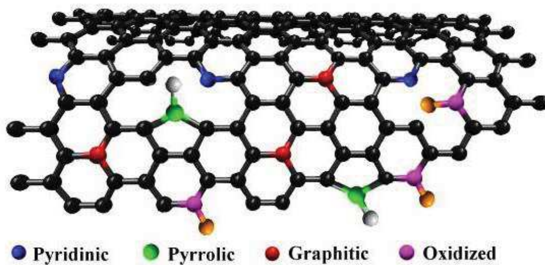
Fig. 1.4. Types of nitrogen species that can be incorporated into graphitic carbon.
