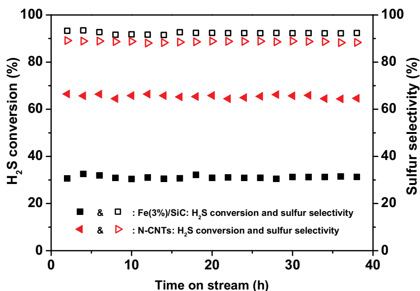
Fig. 1.15. Desulfurization performance on the N-CNTs and Fe 2 O 3 /SiC catalysts. Reaction conditions: reaction temperature = 230°C, O 2 -to-H 2 S molar ratio = 2.5, WHSV = 0.6 h -1 , steam = 30 vol.%. Results reproduced according to [142].
