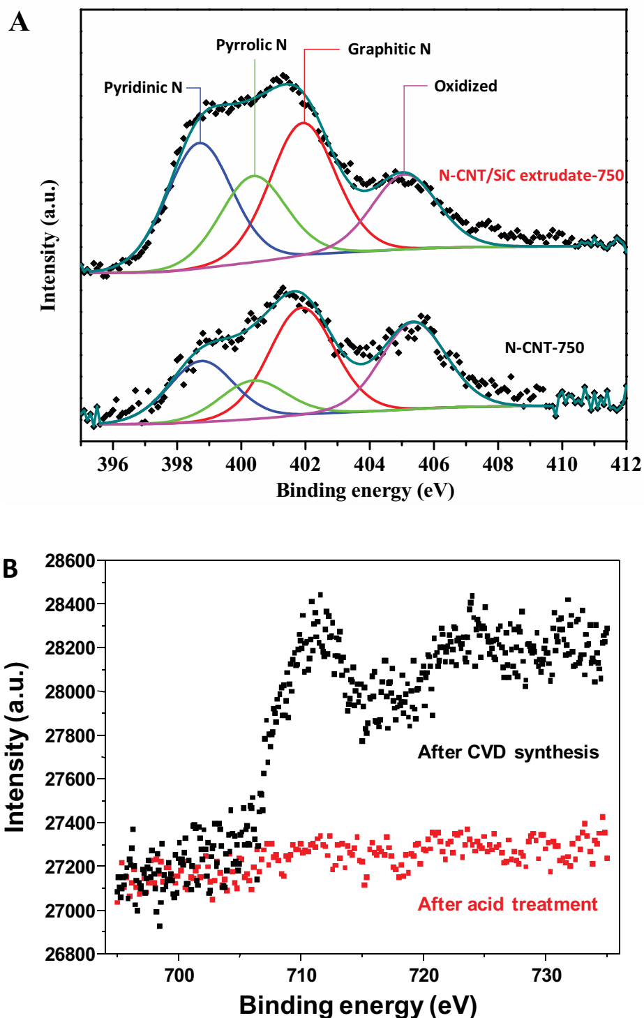
Fig. 2.6. (A) N1s XPS spectra on the N-CNT/SiC-750 and N-CNT-750 catalysts after acid treatment in HNO 3 (35 vol. %) at 80 °C for 6 h. (B) Fe2p XPS spectra recorded on the N-CNT-750 sample after CVD synthesis and after acid treatment.
