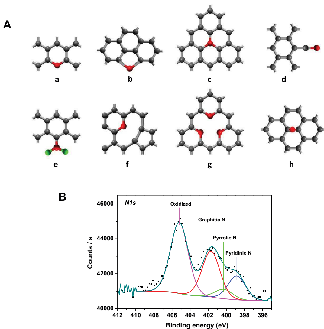
Fig. 1.10. (A) Different nitrogen bonding configuration in graphitic carbon network, (a) pyridine-like N, (b) pyrrole-like N, (c) quaternary or graphitic N, (d) nitrile -C\equiv N , (e) amine group -NH_2 , (f) pyridinic N-vacancy complex, (g) pyridinic N3-vacancy, (h) interstitial N. (B) XPS N1s analysis showing the presence of the different nitrogen species incorporated in the carbon matrix.
