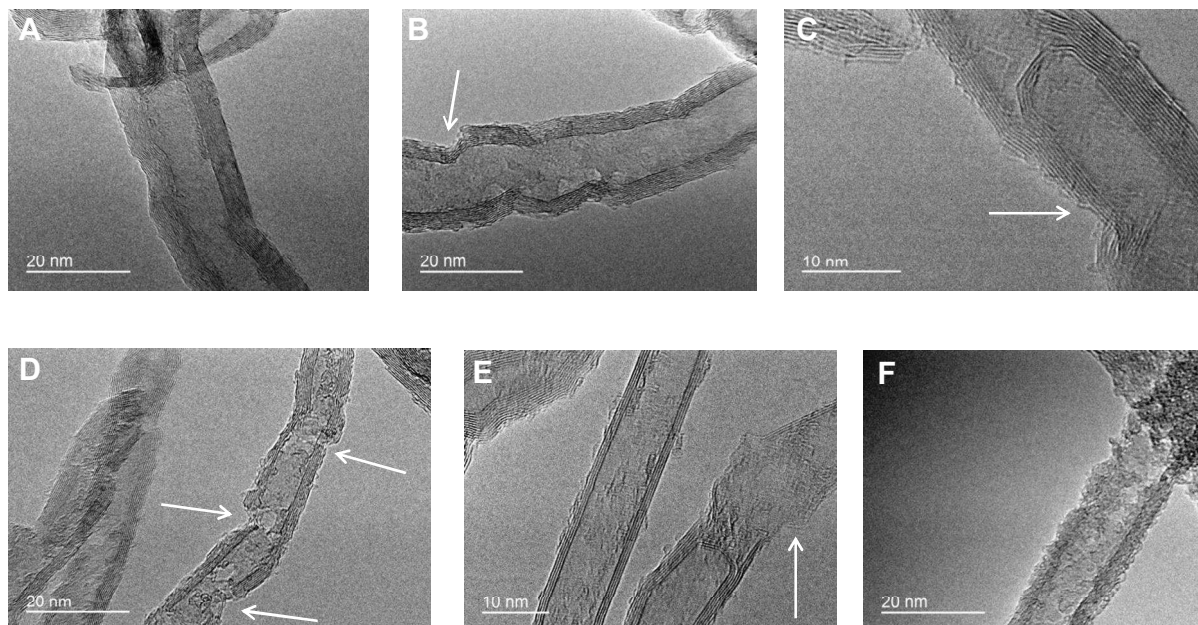
Fig. 4.2. Representative TEM micrographs: (A) Pristine graphitized CNTs, and (B), (C), (D), (E) and (F) oxidized CNTs as function of treatment temperature and duration. Sidewall defects are indicated with arrows.
