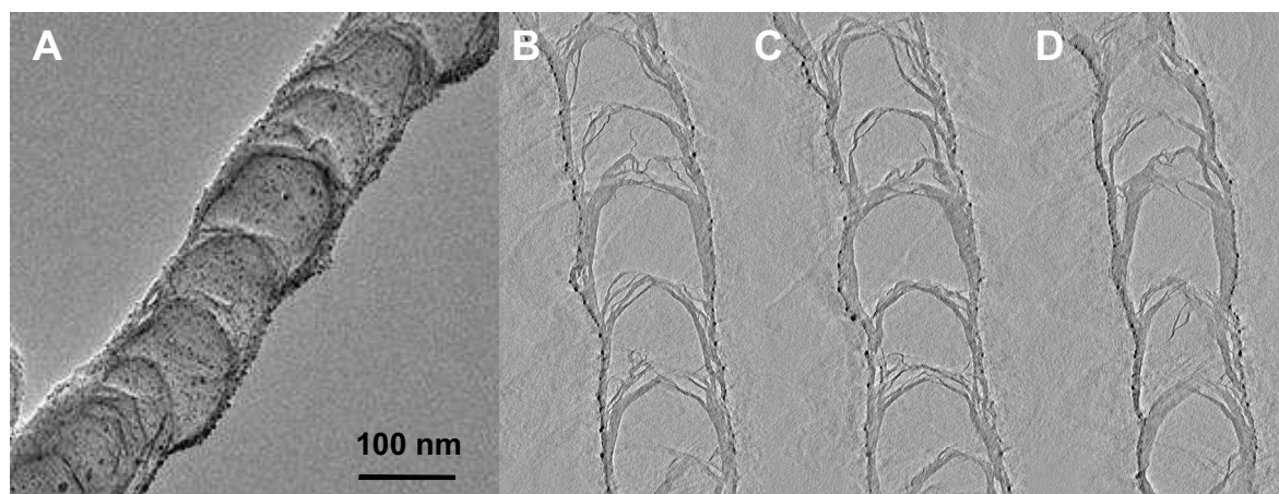
Fig. 1.8. (A) 2D TEM micrograph of the Pd/N-CNTs with 5 wt % loading. (B to D) 3D TEM sections showing the complete absence of Pd nanoparticles inside the N-CNT compartments.
