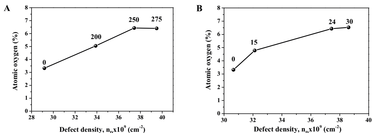
Fig. 4.5. (A) Amount of oxygen incorporated and defect density as a function of the acid treatment temperature. The treatment duration is keep at 24 h. (B) Amount of oxygen incorporated and defect density as a function of the acid treatment duration. The treatment temperature is keep at 250 °C.
