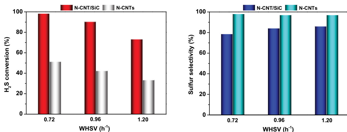
Fig. 1.18. Desulfurization performance, expressed in terms of H 2 S conversion, on the N-CNT/SiC and N-CNT catalysts. Reaction conditions: reaction temperature = 190 °C, O 2 -to-H 2 S molar ratio = 2.5, steam = 30 vol.%.
