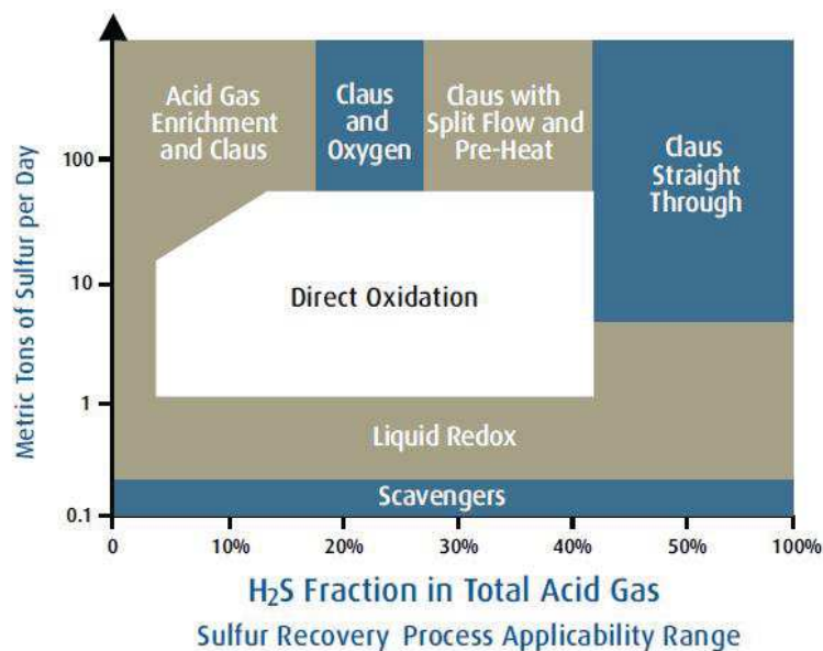
Fig. 1.21. Comparative chart of hydrogen sulfide conversion technologies [198].
