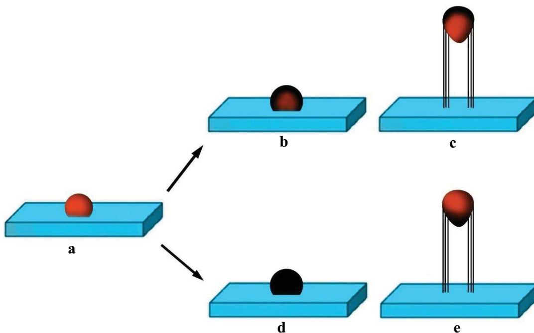
Fig. 1.6. Two ways grow the conventional CNTs in using CVD method: (a) decomposition of the carbon-containing precursor on the surface of the catalyst particles; (b, c) carbon species diffuse only on the surface of the catalyst particle; (d, e) diffusion of carbon atoms through the particles as a solid solution and precipitation of carbon at the metal-support interface and the formation of a nanofiber or a nanotube [33].
