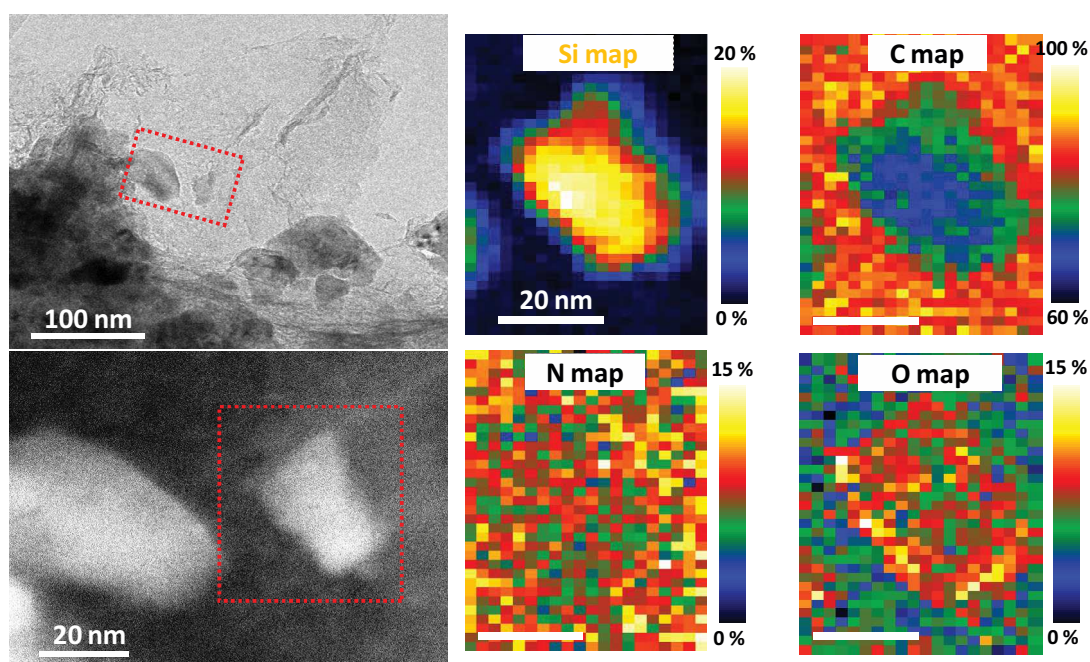
Fig. S8. Morphology of ^A\text{N@C/SiC}_p^2 [III] sample (Table S1, entry 3). An overview bright field TEM image (Top left). A high-angle annular-dark-field image (STEM-HAADF) which was taken from the area marked by the red dashed-line box in the top left image (Bottom left). Elemental maps of Silicon, Carbon, Nitrogen and Oxygen, respectively taken from the area highlighted by the red dashed-line box in the bottom-left image (Four color images on the right side). The colors correspond to the relative atomic composition ratio indicated by the adjacent vertical color bars.
