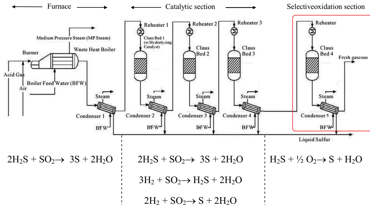
Fig. 1.24. Connecting Super-Claus process with Claus plans process for the ultimate sulfur recovery.
