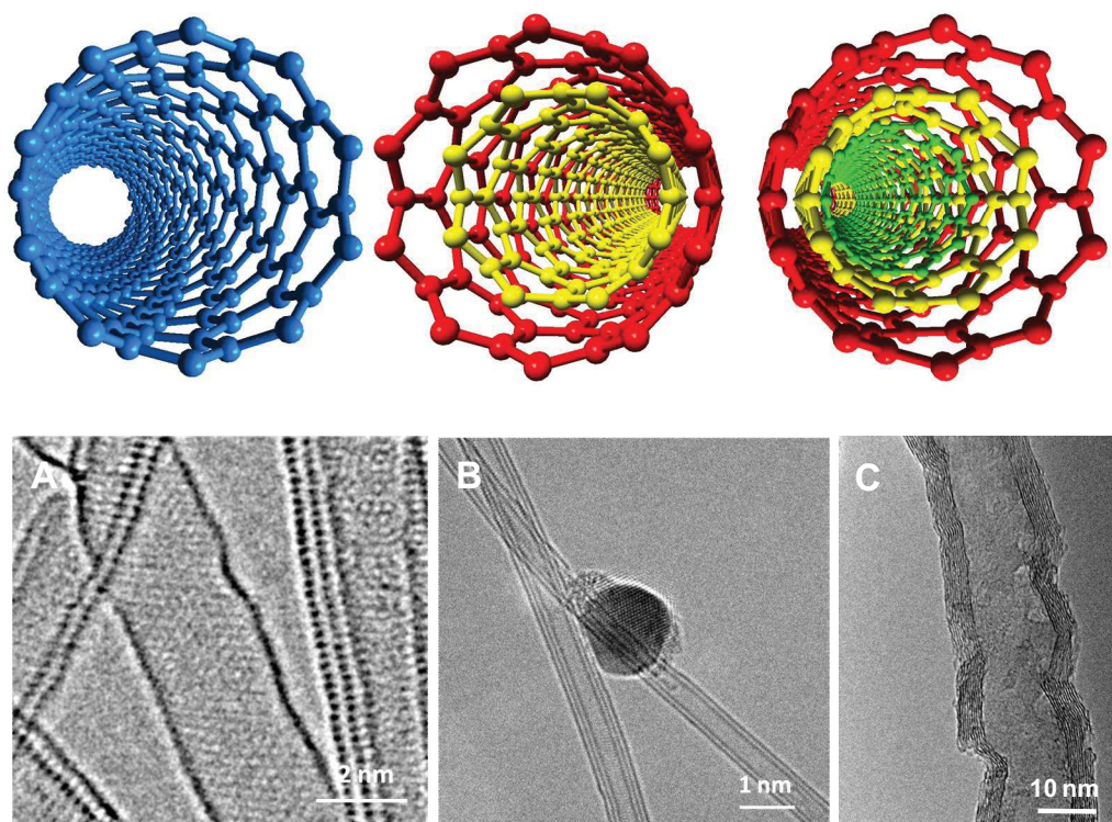
Fig. 1.1. Schematic representation of single-walled, double-walled and multi-walled carbon nanotubes and the corresponding TEM micrographs.
