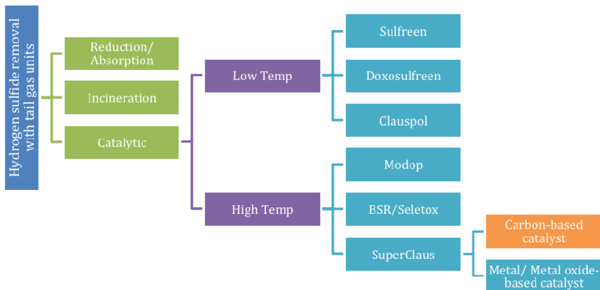
Fig. 1.23. Processes developed for hydrogen sulfide removal in tail gas.
