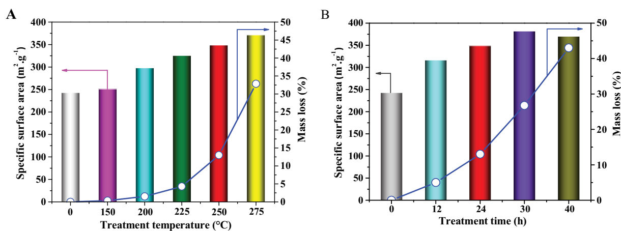
Fig. 4.3. Weight loss (open circles) and specific surface area (bares) modification of the acid treated carbon-based materials as a function of the treatment temperature with a duration fixed at 24 h (A) and duration at a fixed temperature of 250 °C (B).
