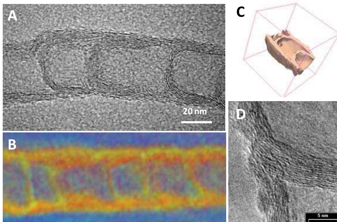
Fig. 1.7. (A) High-resolution TEM micrograph of the arches presented inside the N-CNT axis. (B) STEM-EELS results evidencing an enrichment of nitrogen in the area close to the arch. (C, D) TEM tomography and high-resolution TEM investigation of the microstructure of the N-CNTs evidencing the absence of pores or channel inside the arch.
