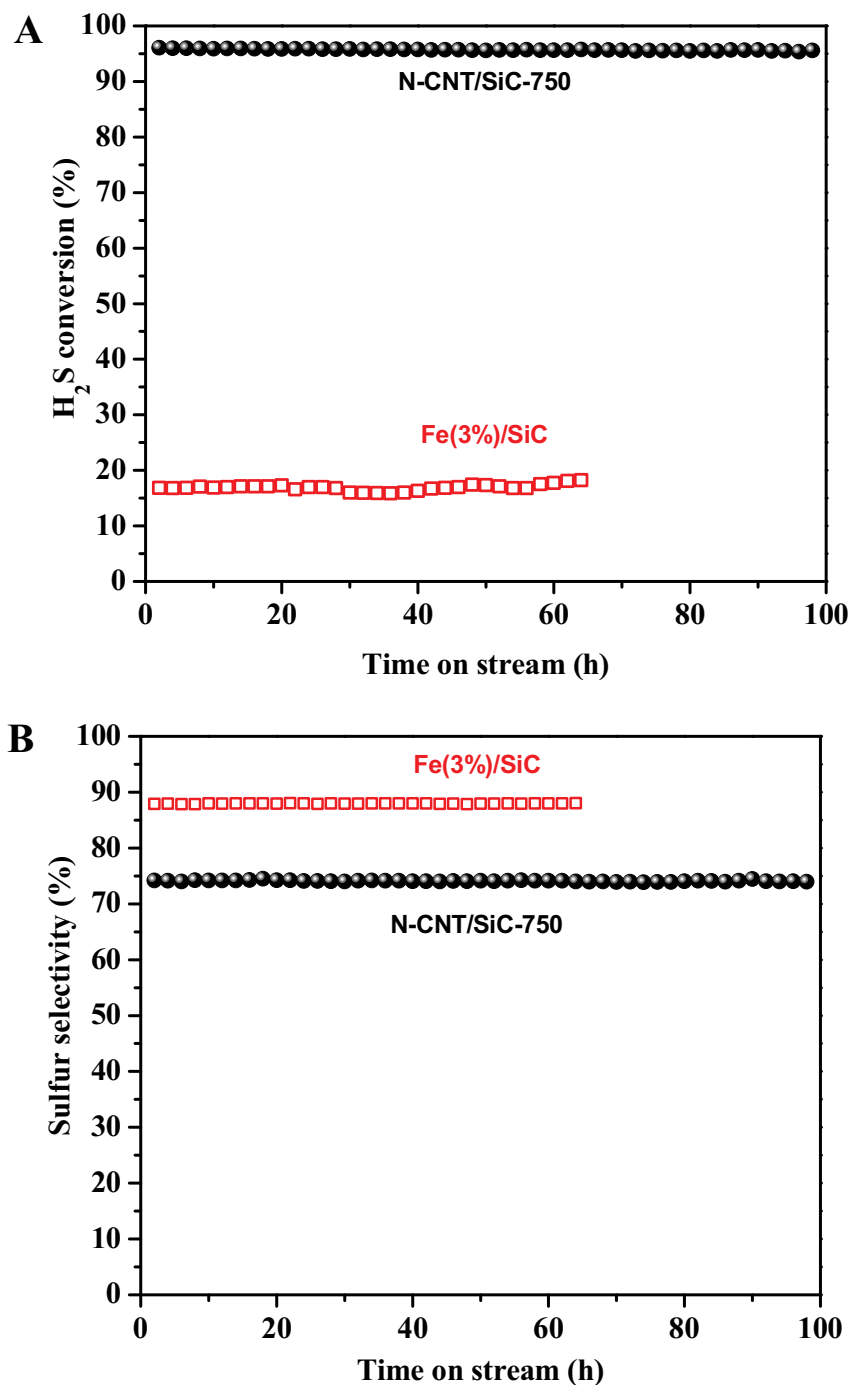
Fig. 2.11. Desulfurization conversion (A) and sulfur selectivity (B) on the N-CNT/SiC-750 and Fe 2 O 3 -3%/SiC catalysts. Reaction conditions: O 2 -to-H 2 S molar ratio = 2.5, reaction temperature = 190 °C, WHSV = 0.6 h -1 .
