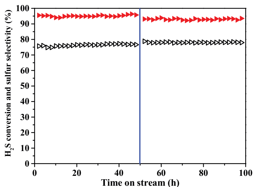
Fig. 4.13. Desulfurization activity on the O-CNT-250-24 before (A) and after thermal treatment under helium at 450 °C for 2 h (B). Reaction conditions: catalyst weight = 0.3 g; reaction temperature = 230 °C; WHSV = 0.6 h -1 , O 2 -to-H 2 S = 2.5.
