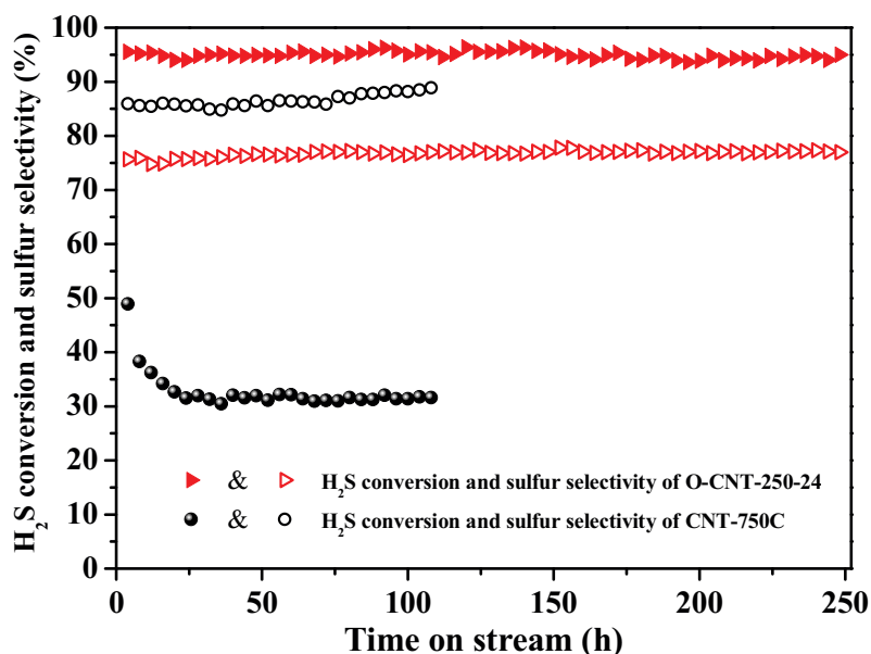
Fig. 4.7. Desulfurization conversion, sulphur selectivity on the O-CNT-250-24 compared to the CNTs graphitized (CNT-750C). Reaction conditions: catalyst weight = 0.3 g; reaction temperature = 230 °C; WHSV = 0.6 h -1 ; O 2 -to-H 2 S molar ratio = 2.5.
