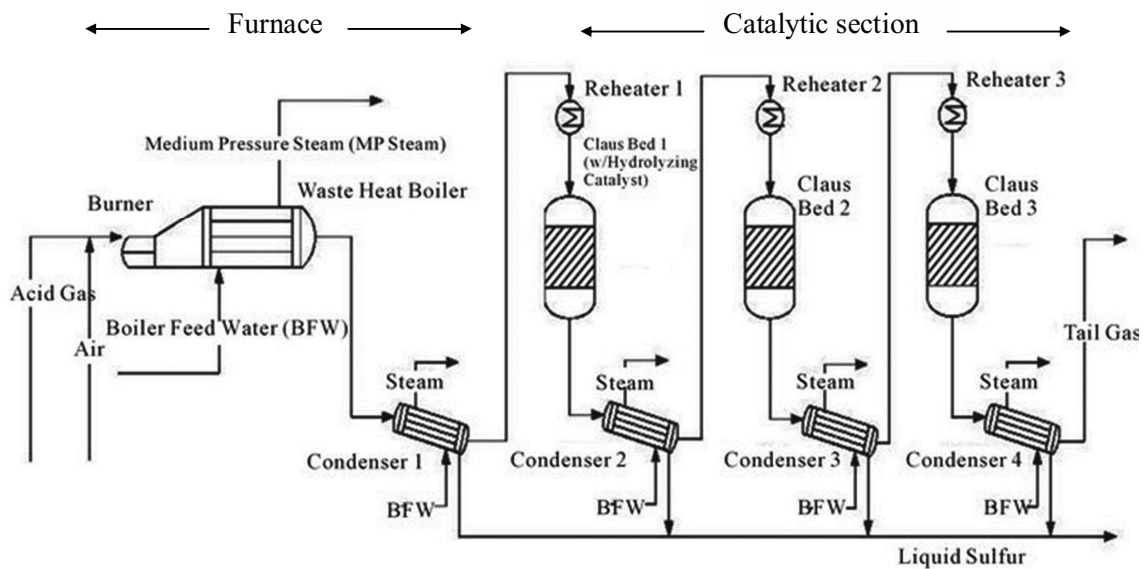
Fig. 1.22. Schematic flow diagram representation of the Claus process.
