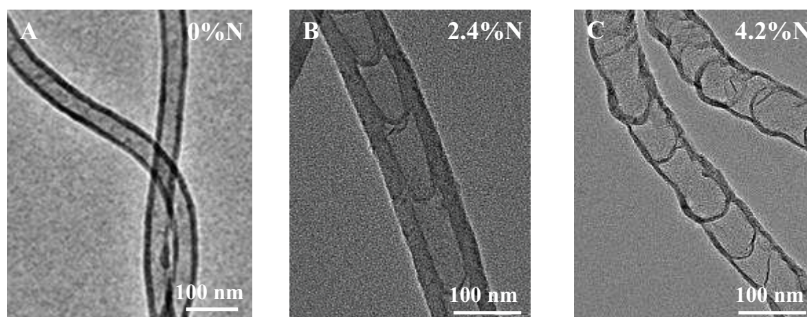
Fig. 1.11. TEM micrograph display the compartment of various nitrogen concentrations doped carbon nanotube by CVD method with using C_2H_6/NH_3/H_2 as carbon and nitrogen source and Fe/Al_2O_3 catalyst.
