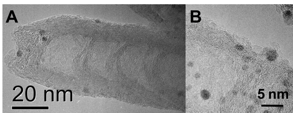
Fig. 1.12. Representative TEM micrographs of the Pd/N-CNTs catalyst used in the selective liquid-phase hydrogenation of cinnamaldehyde [55].
