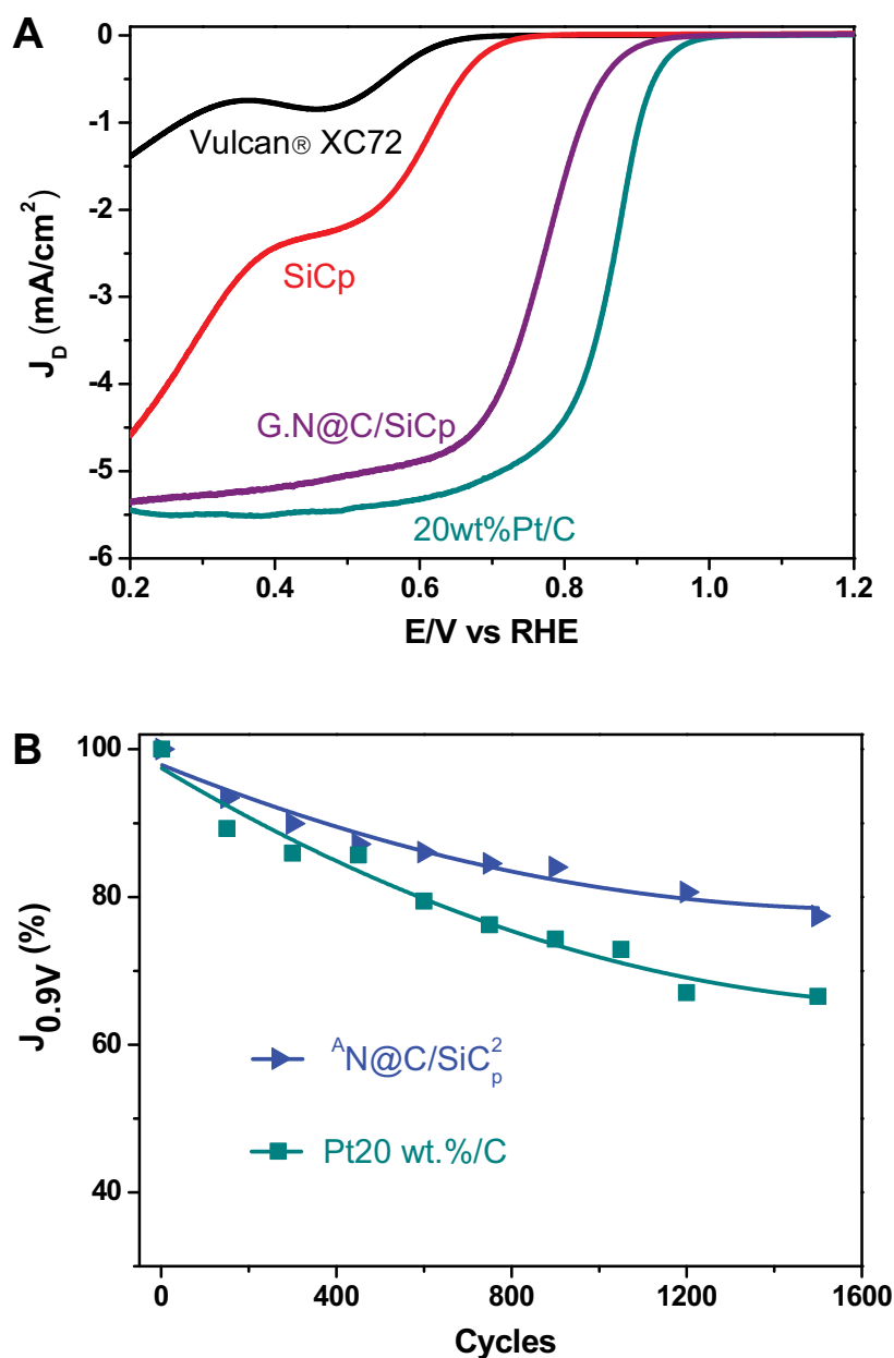
Fig. 3.3. Catalytic applications: (A) RRDE potential curves at 25 °C for ORR in O 2 saturated 0.1 M KOH solution recorded by a rotating ring-disk GC electrode [GC disk, A = 0.238 cm 2 ]. Curves recorded at 1600 rpm refer to [III] (< 40 μm, 450 μg.cm -2 ), Vulcan ® XC72 (100 μg.cm -2 ), 20 wt.% Pt/C (Vulcan ® XC72, 25 μg Pt .cm -2 ) and SiC p (< 40 μm, 450 μg.cm -2 ). (B) Long-term stability of [III] and 20 wt.% Pt/C catalysts at 25 °C and 1600 rpm in O 2 saturated 0.1 M KOH; the test was carried out for 1,500 cycles between 1.0 and 0.6 mV.
