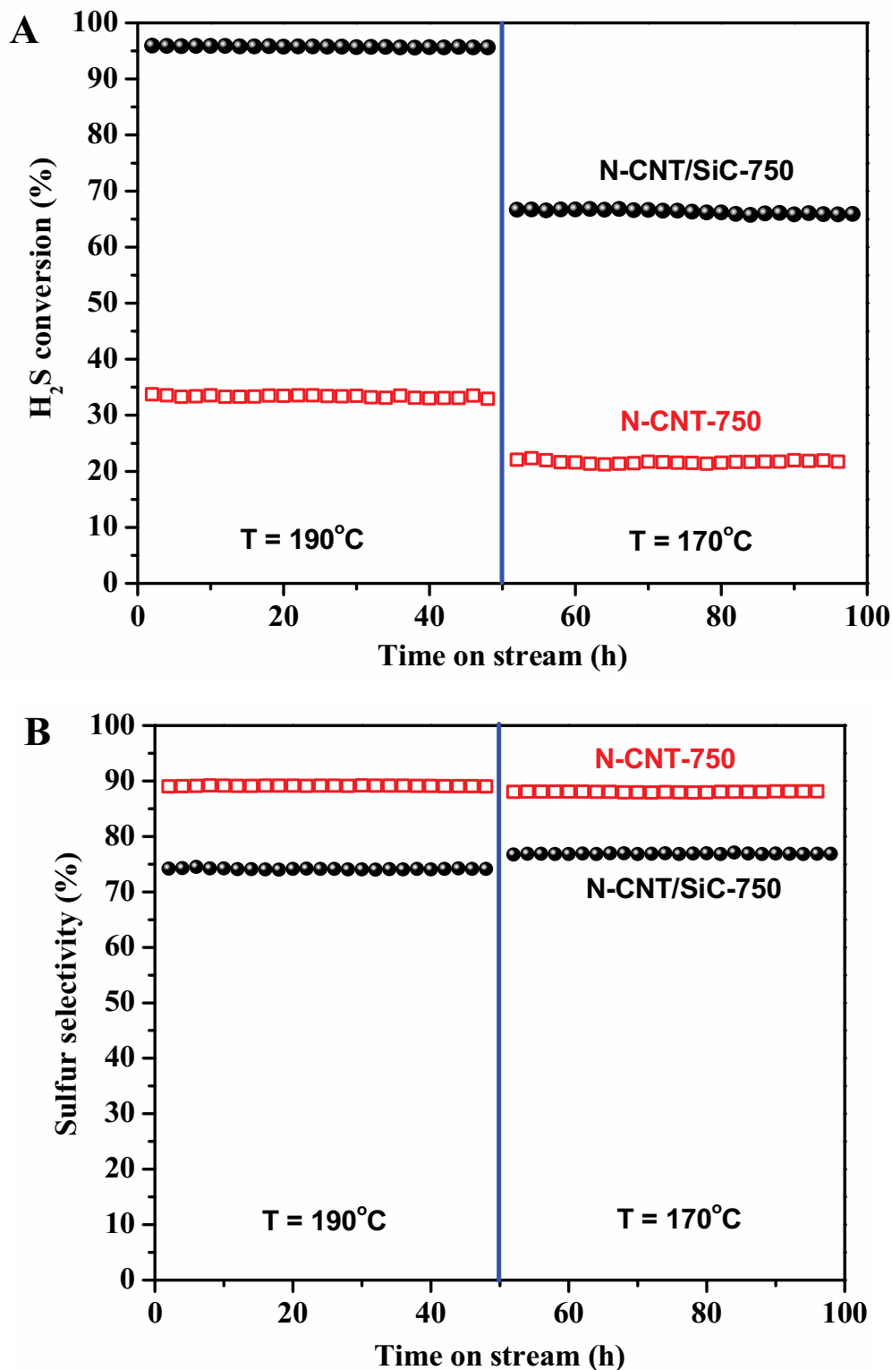
Fig. 2.7. Desulfurization conversion (A) and sulfur selectivity (B) on the N-CNT/SiC-750 and N-CNT-750 catalysts as a function of the reaction temperature. Reaction conditions: catalyst weight = 0.8 g, O 2 -to-H 2 S molar ratio = 2.5, reaction temperature = 170 – 190 °C, WHSV = 0.6 h -1 . The same catalyst was used for both tests.
