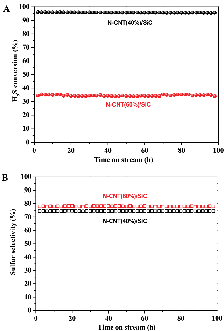
Fig. 2.9. Desulfurization performance, H 2 S conversion (A) and sulfur selectivity (B), on the N-CNT/SiC with different N-CNTs loading, i.e. 40 and 60 wt.%, catalysts, synthesized at 750 °C. Reaction conditions: O 2 -to-H 2 S molar ratio = 2.5, reaction temperature = 190 °C, WHSV = 0.6 h -1 .
