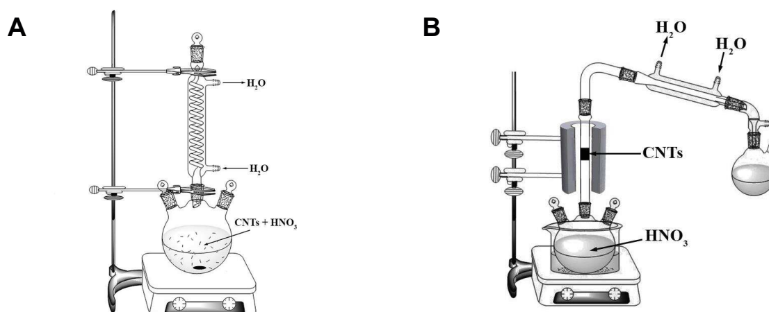
Fig. 1.9. Illustration of the setup used for (A) liquid-phase, where the CNTs are treated at the same temperature in the presence of the oxidizing agent, and (B) gas-phase functionalization of CNTs where the pre-treatment temperature of the CNTs can be tuned with respect to the temperature of the oxidizing chemical agent.
