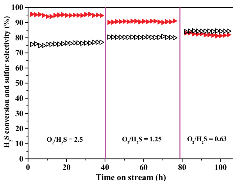
Fig. 4.10. Desulfurization activity and sulfur selectivity of the O-CNT-250-24 as a function of the O 2 -to-H 2 S molar ratio. Reaction conditions: catalyst weight = 0.3 g; reaction temperature = 230 °C; WHSV = 0.6 h -1 .
