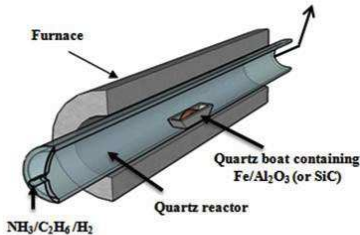
Fig. 1.5. Schematic diagram of fixed bed catalyst CVD apparatus [32].
