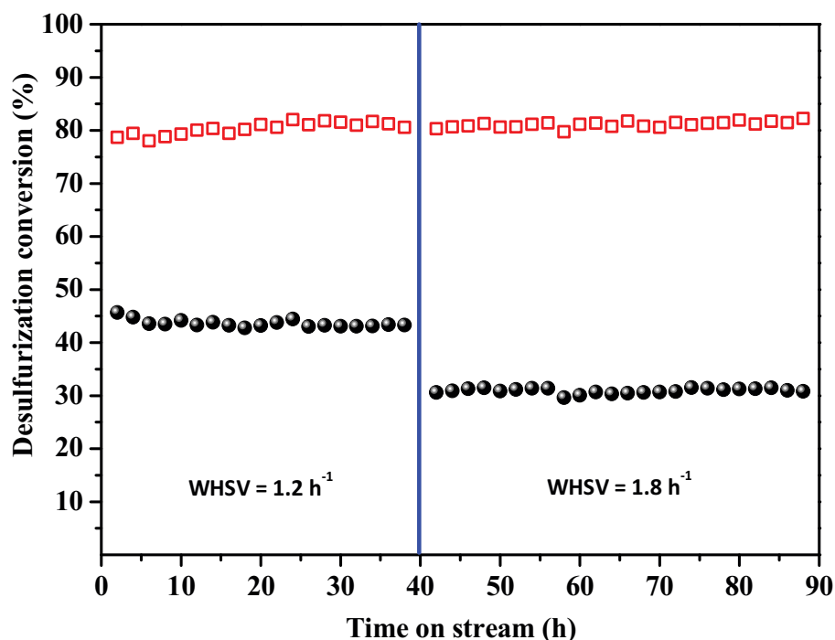
Fig. 2.8. Desulfurization performance at high space velocity on the N-CNT/SiC-750 catalyst. Reaction conditions: catalyst weight = 0.4 g, O 2 -to-H 2 S molar ratio = 2.5, reaction temperature = 190 °C, WHSV = 1.2 and 1.8 h -1 . The same catalyst was used for both tests.
