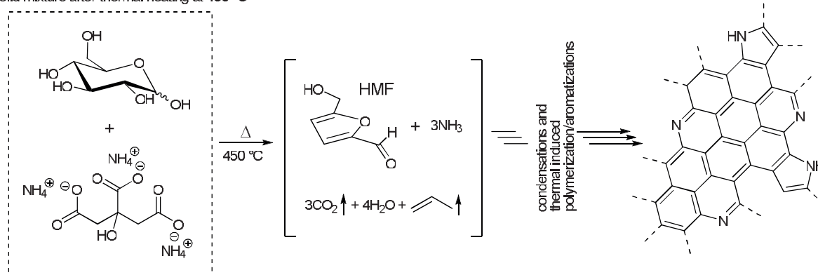
Fig. S3. Proposed mechanism for the thermal transformation of \alpha,\beta -D-glucopyranose and ammonium citrate tribasic (pre-catalyst phase) into a N-rich, heteroaromatic, graphene-like network (N@C - catalytically active phase). The thermal treatment at 450 °C is supposed to start the progressive dehydration of the sugar into the 5-hydroxymethyl-furfural (5-HMF) [2]. Under these conditions, ammonium citrate tribasic, is expected to act as both a N-reservoir for the generation of N-containing heterocycles [3,4] and a pore-forming agent (due to its complete decomposition into volatiles like \text{NH}_3 , \text{CO}_2 , \text{H}_2\text{O} and propene) thus contributing to the ultimate material mesoporosity.
