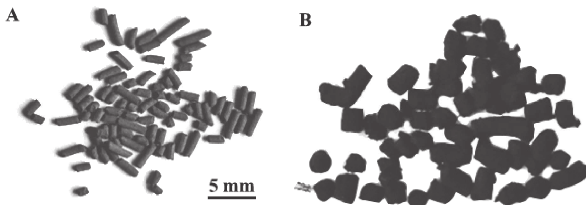
Fig. 2.3. Digital photos of the SiC before (A) and after (B) N-CNTs loading carried out at 750 °C showing the significant increase of the apparent volume of the catalyst due to the formation of a high surface-to-volume N-CNTs.
