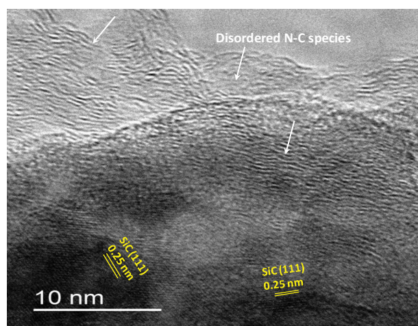
Fig. S7. HR-TEM high-resolution image of the ^A\text{N@C/SiC}_p^2 [III] sample (Table S1, entry 3) showing the N@C coating phase in the form of disordered and crumpled N-doped carbons at the SiC support.
