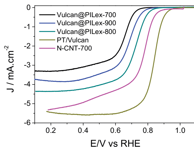
Fig. 1.13. ORR performance of the different N-CNTs and the commercial Pt/Vulcan catalysts. N-CNT-700: nitrogen-doped carbon nanotubes synthesized by a CVD method at 700°C, Vulcan@PILex-X: nitrogen-doped carbon layer synthesized from a thermal decomposition of the polymerized ionic liquids (PILs) at different temperatures.
