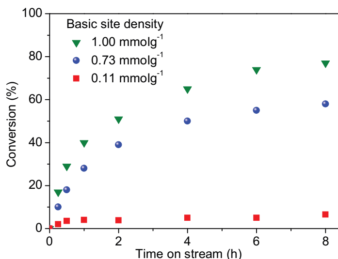
Fig. 1.16. Effect of the amount of grafted triethylamine on the transesterification activity, expressed in terms of glyceryltributyrate conversion, on the nitrogen-grafted CNTs catalysts. Reaction conditions: Temperature = 60°C, glyceryltributyrate to methanol ratio = 1:12, catalyst weight= 2 wt.% versus the reactant mixture. Results reproduced from [146].
