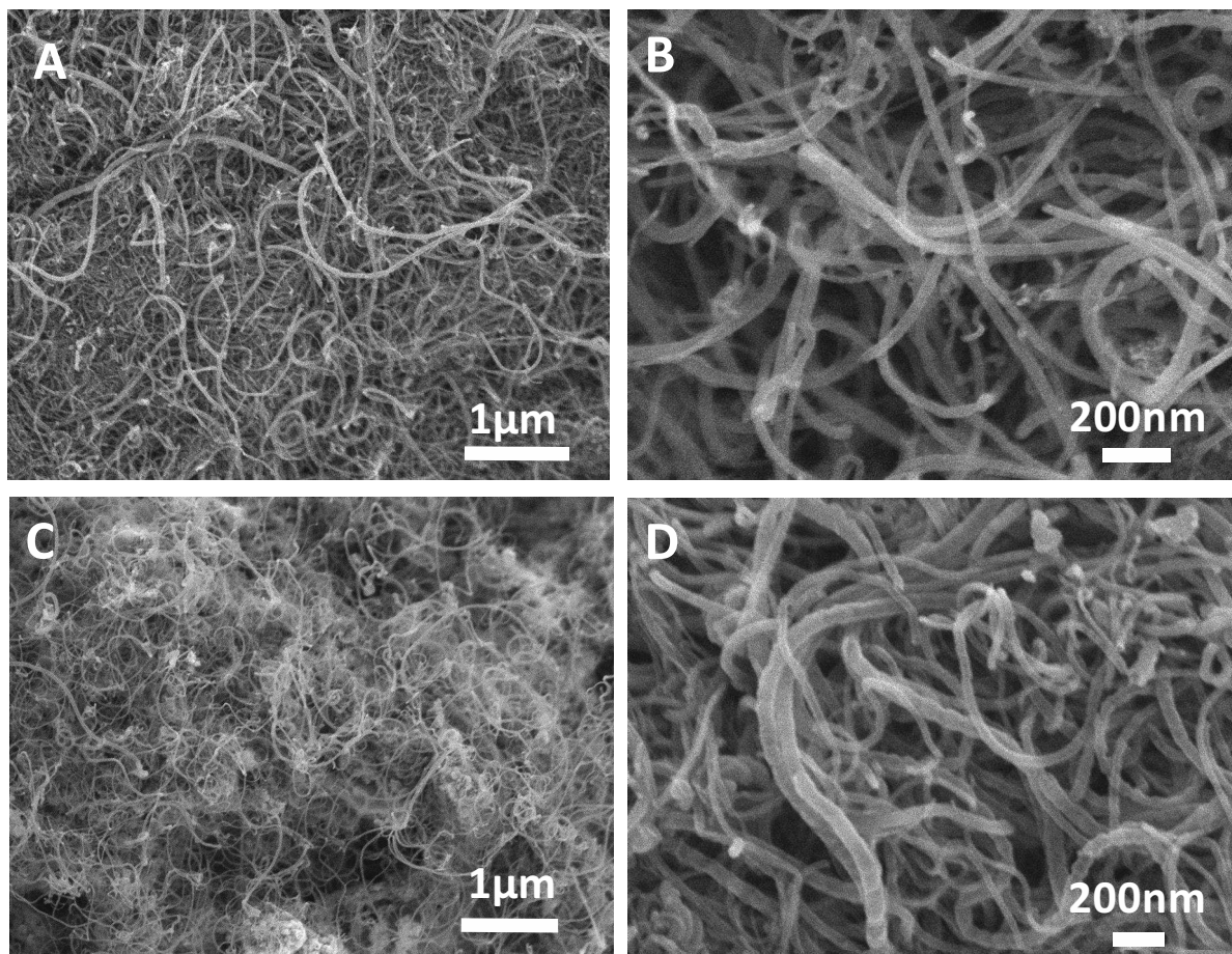
Fig. 2.4. SEM micrographs of the N-CNT/Al 2 O 3 synthesized at 750 °C (A and B) and the N-CNT/SiC synthesized at 750 °C (C and D) composites showing the high coverage of the SiC surface by the N-CNT network.
