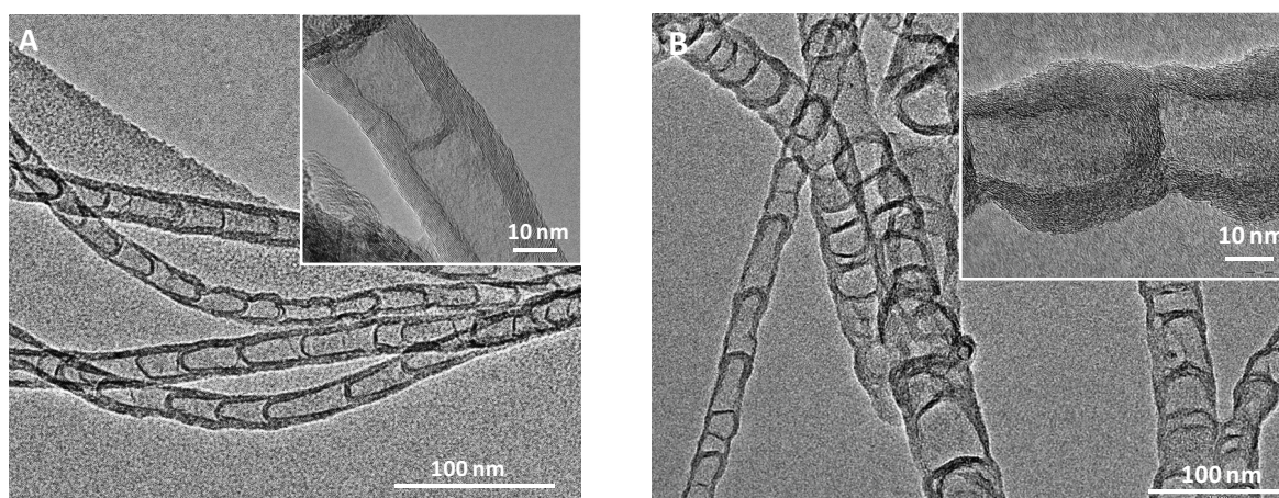
Fig. 2.5. TEM micrographs of the N-CNTs (A) and the N-CNT/SiC (B) synthesized at 750 °C with similar closed periodical bamboo-like structure.
