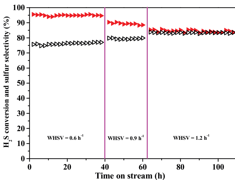
Fig. 4.9. Desulfurization activity and sulfur selectivity of the O-CNT-250-24 as a function of the WHSV. Reaction conditions: catalyst weight = 0.3 g; reaction temperature = 230 °C; O 2 -to-H 2 S molar ratio = 2.5.
