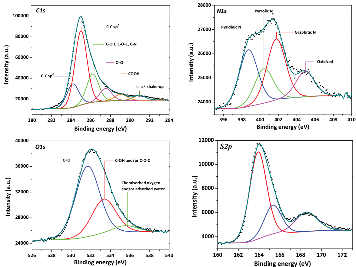
Fig. 2.12. XPS analysis of the N-CNT/SiC-750 catalyst after desulfurization reaction showing the formation of sulfur on the spent catalyst.
