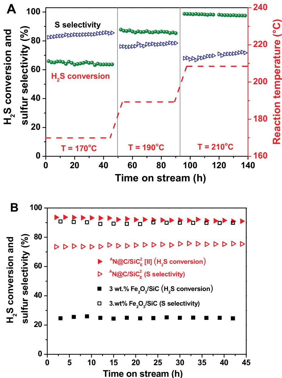
Fig. 3.4. (A) Desulfurization performance on [II] as a function of the reaction conditions (1g of [II], O 2 /H 2 S molar ratio = 2.5, WHSV = 0.3 h -1 ). (B) Comparative study of H 2 S conversion and sulfur selectivity over [II] and 3 wt.% Fe 2 O 3 /SiC catalysts (operative conditions: T = 210 °C, 1g of catalyst, O 2 /H 2 S molar ratio = 2.5, WHSV = 0.6 h -1 ).
