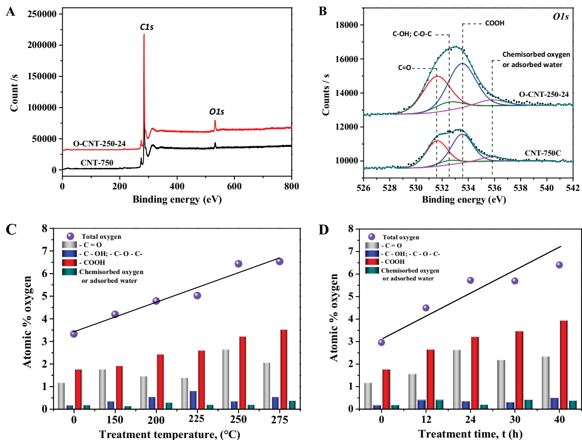
Fig. 4.4. (A) Survey XPS of O-CNT-250-24 in comparison with pristine graphitized CNTs, (B) deconvolution O1s present the oxygen species on the surface of the CNTs wall, (C, D) Oxygen species distribution of the acid treated carbon-based materials as a function of the treatment duration and temperature in comparison with the pristine graphitized CNTs.
