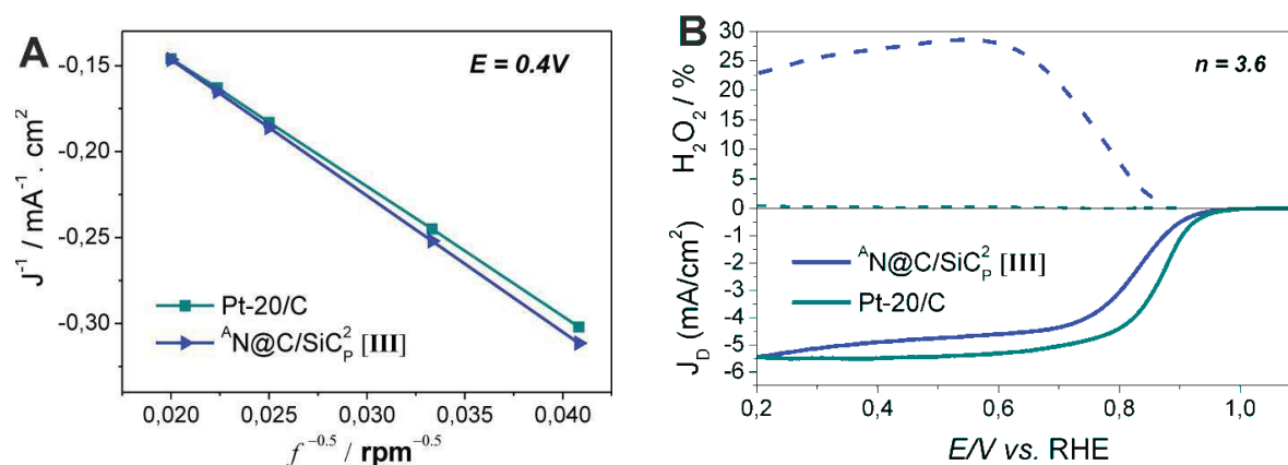
Fig. S9. (A) K-L plots for [III] and the reference 20 wt.% Pt/C catalysts as obtained from the respective LSVs at 0.4 V (vs. RHE). Parameters used: O_2 concentration (C), 1.15 \times 10^{-3} \text{ mol.L}^{-1} ; O_2 diffusion coefficient (D), 1.95 \times 10^{-5} \text{ cm}^2.\text{s}^{-1} ; kinematic viscosity ( \nu ) of the electrolyte solution, 0.008977 \text{ cm}^2.\text{s}^{-1} . (B) [down] RRDE current - potential curves at 25 °C for ORR in O_2 saturated 0.1 M KOH solution recorded by using a rotating ring-disk GC electrode [GC disk, A = 0.238 \text{ cm}^2 ] with (B) [top] Pt ring [ A = 0.234 \text{ cm}^2 ]. Both samples ([III] and 20 wt.% Pt/C) are measured at an angular rotation rate ( f ) of 1600 rpm.
