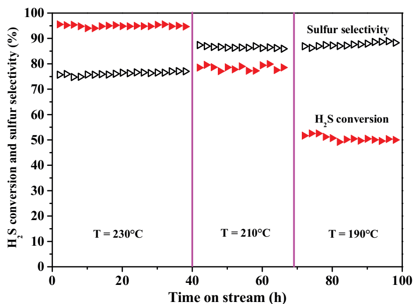
Fig. 4.8. Desulfurization activity and sulfur selectivity of the O-CNT-250-24 as a function of the reaction temperature. Reaction conditions: catalyst weight = 0.3 g; WHSV = 0.6 h -1 ; O 2 -to-H 2 S molar ratio = 2.5.
