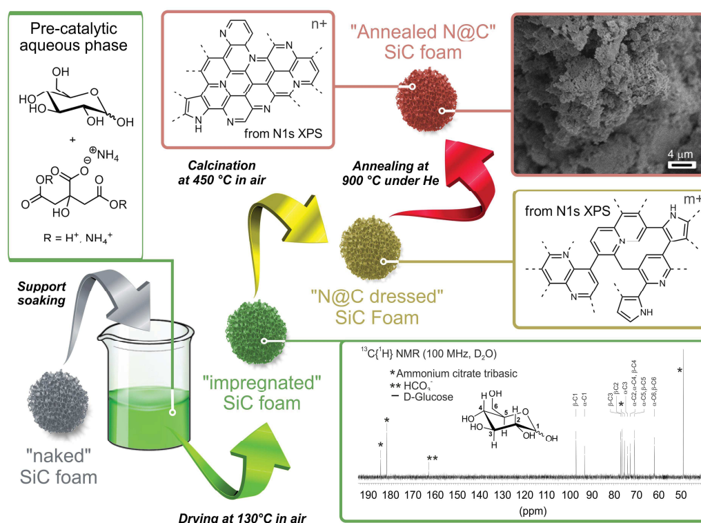
Fig. 3.1. Synthesis of a highly N-doped carbon-based coating (N@C) on a macroscopically shaped host matrix (SiC foam). Arrows refer to the sequential synthetic steps; from the material soaking and drying up to its calcination at 450 °C in air followed by annealing at 900 °C under inert atmosphere.
