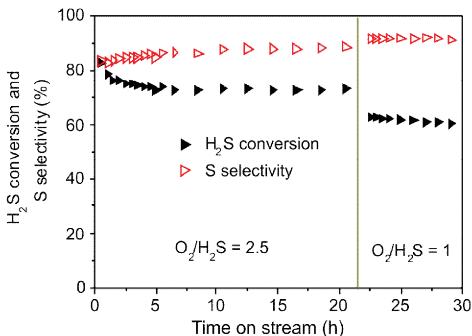
Fig. S10. H_2S conversion and sulfur selectivity on ^A N@C/Al_2O_3B^2 catalyst (VI) under two O_2/H_2S molar ratio. Reaction conditions: M_{\text{catal}} = 1 \text{ g} ; T = 230 \text{ }^\circ\text{C} , WHSV = 0.6 \text{ h}^{-1} .
