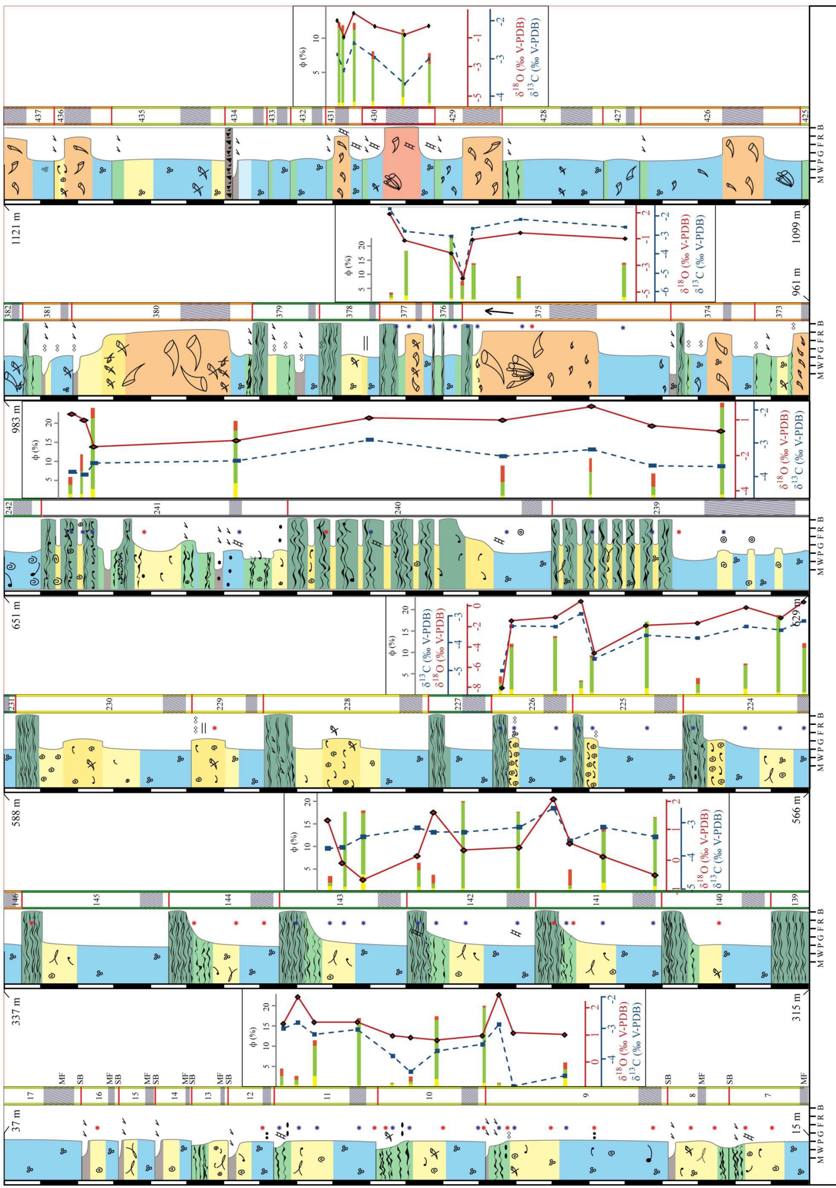
Figure 3-27: Staking pattern and facies evolution of six intervals, respectively from the left to the right: SQ 7-17; SQ 139-146; SQ 239-242; SQ 224-231; SQ 139-146; SQ 239-242; SQ 373-382 and SQ 426-437. Stable isotopes ( \delta^{13}\text{C} & \delta^{18}\text{O} ) are displayed for the corresponding SQ. Facies and SQ colors, textures, diagnostic structures and sedimentary structures, facies elements and reservoir properties charts legends are explained in figure 3-24.
