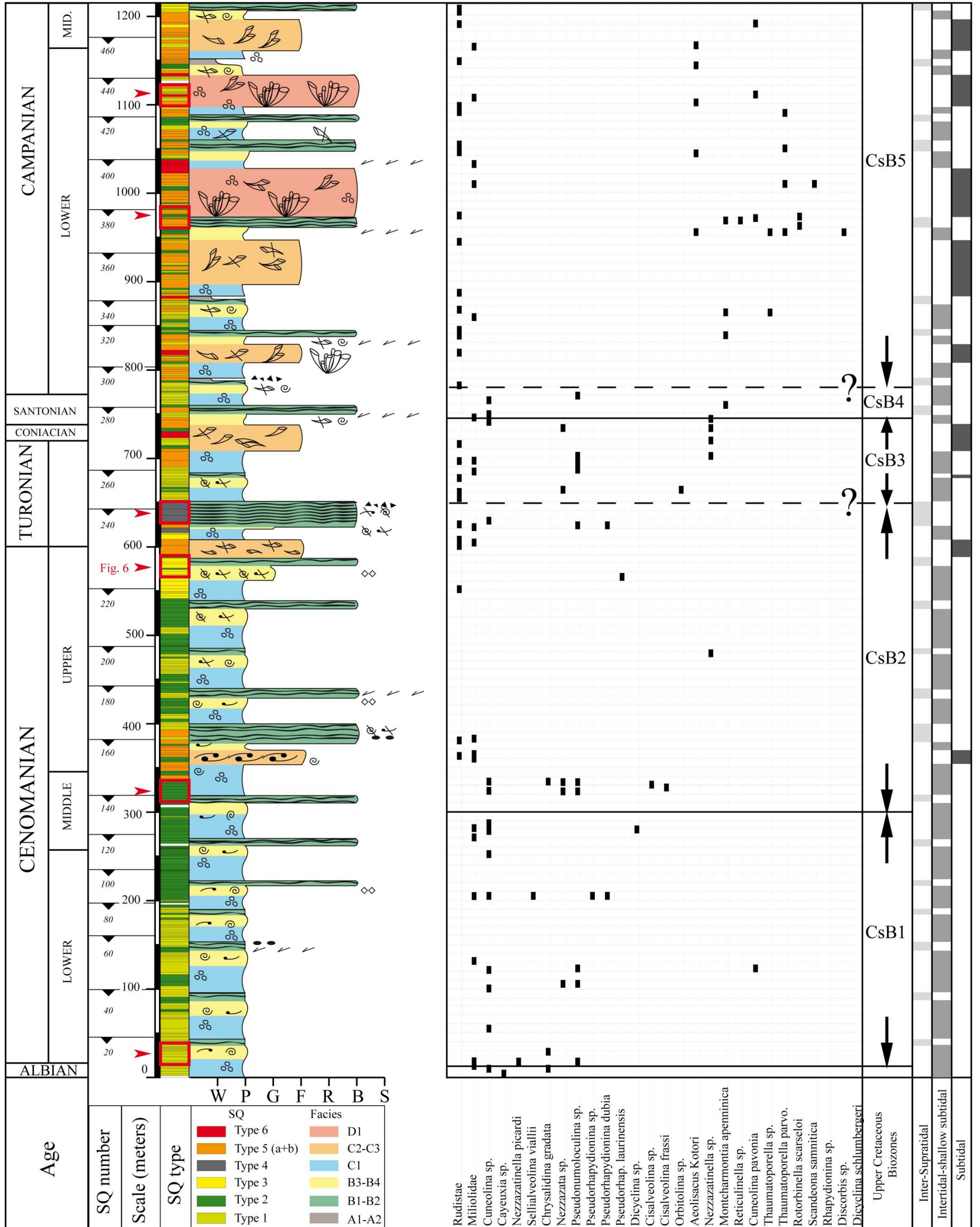
Figure 3.24: Simplified lithostratigraphy of the Llogara pass succession with associated biostratigraphy and depositional environments. Each identified SQ is mentioned next to the litholog, they are specifically described in the result part. Red squares indicate the location of six intervals presented in Fig. 3.27. Biozones (CsB) as defined by Fleury (1980). Abbreviation: parvo. for parvovesicularifera.
