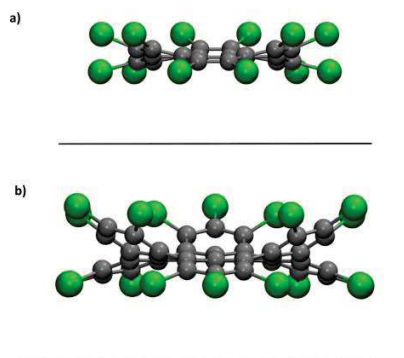
Figure 5.3 : Side-view of the optimized geometries for the adsorption of a) coronene and b) molecule 2 ( C_{42}Cl_{18} ) on graphene (represented with a grey line). The green spheres represent the chlorine atoms while the grey spheres represent the carbon atoms.
