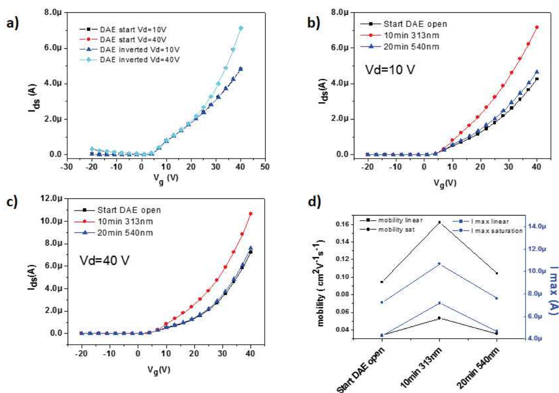
Figure 6.22 :Electrical characterization of a device with both electrodes covered by AZO SAMs of channel length 100 \mu m ; a) transfer characteristics in linear ( V_d=10V ) and saturation regime ( V_d=40V ) grounding alternatively one of the two electrodes; b) transfer characteristics in the linear regime showing a switching cycle of diarylethene: start(black), transfer after illumination at 313 nm (red) and transfer after illumination at 530 nm (blue); c) transfer characteristics in saturation regime showing a switching cycle of diarylethene: start (black), transfer after illumination at 313 nm (red) and transfer after illumination at 530 nm (blue); d) mobility and maximum drain current in saturation regime plotted for all the transfer curves depicted in fig. b) and c).
