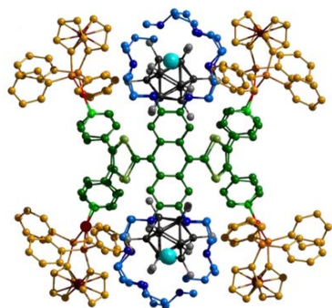
(B_{12}F_{12})_2 \subset AA9
