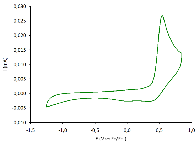
Figure 88 : Voltammogramme cyclique de (3-Py)Fluo-DTF : C = 1,0 \text{ mM} , \text{CH}_2\text{Cl}_2 , ( n\text{-Bu}_4\text{NPF}_6 ( 0,1 \text{ M} )), 100 \text{ mV}\cdot\text{s}^{-1} , carbone vitreux, vs. \text{Fc}/\text{Fc}^+ .
