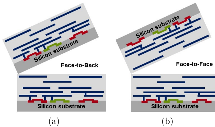
FIGURE B.4: (a) la configuration de 3D Face-à-dos, (b) la configuration de 3D face-à-face.
