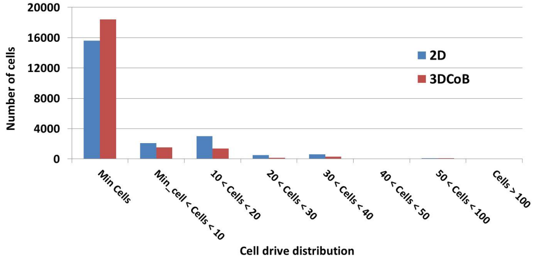
FIGURE 3.9: Comparison of standard cell driving size distribution for the FFT block implementation at target frequency = 1.67GHz for both 2D and 3DCoB libraries.
