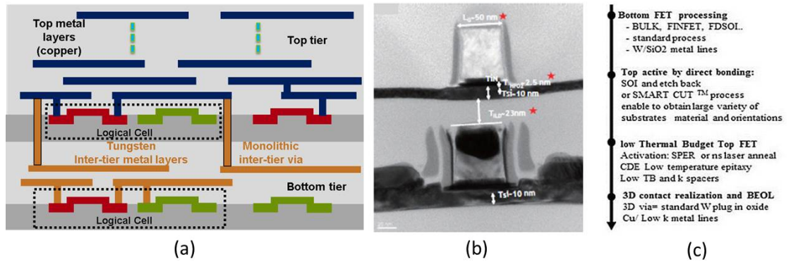
FIGURE B.7: Monolithique 3D technologie [8].
