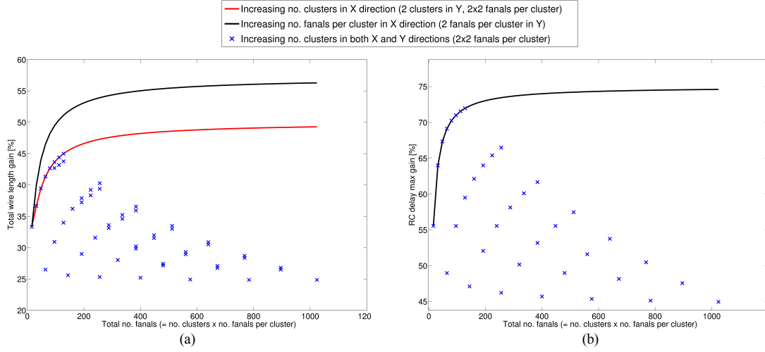
FIGURE A.6: (a) Total wire length gain (b) maximal RC delay gain in function of the total number of fanals n for different network dimensions.
