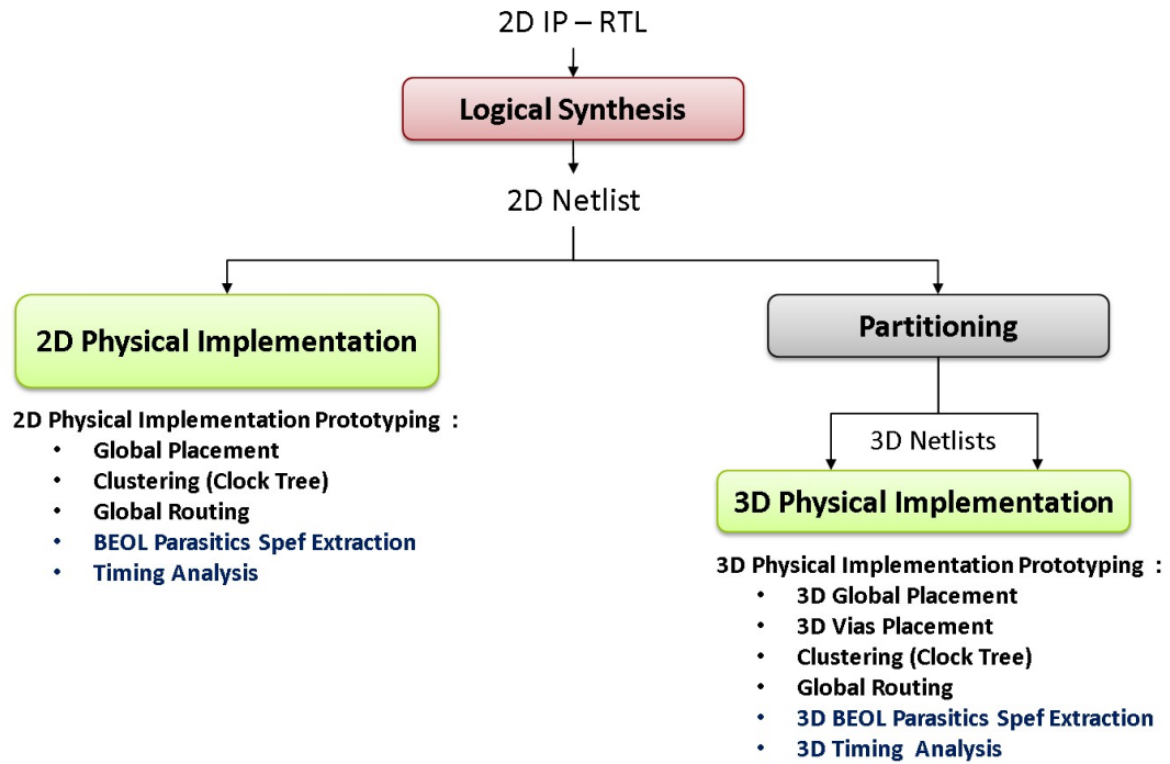
FIGURE 2.11: 2D/3D Design Implementation Framework.
