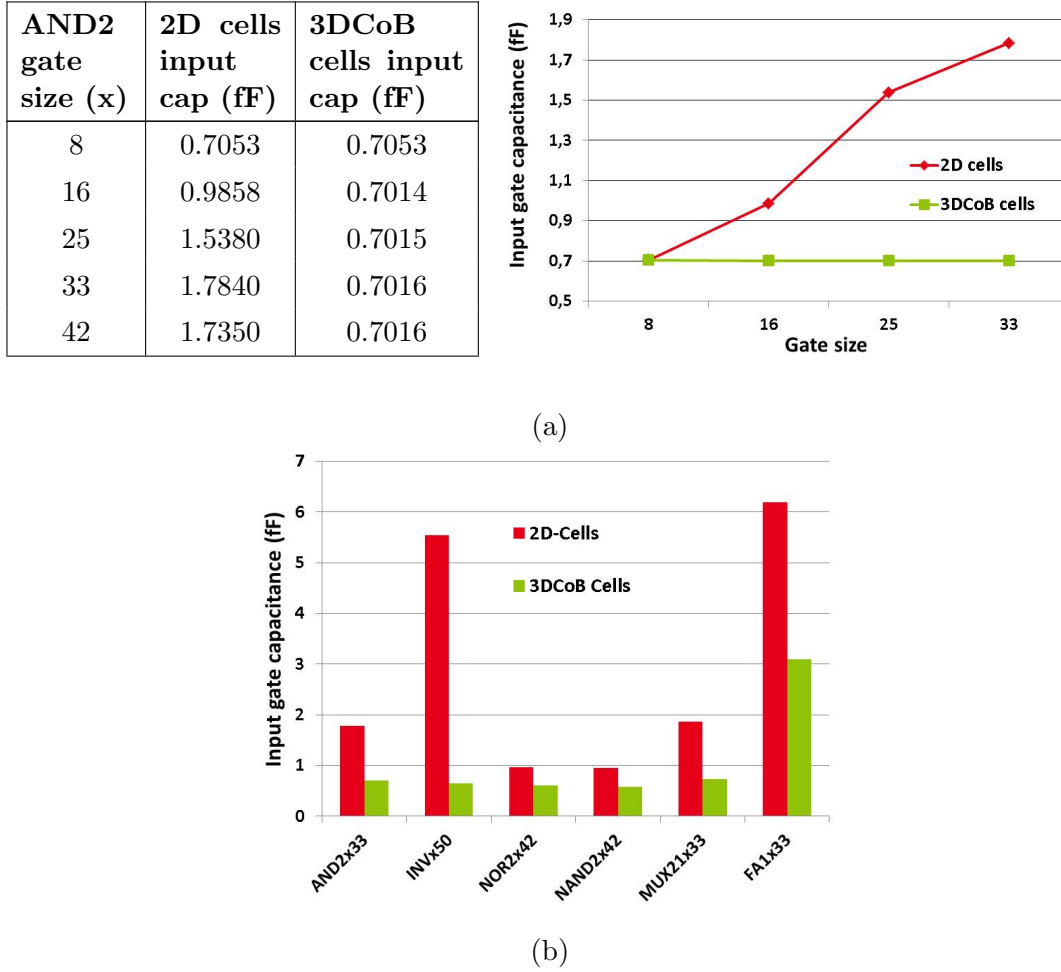
FIGURE 3.3: Input gate capacitance results for 2D and 3DCoB cells (in fF), where (a) shows input cap of one gate as an example ‘2-input AND’ at different driving, and (b) shows different cell types and drives.
