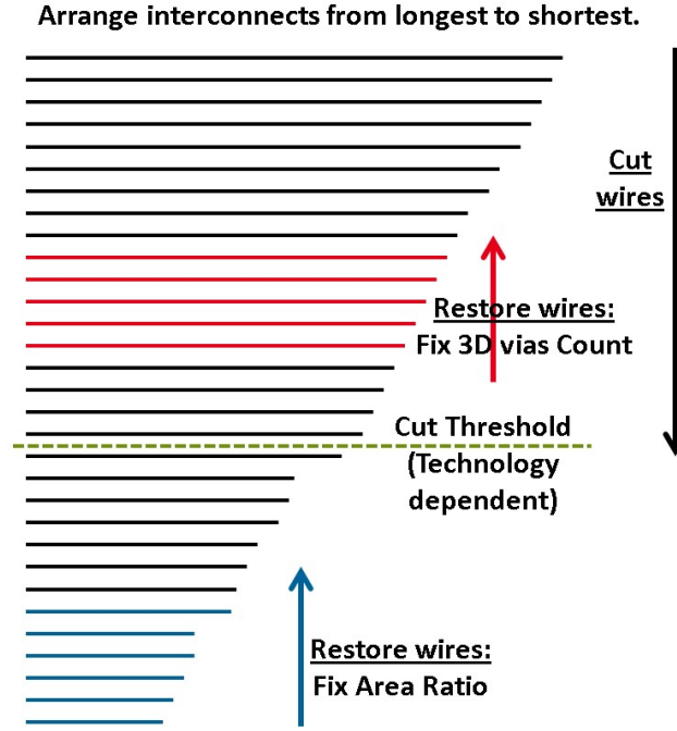
FIGURE 4.3: Bi-Directional Partitioning (BDP) diagram showing the design nets arranged from the longest net to the shortest net where the cut wires is performed from the longest to the shortest one (down arrow) till a certain Cut Threshold, and restore wires is performed from the shortest to the longest (up arrows).
