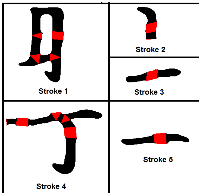
Figure 3.34 : Strokes extraits
