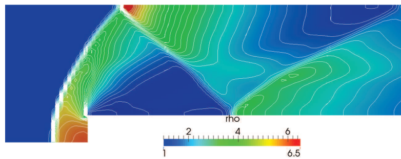
(ii) Approximated solution for 4 units of time obtained with a MUSCL scheme with MINMOD limiter and first order van Leer flux scheme
