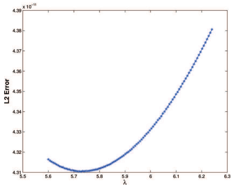
Figure 2.19: Research for the optimal Robin coefficient for an overlap equal to 3 cells. The research has been done for converged solution inside the Schwarz process.
