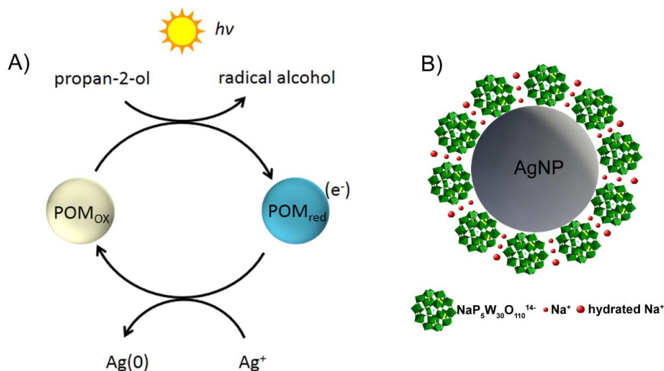
Fig. 6.4 Schematic mechanism of POM-catalyzed photochemical synthesis of \text{Ag}^+ to \text{Ag}(0) nanoparticles, the model structure of \text{P}_5\text{W}_{30}\text{O}_{110} @AgNPs..
