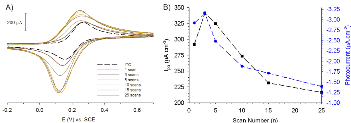
Fig. 4.12 A) CVs of 1 mM 1,1-ferrocenedimethanol in aqueous solution with \text{Na}_2\text{SO}_4 ( 0.5 \text{ mol.L}^{-1} ) at modified ITO electrode with poly-POM-14,4-ZnOEP films deposited after 1 to 25 scans between -0.05 and +1.90 V vs. SCE (full line) and at non-coated ITO electrode (dotted line). v=100 \text{ mV s}^{-1} . B): (●) plots of the photocurrent measured in aqueous solution containing \text{Na}^+ \text{I}_3^- 0.1 \text{ mol L}^{-1} and \text{Na}^+ \text{I}^- 0.5 \text{ mol L}^{-1} vs. the numbers of iterative scans. (■) plot of the anodic peak current in aqueous solution of 0.5 \text{ mol L}^{-1} \text{ Na}_2\text{SO}_4 and 1 \text{ mmol L}^{-1} 1,1-ferrocenedimethanol vs. the numbers of iterative scans.
