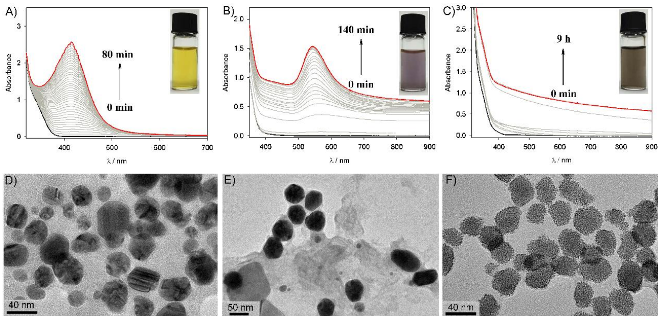
Fig. 6.5 Absorption spectra of metal nanoparticles (Ag, Au, Pt) in aqueous solution, obtained under UV-vis irradiation \text{Na}_{14}[\text{NaP}_5\text{W}_{30}\text{O}_{110}] ( \text{P}_5\text{W}_{30} ) with the corresponding metal ions A) 2\text{Ag}^+ \text{SO}_4^{2-} (0.2 mM), B) \text{K}^+[\text{AuCl}_4]^- (0.4 mM) or C) 2\text{H}^+[\text{PtCl}_6]^{2-} (0.4 mM) in the presence of 0.13 M propan-2-ol. Inset: photo of the getting metal nanoparticles in solutions. TEM images of D) \text{P}_5\text{W}_{30}\text{O}_{110} @Ag, E) \text{P}_5\text{W}_{30}\text{O}_{110} @Au, and F) \text{P}_5\text{W}_{30}\text{O}_{110} @Pt.
