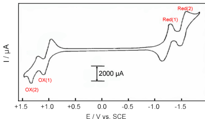
Fig. 1.3. Cyclic voltammogram of 2.5 \times 10^{-4} \text{ mol L}^{-1} octaethylporphyrin \text{H}_2\text{OEP} in 1,2\text{-CH}_2\text{Cl}_2 containing 0.1 \text{ mol L}^{-1} TBAPF 6 , scan rate : 50 \text{ mV s}^{-1} .
