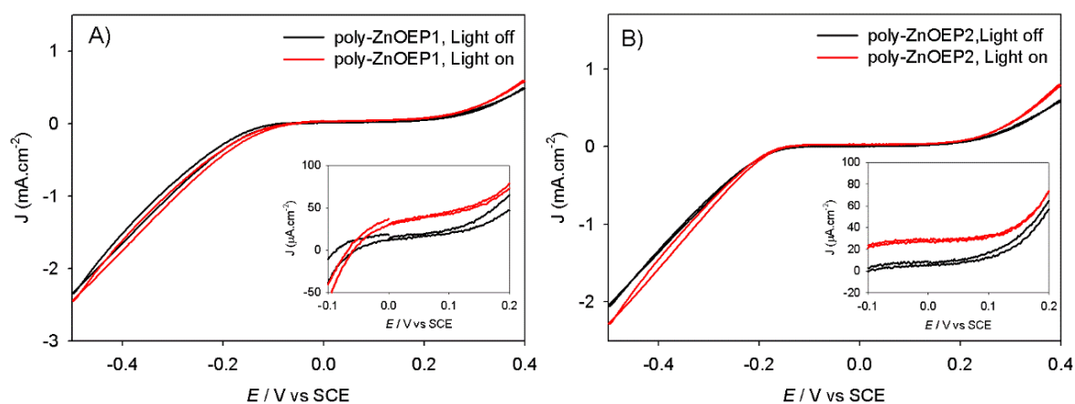
Fig. S5.8 CVs of A) poly-ZnOEP1 , B) poly-ZnOEP2 electrodes in acetonitrile containing I_2 5 mmol L^{-1} and NaI 0.5 mol L^{-1} . Inset: zoom of the cyclic voltammograms between -0.1 V and 0.2 V.
