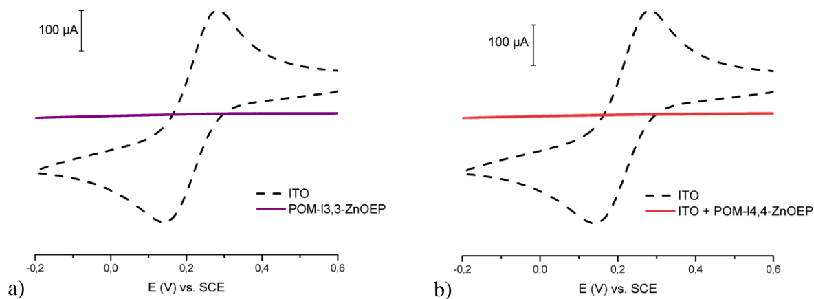
Fig. S4.12 Cyclic voltammograms of 1 \text{ mmol L}^{-1} of \text{K}_3\text{Fe}(\text{CN})_6 , in 0.5 \text{ M Na}_2\text{SO}_4 at modified ITO electrode with a) poly-POM-13,3-ZnOEP , b) poly-POM-14,4-ZnOEP films (full line) and at noncoated ITO electrode (dotted black line). \nu = 100 \text{ mV s}^{-1} . Similar behaviours have been obtained for poly-POM-s4,4-ZnOEP and poly-POM-m3,3-ZnOEP films.
