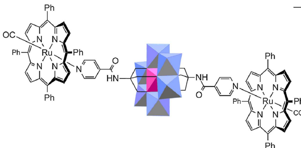
Fig. 1.31 Postulated structure of Ru(CO)TPP - dipyridyl-Anderson type POM.
