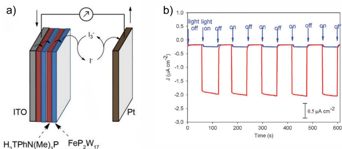
Fig. 1.25 a) Schematic illustration of the multilayer assembly [\text{H}_2\text{TPhN(Me)}_3\text{P}^{4+}/\alpha_2\text{-Fe(P}_2\text{W}_{17}\text{O}_{61})^{7-}]_n for the photocurrent generation. b) Photoelectrochemical response of [\text{H}_2\text{TPhN(Me)}_3\text{P}]^{4+} (blue curve) and [[\text{H}_2\text{TPhN(Me)}_3\text{P}^{4+}/\alpha_2\text{-Fe(P}_2\text{W}_{17}\text{O}_{61})^{7-}]_{25}] films (red curve).
