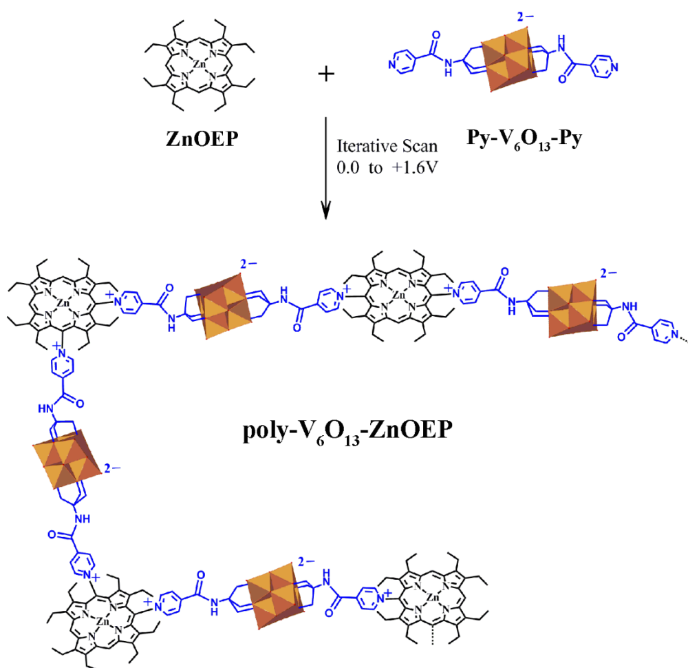
Fig. 2.2 Electropolymerization scheme of ZnOEP in the presence of [V_6O_{13}\{(OCH_2)_3CNHCO(4-C_5H_4N)\}_2]^{2-} ( Py-V 6 O 13 -Py ).
