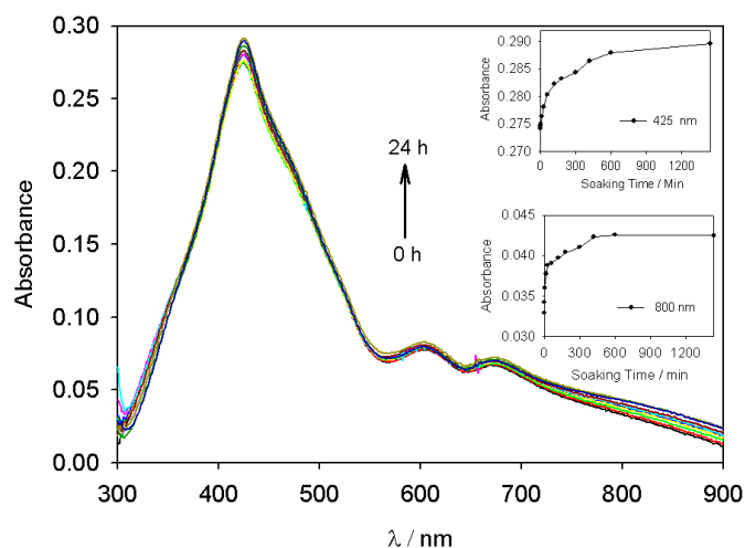
Fig. 6.8 Evolution of UV-vis spectra of the modified ITO electrode with poly- cis -H 2 Ph 2 Py 2 P-ZnOEP after soaking in P 5 W 30 @Ag aqueous solution. Inset: absorbance intensity at λ = 425 nm and λ = 800 nm vs. time.
