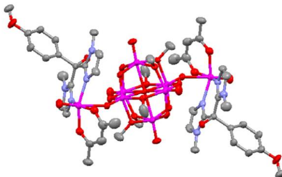
Fig. 1.27 Molecular structure of [\{VO(bmimp)(acac)\}_2\{V_6O_{13}(OCH_3)_6\}] (ORTEP dia-gram, thermal ellipsoids are represented at 50% probability; H atoms were omitted for clarity; C = grey; O = red; V = pink); N = pale blue.
