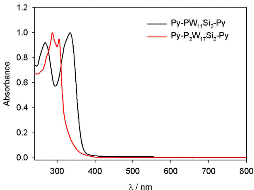
Fig. S3.1 Normalized UV-vis absorption spectra of Py-PW 11 Si 2 -Py and Py-P 2 W 17 Si 2 -Py in CH 3 CN.
