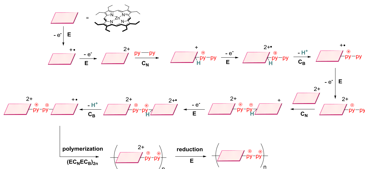
Fig. 1.49 E(\text{EC}_N\text{EC}_B)_nE mechanism proposed for the electropolymerization.
