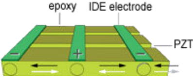
Figure 2.14. P1 type MFC actuator.
