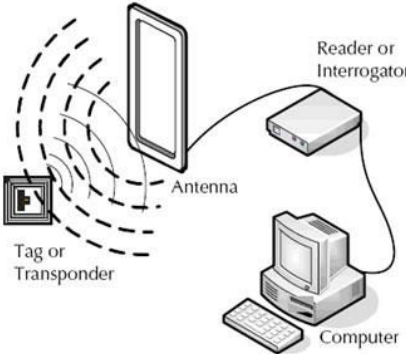
Figure 1.4. RFID system [18].
