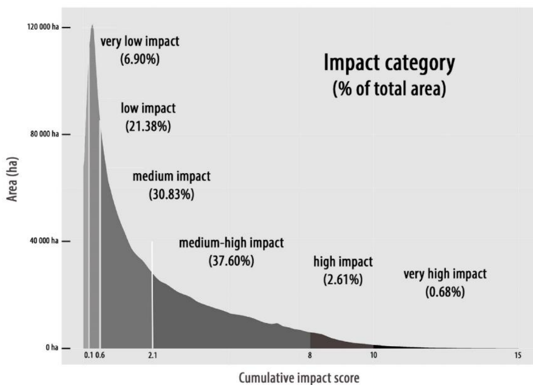
Figure 3. Cumulative impact scores ( I_c ) depicting the area (in ha) and the percent of total area (in parentheses) that falls within each impact category.
