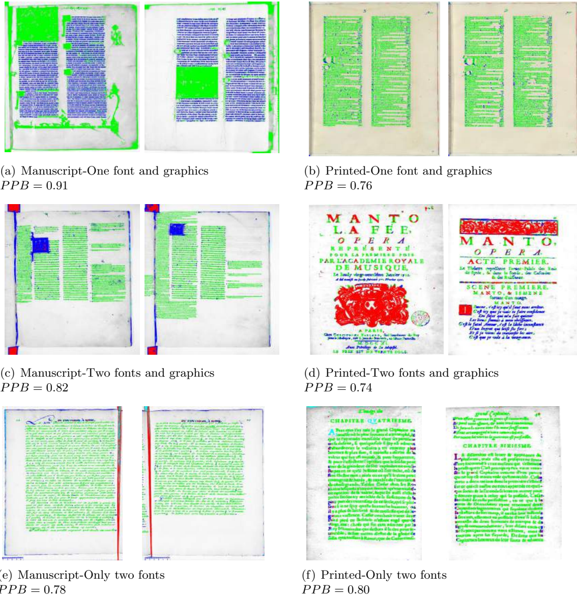
Figure 5.13.: Examples of resulting images of the proposed auto-correlation -based pixel-labeling framework for DHB content on the “DIGIDOC-Framework dataset” , performed by introducing 2000 pixels into the CCI technique and using the MD in the pixel-labeling task. For the same book, each cluster (represented by a given color) represents a similar or homogeneous region. Since the process is unsupervised, the colors attributed to text or graphics may differ from one book to another.
