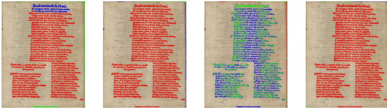
(f) Gabor J = 0.83 PPB = 0.99 F = 0.57 CA = 0.91 (g) Haar J = 0.85 PPB = 0.99 F = 0.34 CA = 0.92 (h) Db3 J = 0.47 PPB = 0.61 F = 0.44 CA = 0.56 (i) Db4 J = 0.85 PPB = 0.99 F = 0.35 CA = 0.92
