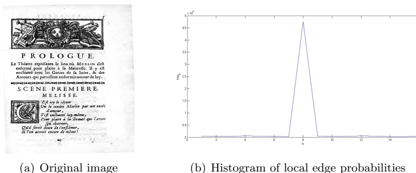
Figure B.5.: Illustration of the histogram of local edge probabilities. Figure (a) is the original image. Figure (b) represents the histogram of local edge probabilities corresponding to the original image.
