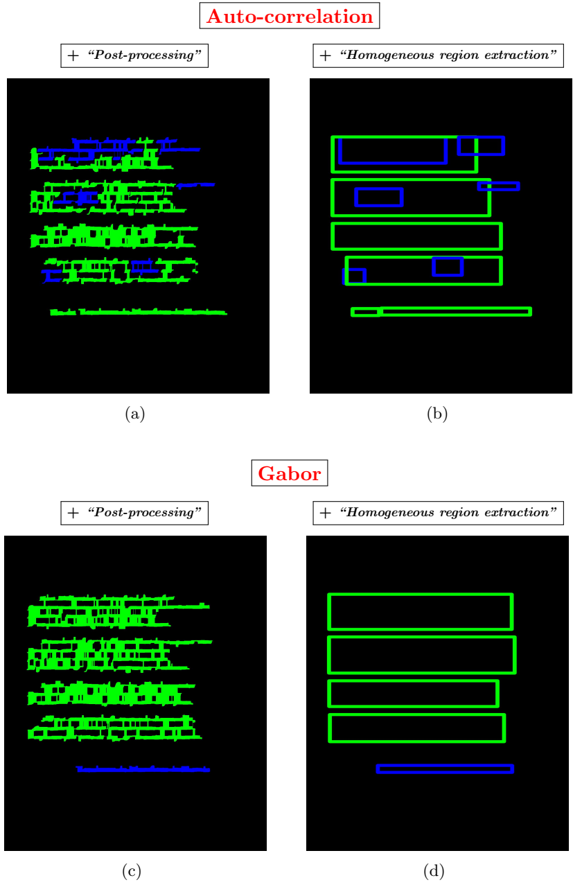
Figure B.33.: Examples of visual results of the "Homogeneous region extraction" task, performed after the "Post-processing" step on the auto-correlation and Gabor -based pixel-labeling scheme, illustrated in an "Only two fonts" HDI from the "DIGIDOC-Texture dataset" .
