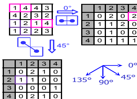
Figure B.17.: Illustration of the process of calculating the GLCM for the 0° and 45° directions.
