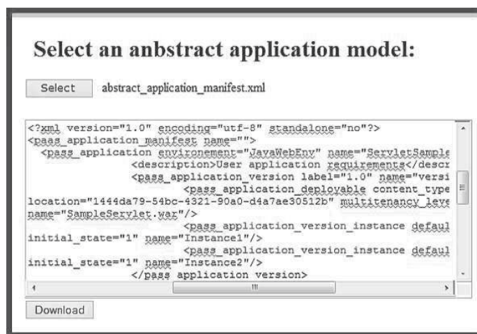
Figure 6.4: Screenshot of the interface allowing to import the abstract application manifest and generate the deployment manifest
