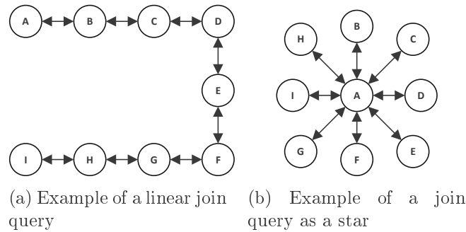
Figure 6.5: Example of a join queries
