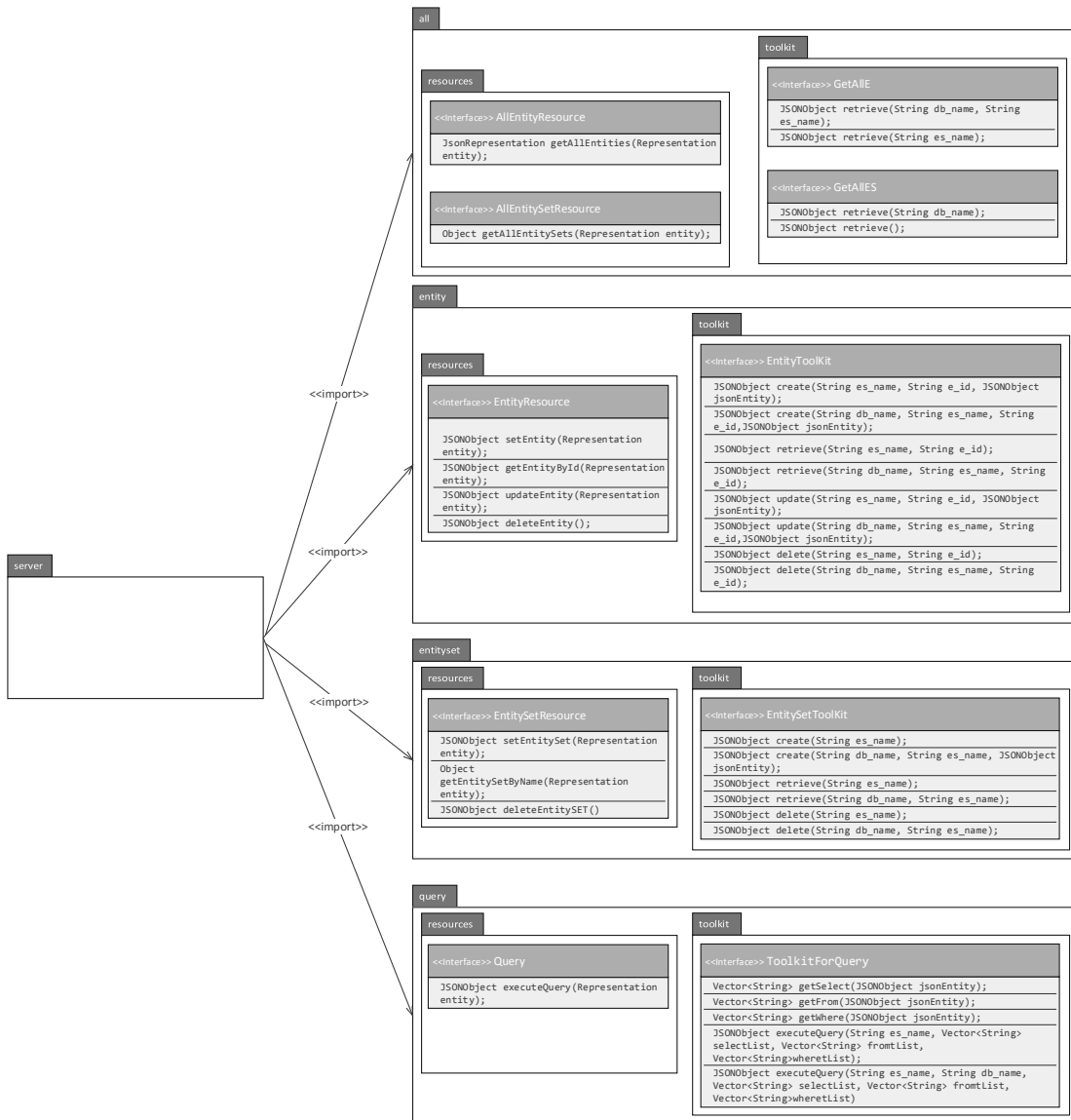
Figure 6.2: Package diagram of ODBAPI
