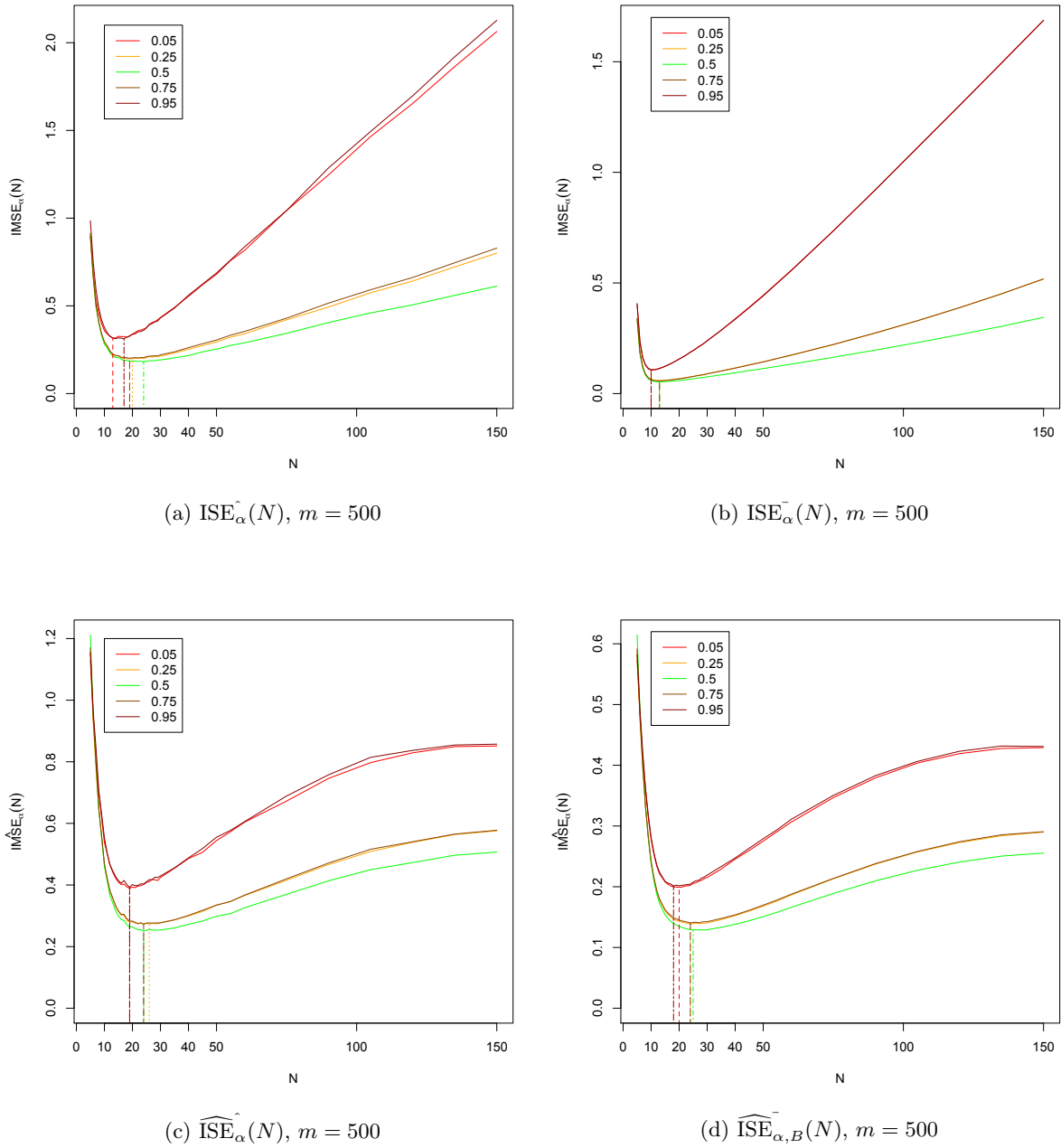
Figure 3.4 – Plots of the mappings N \mapsto \text{ISE}_{\alpha}^{\wedge}(N) (top left), N \mapsto \text{ISE}_{\alpha, B}^{-}(N) with B = 50 (top right), and of the sample mappings N \mapsto \widehat{\text{ISE}}_{\alpha}^{\wedge}(N) with \tilde{B} = 30 (bottom left), N \mapsto \widehat{\text{ISE}}_{\alpha, B}^{-}(N) with \tilde{B} = 30 and B = 50 (bottom right), averaged over 500 mutually independent replications of Model ( \mathcal{M}1 ) with sample size n = 300 .
