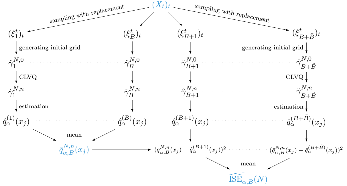
Figure 3.3 – Construction step by step of the sample ISE, \widehat{ISE}_{\alpha,B}^-(N) .
