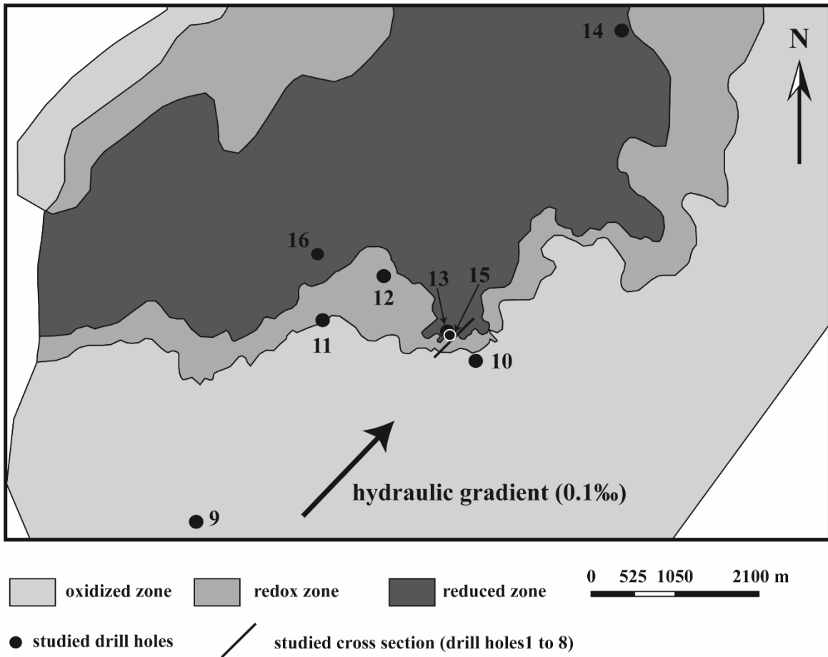
Figure 2: Location of drill holes sampled for this study on a redox map of the K 2 Ss 2 formation (Eastern Gobi Basin, Mongolia). This map was drawn taking into account the color of several hundred boreholes logged by COGEGOBI in 2012.
