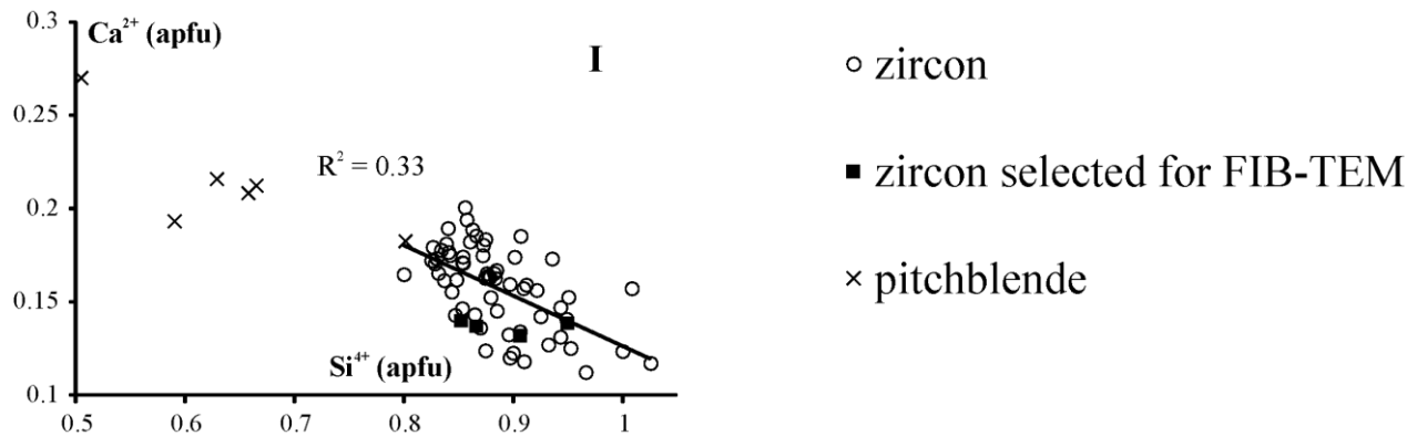
Figure 4: plot of (in apfu): (A) Zr versus Hf; (B) Zr versus Y; (C) Zr versus V; (D) Zr versus U; (E) Zr/Hf versus Hf (in element weight%); (F) U versus Ca; (G) U versus V; (H) Si versus Al; (I) Si versus Ca. The correlation is represented by the black line with the R^2 .
