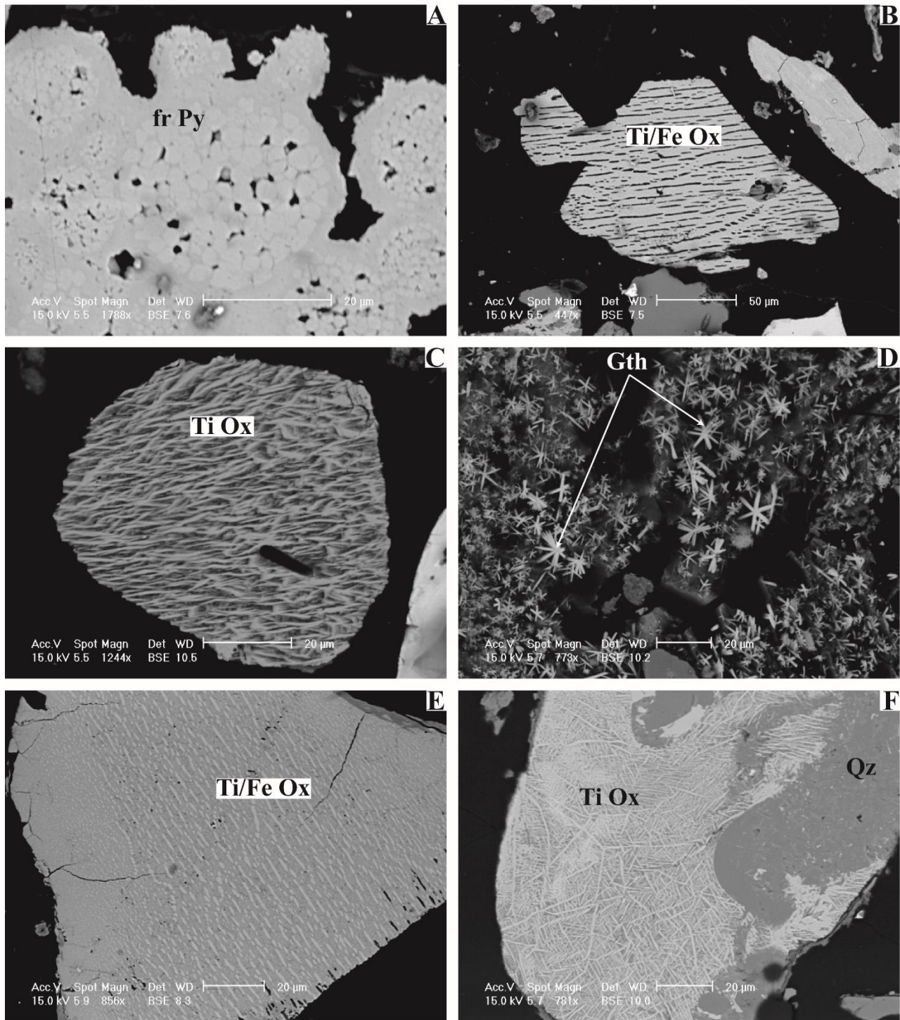
Figure 12: SEM images (BSE: backscattered electrons) of typical heavy minerals in various samples from the redox front. (A) Framboidal pyrite and pyrite cement between framboidal pyrites in the reduced zone. (B) Ti/Fe oxide in the reduced zone. (C) Ti oxide in the reduced zone. (D) Star-like goethite in clusters on phyllosilicates in the oxidized zone. (E) Ti/Fe oxide in the oxidized zone. (F) Ti oxide and quartz in the oxidized zone.
