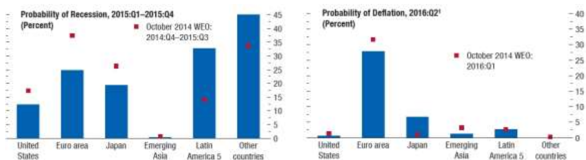
Figure 1. The probability of recession and deflation forecasts
