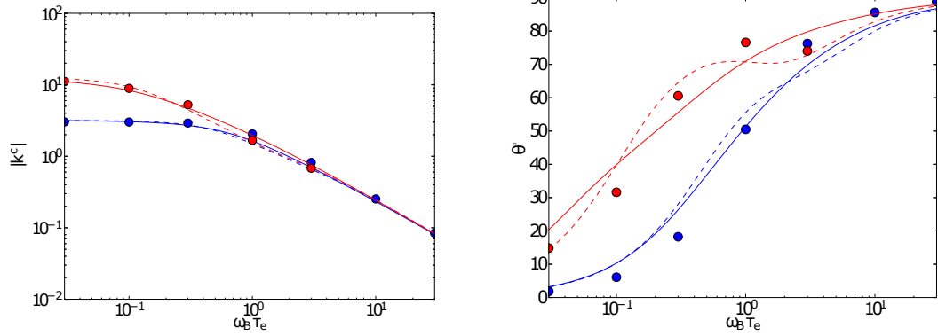
(c) Absolute value of the dimensionless thermal conductivity.
