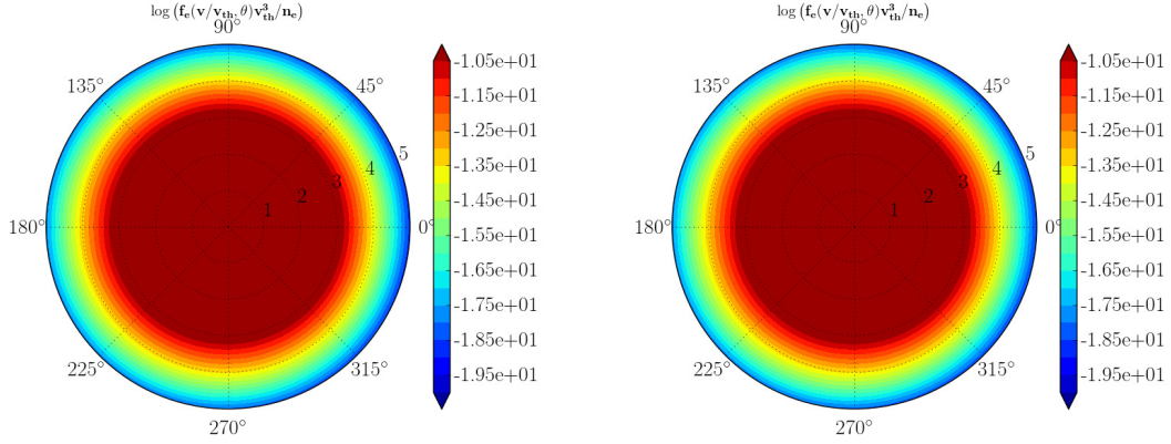
(a) P1 total EDF in the hot (right) region of plasma. (b) M1 total EDF in the hot region of plasma.
