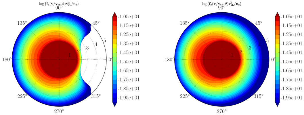
(c) P1 total EDF in the cold (left) region of plasma. (d) M1 total EDF in the cold region of plasma.
