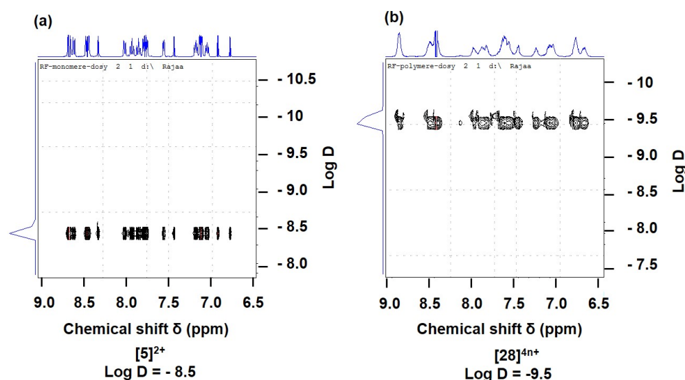
Figure 4.8: Aromatic region of the ^1\text{H} DOSY NMR spectra (a) of the metallo ligand [\text{Ru}(\phi\text{-tpy})_2]^{2+} [5] ^{2+} and (b) polymer [28] ^{4n+} in \text{CH}_3\text{CN} . The diffusion coefficients, D ( \text{m}^2\cdot\text{s}^{-1} ) are plotted in a logarithmic scale vs. the chemical shift
