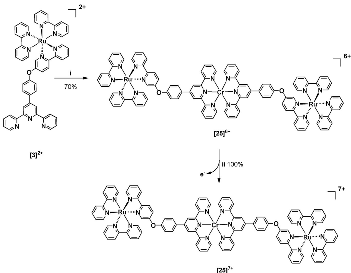
Figure 3.17: Synthesis of the trinuclear complex [\mathbf{25}]^{6+} , (i) \text{CrCl}_2 , MeOH, 65 °C, 4 h, \text{KPF}_6 ; (ii) oxidation by exhaustive electrolysis at 0 V vs. \text{Ag}/\text{AgNO}_3 ( 10^{-2} M) in \text{CH}_3\text{CN} + 0.1 M [(\text{Bu})_4\text{N}]\text{ClO}_4 .
