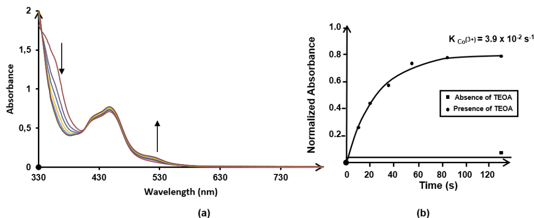
Figure 1.24: (a) Spectroscopic probing of the photoinduced reduction of [\mathbf{7}]^{7+} (b) Evolution of the absorbance of [\mathbf{7}]^{7+} at 513 nm upon continuous irradiation
