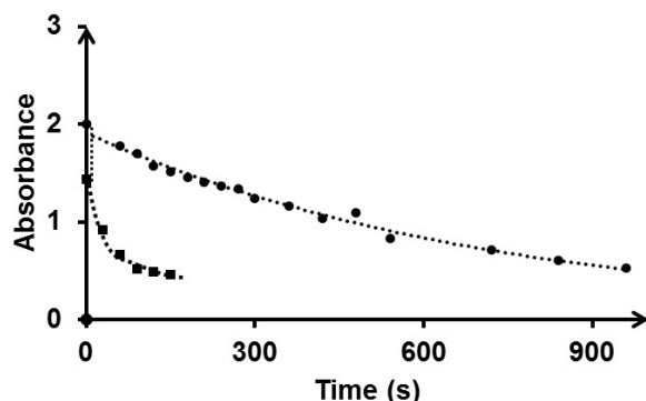
Figure 3.14: The evolution of the absorption at 370 nm under similar experimental conditions for a mixture of [\text{Cr}(\text{tpy})_2]^{3+}/\text{PPh}_3 (●) and a mixture of [\text{Ru}(\text{bpy})_3]^{2+}/[\text{Cr}(\text{tpp})_2]^{3+}/\text{PPh}_3 (■).
