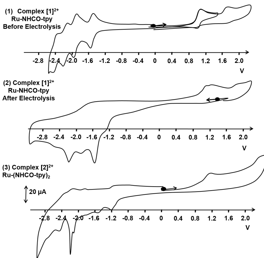
Figure 1.9: CV of modified ruthenium complexes in a 10^{-3} M solution \text{CH}_3\text{CN} + 0.1 M [\text{N}(\text{Bu})_4]\text{PF}_6 using a glassy carbon electrode(5mm) at a scan rate 100 mV/s recorded vs. \text{Ag}/\text{AgNO}_3 ( 10^{-2} M); (1) \text{Ru-NHCO-tpy} before electrolysis; (2) \text{Ru-NHCO-tpy} after electrolysis carried out at 1.4 V; (3) \text{Ru-(NHCO-tpy)}_2
