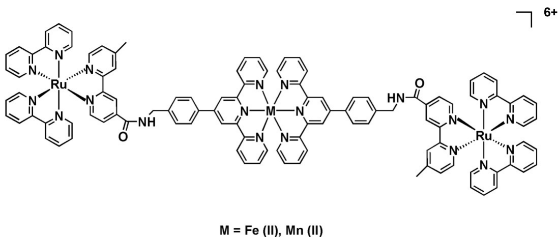
Figure 1.3: Hetero-tri-nuclear complexes based on amide bridges
