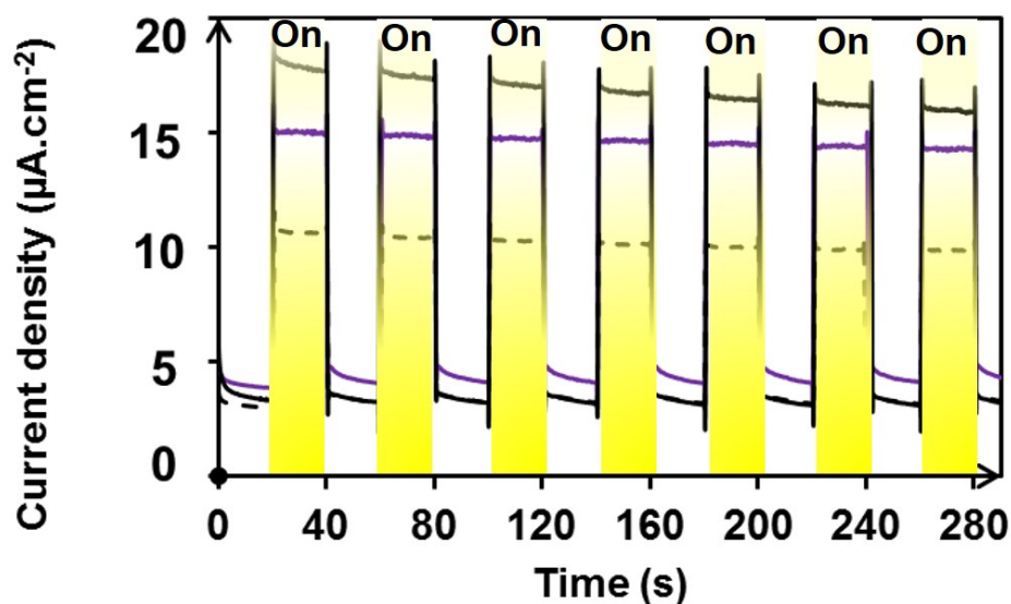
Figure 2.29: Photocurrent density ( \mu\text{A}\cdot\text{cm}^{-2} ) vs. time. Irradiation periods are highlighted in yellow ITO/ [\text{Co}(\text{tpy})_2]\text{O}[\text{Ru}(\text{bpy})_3] dashed line; ITO/ [\text{Co}(\text{tpy})_2]\text{O}[\text{Ru}(\text{bpy})_3]\text{O}[\text{Fe}(\text{tpy})_2] full black line; ITO/ [\text{Zn}(\text{tpy})_2]\text{O}[\text{Ru}(\text{bpy})_3]\text{O}[\text{Fe}(\text{tpy})_2] full purple line
