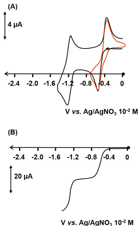
Figure 3.23: (A) black: CV of [27] in \text{CH}_3\text{CN} + 0.1 \text{ M } [\text{Bu}_4\text{N}]\text{ClO}_4 at a carbon electrode of 1 mM solution; scan rate: 100 \text{ mV}\cdot\text{s}^{-1} ; Red: second scan (B) Voltammogram at a carbon RDE of a solution of [27] in \text{CH}_3\text{CN} + 0.1 \text{ M } [\text{Bu}_4\text{N}]\text{ClO}_4 , \omega = 600 \text{ rpm} , scan rate: 5 \text{ mV}\cdot\text{s}^{-1}
