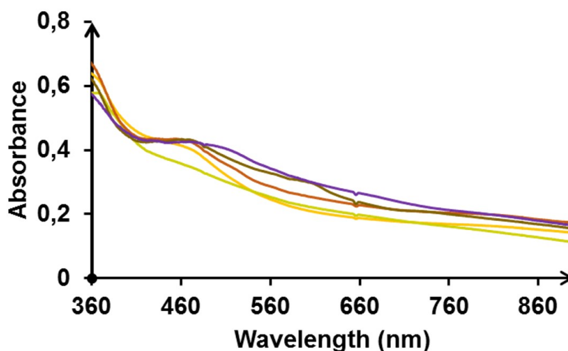
Figure 4.23: Absorption spectra of ITO coated with [\mathbf{29}]^{5n+} in \text{CH}_3\text{CN} : Purple: applied potential = -1.1 V; brown: applied potential = -0.9 V; Red: applied potential = -0.5 V, Orange: applied potential = 0 V; Green: applied potential = 1.2 V
