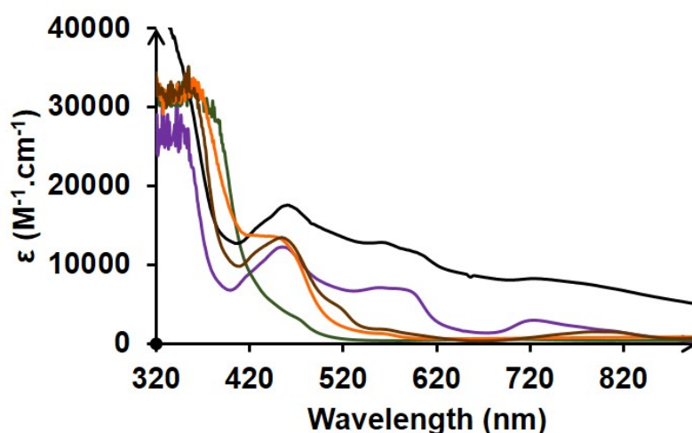
Figure 4.20: Absorption spectra of the different oxidation states of complex [29]^{xn+} in \text{CH}_3\text{CN} + 0.1 \text{ M} [\text{Bu}_4\text{N}]\text{BF}_4 , black line represents [29]^{2n+} , purple line represents [29]^{3n+} ; brown line represents [29]^{4n+} ; red line represents [29]^{5n+} ; green line represents [29]^{6n+} .
