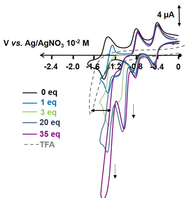
Figure 3.21: CV of [\mathbf{24}]^{2+} in \text{CH}_3\text{CN} + 0.1 \text{ M } [\text{Bu}_4\text{N}]\text{BF}_4 at a carbon electrode of 1 \text{ mM} solution; scan rate: 100 \text{ mV}\cdot\text{s}^{-1} upon addition of 1, 3, 20, 35 equivalent of TFA ; Dashed grey line represents the CV of a solution of 55 equivalence of TFA in \text{CH}_3\text{CN} + 0.1 \text{ M } [\text{Bu}_4\text{N}]\text{BF}_4 .
