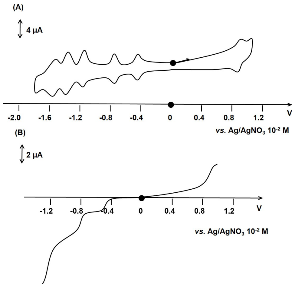
Figure 4.19: (A) CV of [29]^{5n+} ( 10^{-5} M) in \text{CH}_3\text{CN} + 0.1 M [\text{Bu}_4\text{N}]\text{ClO}_4 at a carbon electrode of 0.5 mM solution; scan rate: 100 \text{ mV}\cdot\text{s}^{-1} ; (B) Voltammogram at a carbon RDE in \text{CH}_3\text{CN} + 0.1 M [\text{Bu}_4\text{N}]\text{BF}_4 , \omega = 600 \text{ rpm} , scan rate: 5 \text{ mV}\cdot\text{s}^{-1} .
