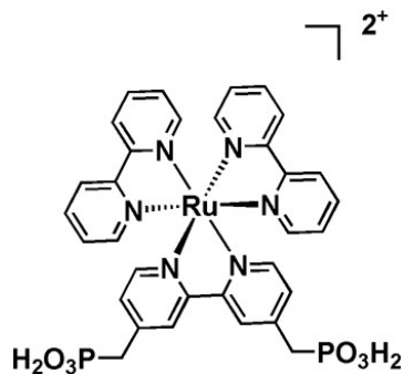
Figure 13: Functionalized [\text{Ru}(\text{bpy})_3]^{2+} precursor used to graft onto nanostructured ITO.
