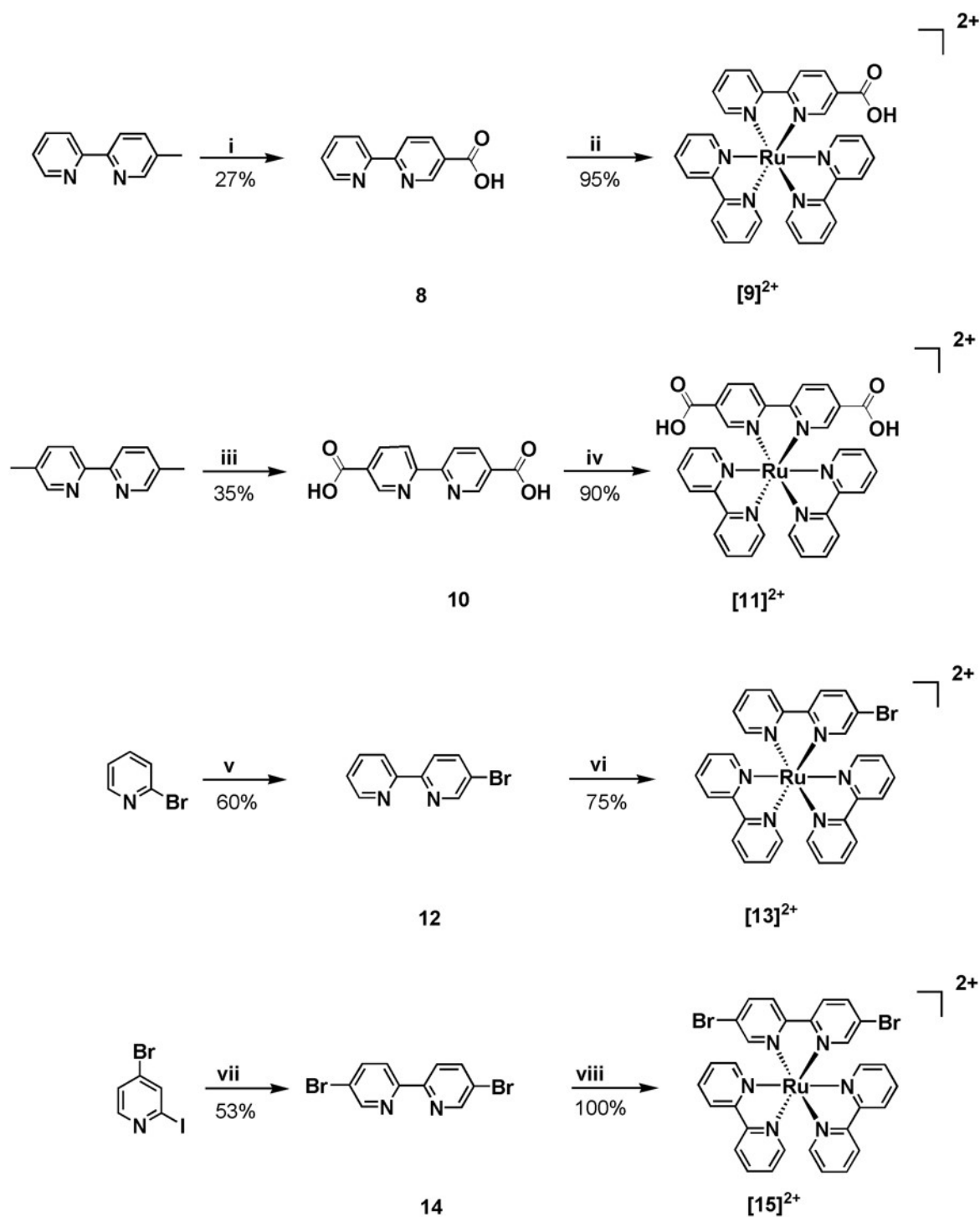
Figure 1.6: Functionalization of the [\text{Ru}(\text{bpy})_3]^{2+} , (i) \text{KMnO}_4 , \text{H}_2\text{O} , 48 h, 100^\circ\text{C} , \text{HCl} ; (ii) [\text{Ru}(\text{bpy})_2(\text{Cl})_2] , ethylene glycol, 2 h, 120^\circ\text{C} , \text{NH}_4\text{PF}_6 ; (iii) \text{KMnO}_4 , \text{H}_2\text{O} , 48 h, 100^\circ\text{C} , \text{HCl} ; (iv) [\text{Ru}(\text{bpy})_2(\text{Cl})_2] , ethylene glycol, 2 h, 120^\circ\text{C} , \text{NH}_4\text{PF}_6 ; (v) n\text{BuLi} , diethylether, 2 h, -78^\circ\text{C} / \text{Me}_3\text{SnCl} , 10 h, 25^\circ\text{C} /4-bromo-2-iodopyridine, [\text{Pd}(\text{PP}_3)_4] , toluene, 24 h, 120^\circ\text{C} ; (vi) [\text{Ru}(\text{bpy})_2(\text{Cl})_2] , ethylene glycol, 2 h, 120^\circ\text{C} , \text{KPF}_6 ; (vii) (\text{Sn}(\text{Bu})_3)_2 , [\text{Pd}(\text{PPh}_3)_4] , toluene, 24 h, 120^\circ\text{C} ; (viii) [\text{Ru}(\text{bpy})_2(\text{Cl})_2] , ethylene glycol, 2 h, 120^\circ\text{C} , \text{KPF}_6
