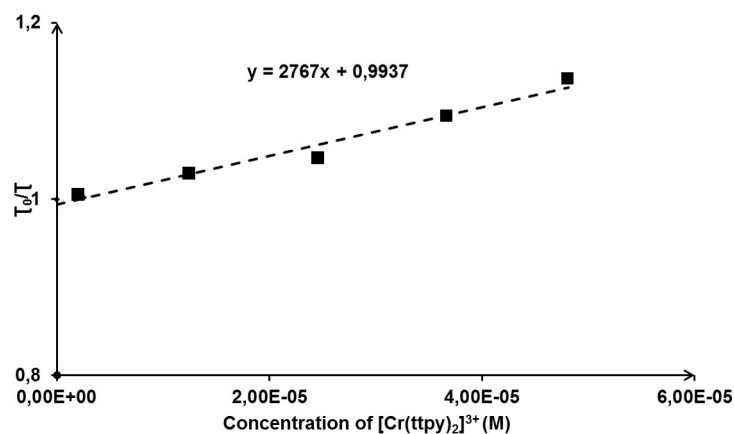
Figure 3.16: A Stern-Volmer plot of the quenching of [\text{Ru}(\text{bpy})_3]^{2+} upon addition of increasing concentration of [\text{Cr}(\text{tppy})_2]^{3+} in deoxygenated \text{CH}_3\text{CN}
