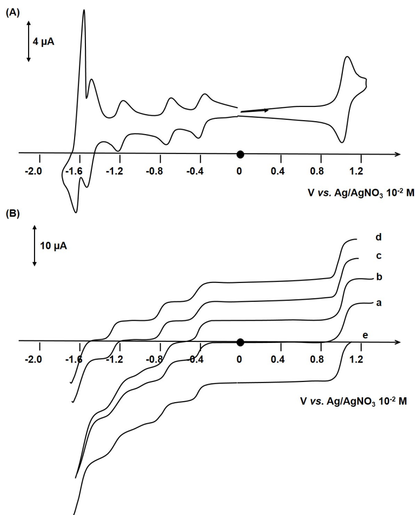
Figure 3.18: (A) CV of [25]^{7+} ( 10^{-3} M) in \text{CH}_3\text{CN} + 0.1 M [\text{Bu}_4\text{N}]\text{ClO}_4 at a carbon electrode; scan rate: 100 \text{ mV}\cdot\text{s}^{-1} ; (B) Voltammogram at a carbon RDE of the same solution, \omega = 600 rpm, scan rate: 5 \text{ mV}\cdot\text{s}^{-1} : (a) [25]^{7+} initial solution, (b) after electrolysis at -0.7 V forming [25]^{6+} , (c) after electrolysis at -1.0 V forming [25]^{5+} , (d) after electrolysis at -1.3 V forming [25]^{4+} , (e) after electrolysis at 1.2 V forming [25]^{9+}
