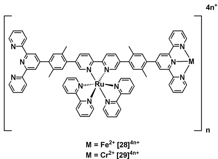
Figure 4.6: One-dimensional bimetallic polymer based on [\text{Ru}(\text{bpy})_3]^{2+} and terpyridyl complex of either \text{Fe}^{2+} or \text{Cr}^{2+}
