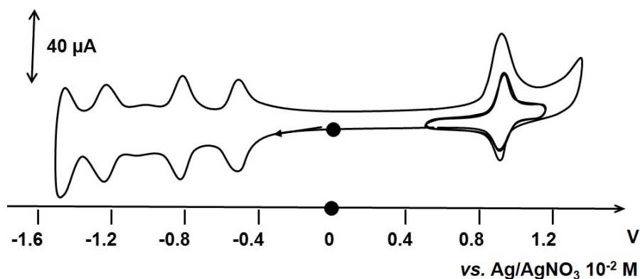
Figure 4.22: CV of the ITO surface coated with [\mathbf{29}]^{5n+} in a \text{CH}_3\text{CN} solution containing 0.1 \text{ M} [\text{Bu}_4\text{N}]\text{ClO}_4 at v = 50 \text{ mV}\cdot\text{s}^{-1} .
