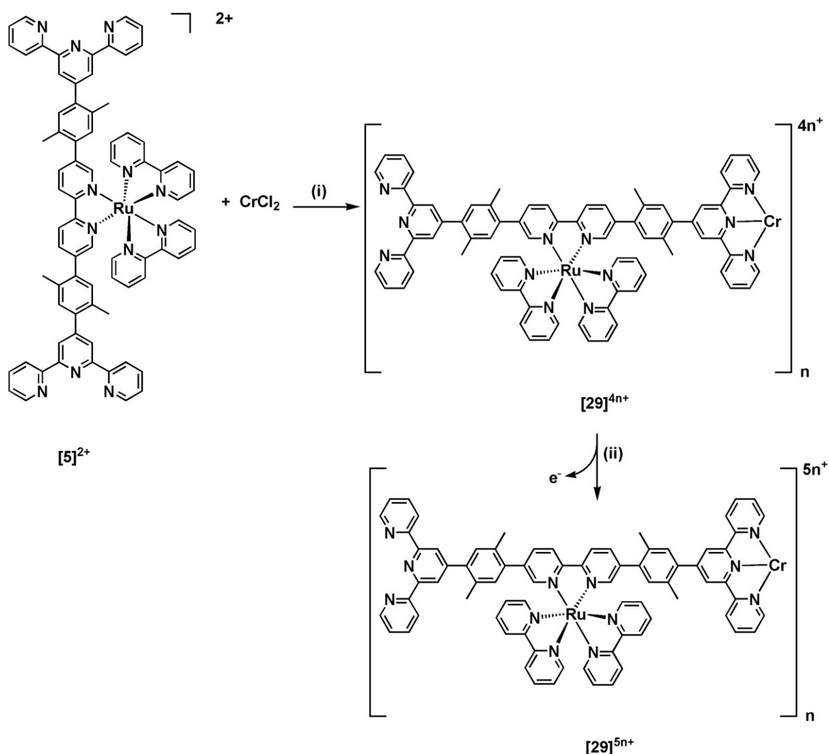
Figure 4.18: Synthesis of the chromium-ruthenium bimetallic polymer [\mathbf{29}]^{4n+} , (i) \text{CrCl}_2 , MeOH, 65^\circ\text{C} , 4 h, \text{NH}_4\text{PF}_6 ; (ii) oxidation by exhaustive electrolysis at 0 V vs. \text{Ag}/\text{AgNO}_3 in \text{CH}_3\text{CN} + 0.1\text{ M } [\text{Bu}_4\text{N}]\text{ClO}_4 to yield [\mathbf{29}]^{5n+} .
