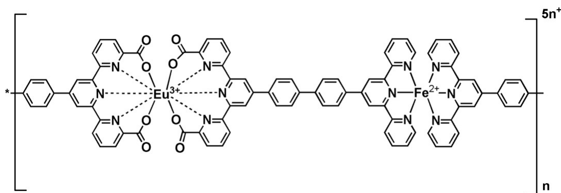
Figure 4.1: Alternating \text{Eu}^{3+} and \text{Fe}^{2+} terpyridyl polymer
