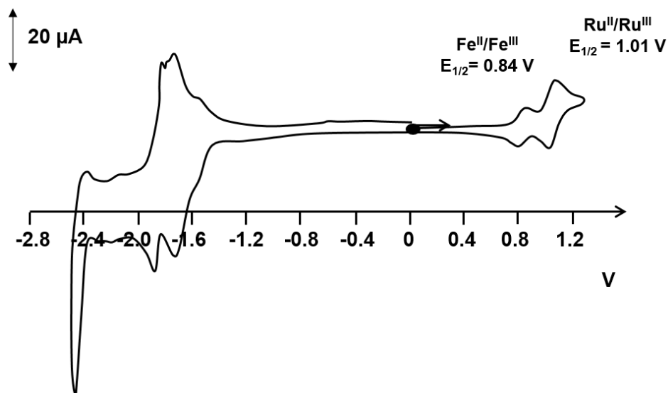
Figure 1.14: CV of [\mathbf{6}]^{6+} ( 10^{-3} M) in a solution of \text{CH}_3\text{CN} + 0.1 M [\text{Bu}_4\text{N}]\text{PF}_6 , and the E_{1/2} values are reported vs \text{Ag}/\text{AgNO}_3 ( 10^{-2} M) at scan rate = 100 mV/s using carbon vitreous disk (5 mm in diameter) as a working electrode
