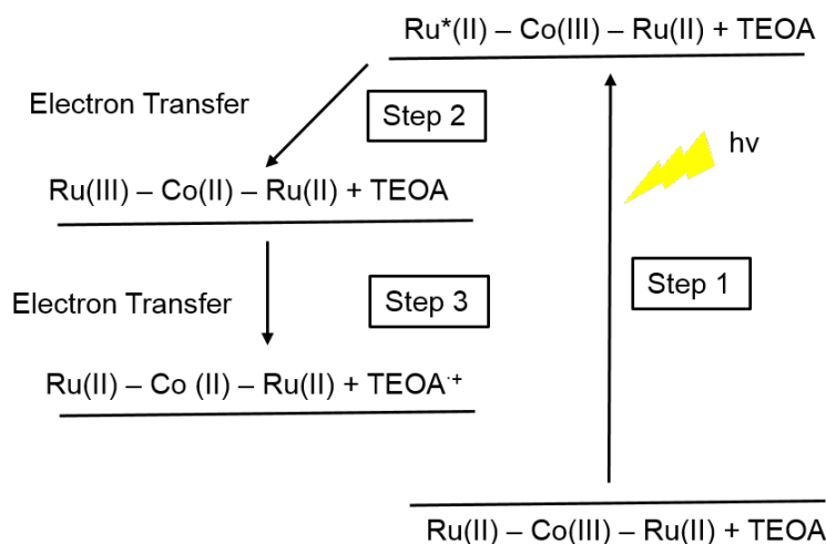
Figure 1.25: Proposed mechanism for the electron transfer in [\mathbf{7}]^{7+}
