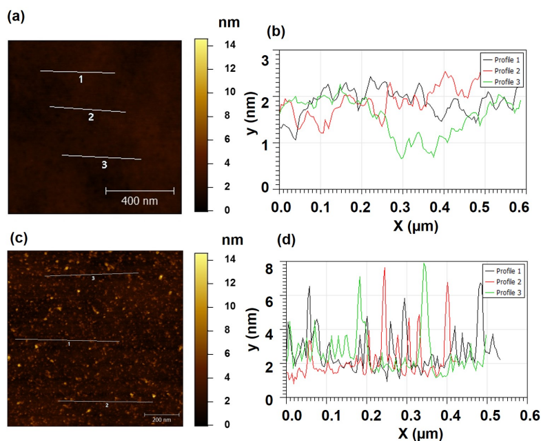
Figure 2.28: (a) AFM topography of a 1 \mu\text{m}^2 naked silicon oxide, (b) Profile of naked ITO, (c) AFM of a of a 1 \mu\text{m}^2 \text{SiO}_2 /[Co(tpy) 2 ] \phi [Ru(bpy) 3 ] \phi [Fe(tpy) 2 ], (d) Profile of \text{SiO}_2 /[Co(tpy) 2 ] \phi [Ru(bpy) 3 ] \phi [Fe(tpy) 2 ]
