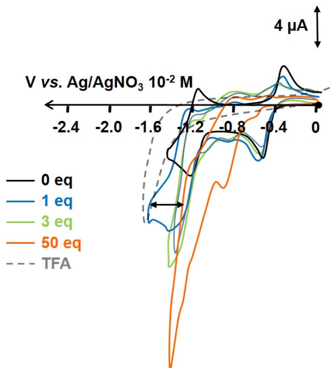
Figure 3.24: CV of [27] in \text{CH}_3\text{CN} + 0.1 \text{ M } [\text{Bu}_4\text{N}]\text{ClO}_4 at a carbon electrode of 1 mM solution; scan rate: 100 \text{ mV}\cdot\text{s}^{-1} upon addition of 1, 3, 50 equivalent of TFA ; Dashed grey line represents the CV of a solution of 55 equivalence of TFA in \text{CH}_3\text{CN} + 0.1 \text{ M } [\text{Bu}_4\text{N}]\text{ClO}_4
