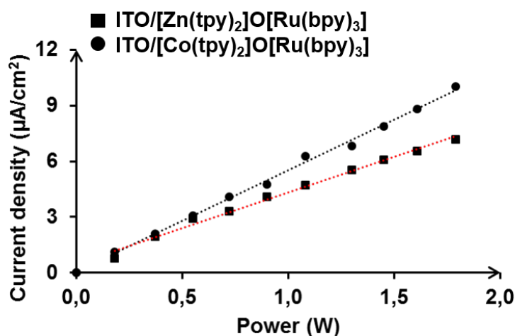
Figure 2.18: The variation of the magnitude of the photocurrent for ITO/[Zn(tpy) 2 ]O[Ru(bpy) 3 ] and ITO/[Co(tpy) 2 ]O[Ru(bpy) 3 ] with changing the power of irradiation
