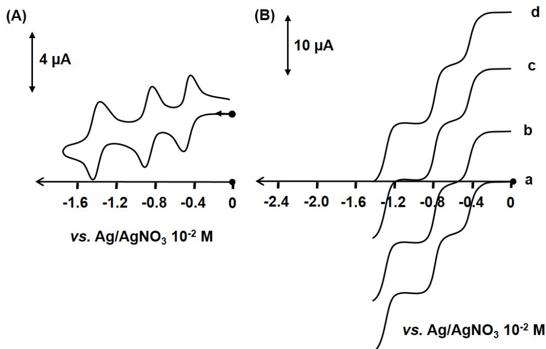
Figure 3.5: (A) CV of [\mathbf{24}]^{3+} ( 10^{-3} M) in \text{CH}_3\text{CN} + 0.1 M [\text{Bu}_4\text{N}]\text{BF}_4 at a carbon electrode (5 mm diameter); scan rate: 100 \text{ mV}\cdot\text{s}^{-1} vs. \text{Ag}/\text{AgNO}_3 ( 10^{-2} M); (B) Voltammogram at a carbon RDE of the same solution, \omega = 600 rpm, scan rate: 5 \text{ mV}\cdot\text{s}^{-1} : (a) [\mathbf{24}]^{3+} , (b) [\mathbf{24}]^{2+} , (c) [\mathbf{24}]^+ , (d) [\mathbf{24}]^0
