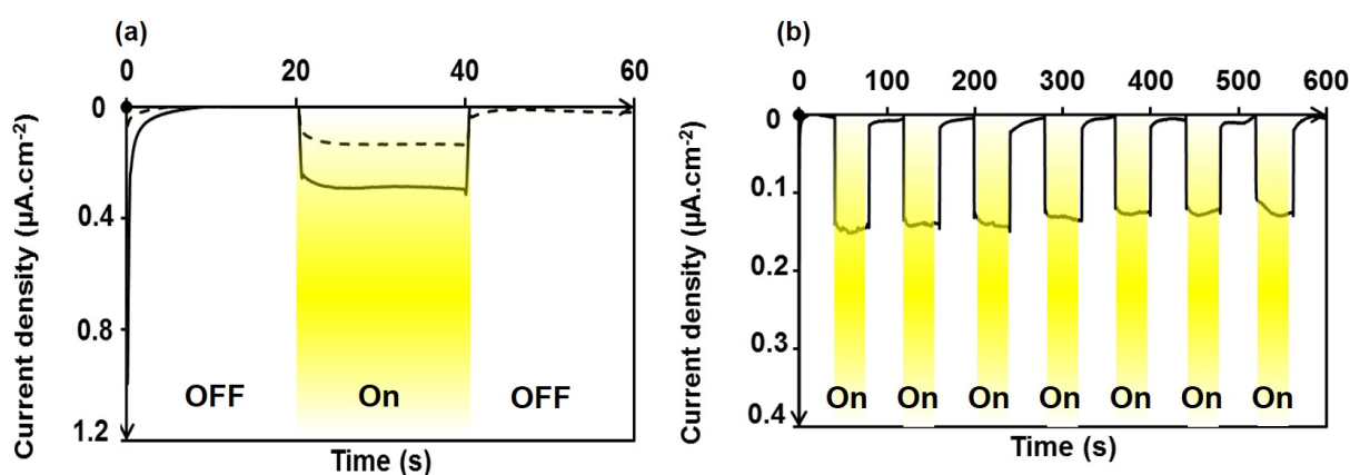
Figure 2.22: Photocurrent density ( \mu \text{ A}\cdot\text{cm}^{-2} ) vs. time. Irradiation periods are highlighted in yellow (a) ITO/[Fe(tpy) 2 ]O[Ru(bpy) 3 ] full line and ITO/[Zn(tpy) 2 ]O[Ru(bpy) 3 ] dotted line; (b) Several on off cycles for ITO/[Fe(tpy) 2 ]O[Ru(bpy) 3 ]
