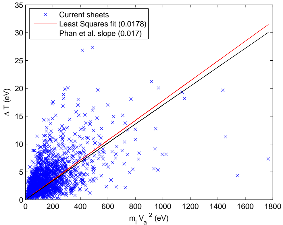
FIGURE 5.21: Scatter plot of electron heating and the available magnetic energy defined as m_i V_a^2 . The red line represents a least squares fit of this data. It yields a slope of 0.0178, with a correlation coefficient of 0.5419. The black line is the slope of 0.017 produced by [114].
