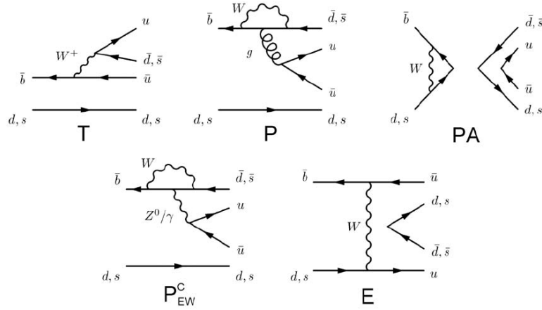
Figure 2.7 – Diagrams contributing to the amplitudes of charmless B^0_{(s)} decays. The topologies involved are: Tree ( T ), Penguin ( P ), Penguin Annihilation ( PA ), Colour-suppressed Electroweak Penguin ( P_{EW}^C ) and Exchange ( E ) [65].
