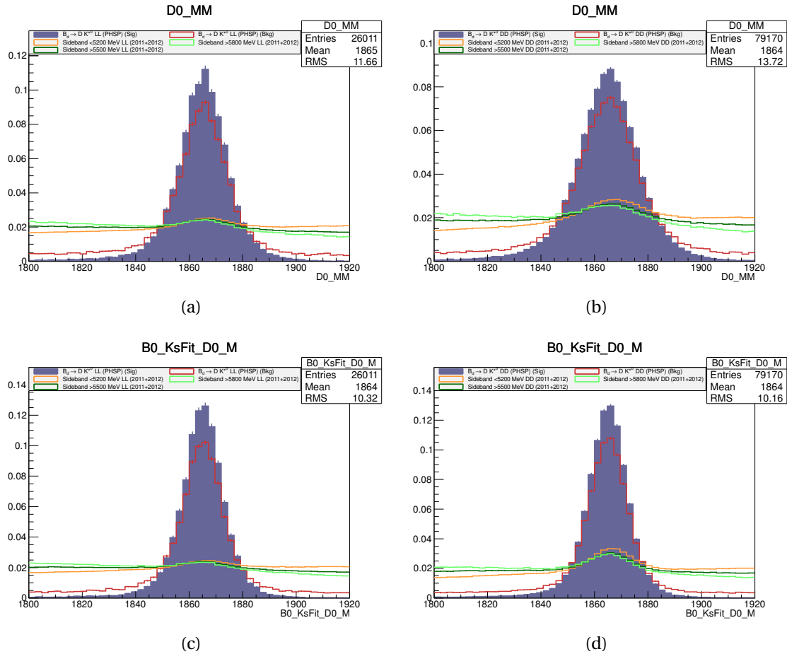
Figure 5.2 – D^0 invariant mass distributions without constraint on LL (a) and DD (b) candidates, and constraining the K^0_S mass and the B^0 flight direction of LL (c) and DD (d) candidates. The blue distributions correspond to the MC B^0 \rightarrow DK^{*0} truth matched signal ( i.e. candidates with correct true ID and correct daughters and mother), the red distributions to the signal failing the truth-matching, the orange distributions to the m_{B^0} < 5.2\text{GeV} data sideband and the (dark) green distributions to the m_{B^0} > 5.8\text{GeV} ( > 5.5\text{GeV} ) data sideband.
