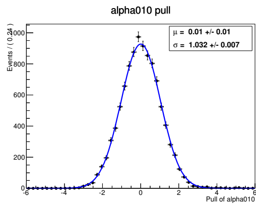
Figure 5.57 – Pull distribution of the helicity component proportion in the B_{(s)}^0 \rightarrow D^{*0}K^{*0} partially reconstructed background ( \alpha_{010} parameter).
